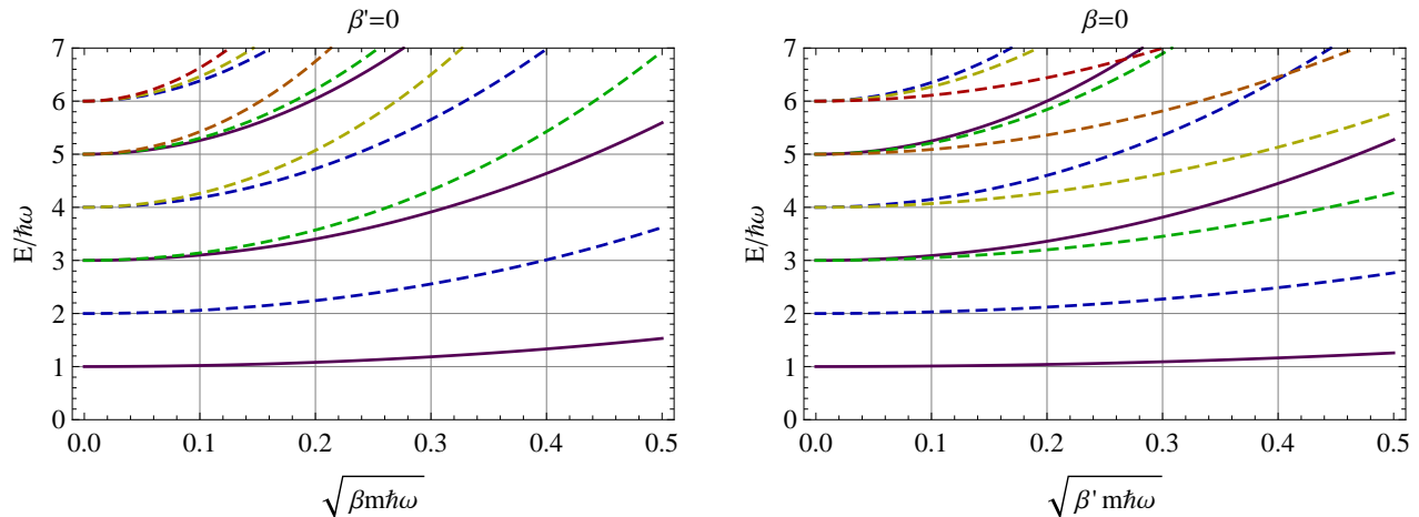
FIG. 2: The energy levels of the 2D isotropic harmonic oscillator for the cases \beta' = 0 (left) and \beta = 0 (right). The purple solid lines indicate s -wave states which are singlets. The dashed lines are doublets with the color indicating \ell = 1 (blue), \ell = 2 (green), \ell = 3 (yellow), \ell = 4 (orange), and \ell = 5 (red). \sqrt{\beta m \hbar \omega} is the ratio of the minimal length \hbar \sqrt{\beta} to the characteristic length scale \sqrt{\hbar/m\omega} of the system.
