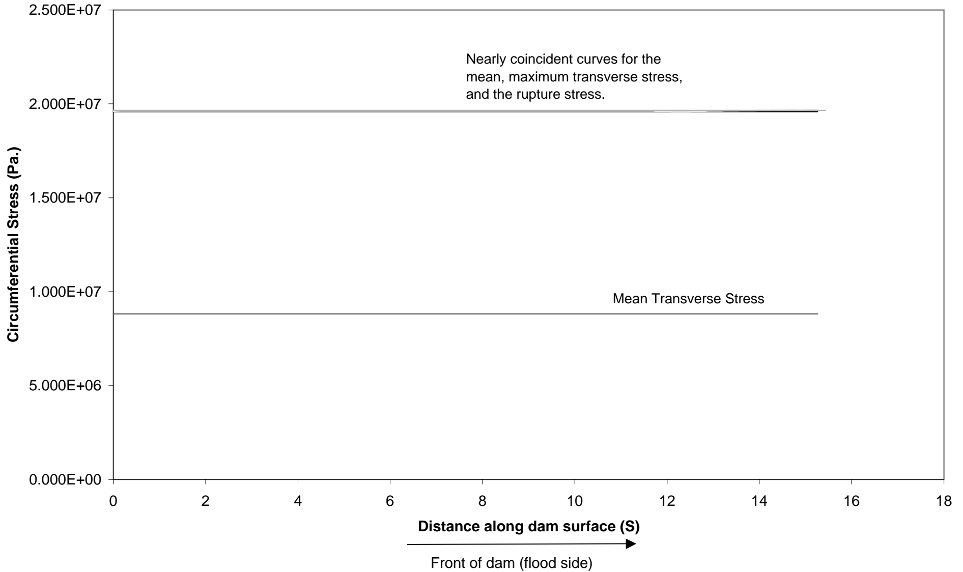
Figure I-12: Plot of the static stresses in the dam for an inflation pressure which would cause the dam to rupture.
