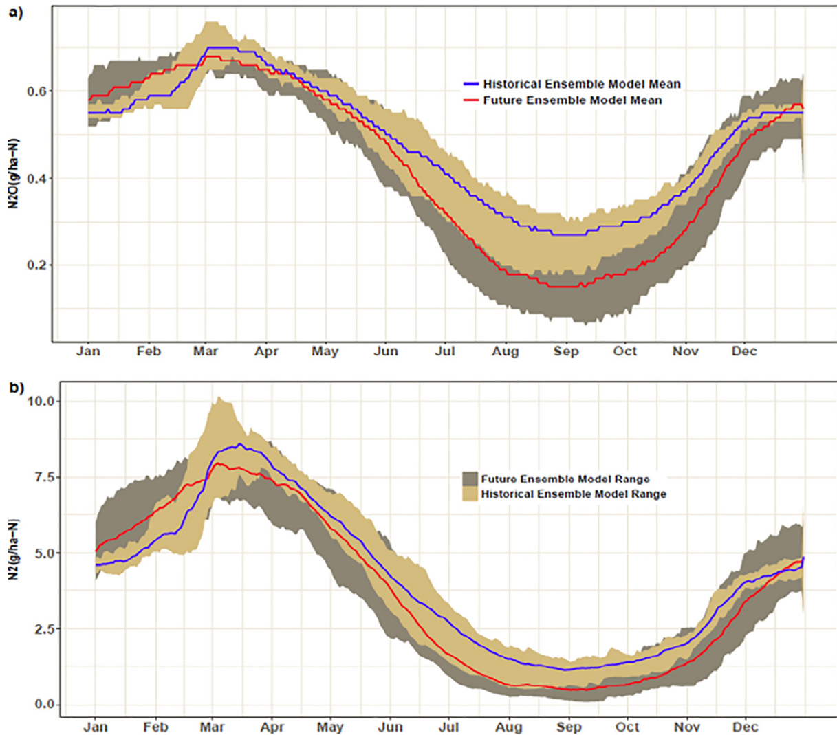
Fig. 5. Model predicted average-by-day N 2 O (a) and N 2 (b) emission rates for the seven climate models for the 24-year future time period and the historical period.
