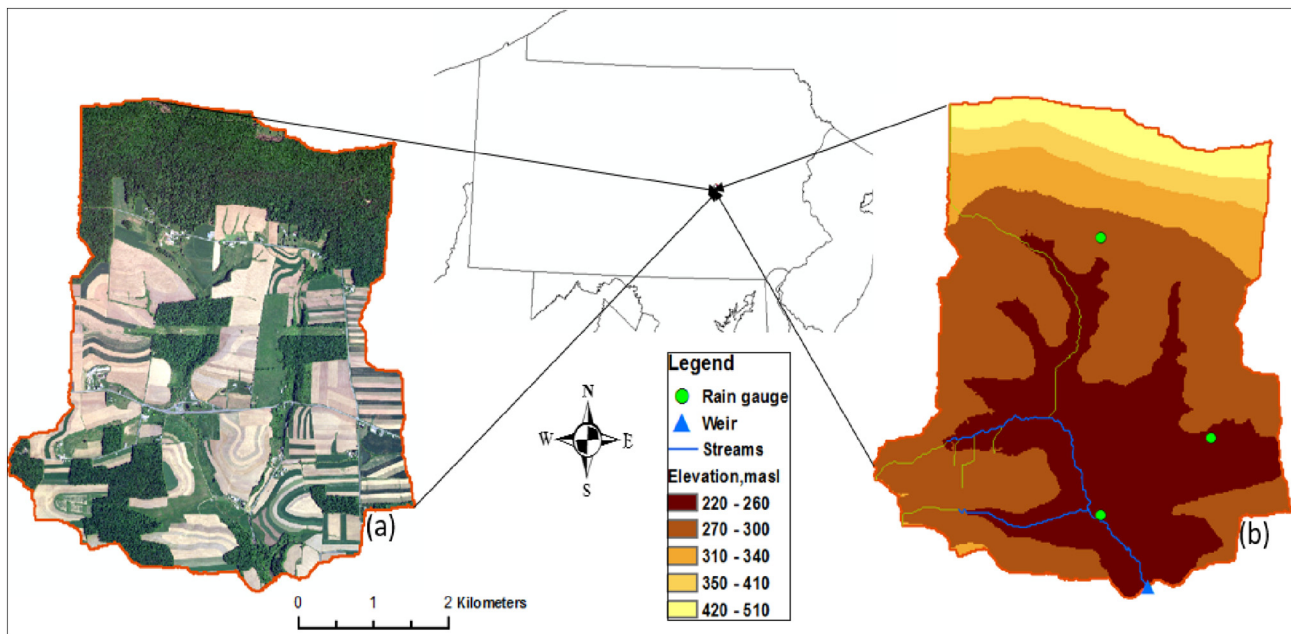
Fig. 1. Location of WE-38 watershed in Pennsylvania, USA, and land cover ortho-imagery for 2015 (a) and digital elevation model (b) showing the location of the weir location and precipitation gauges.
