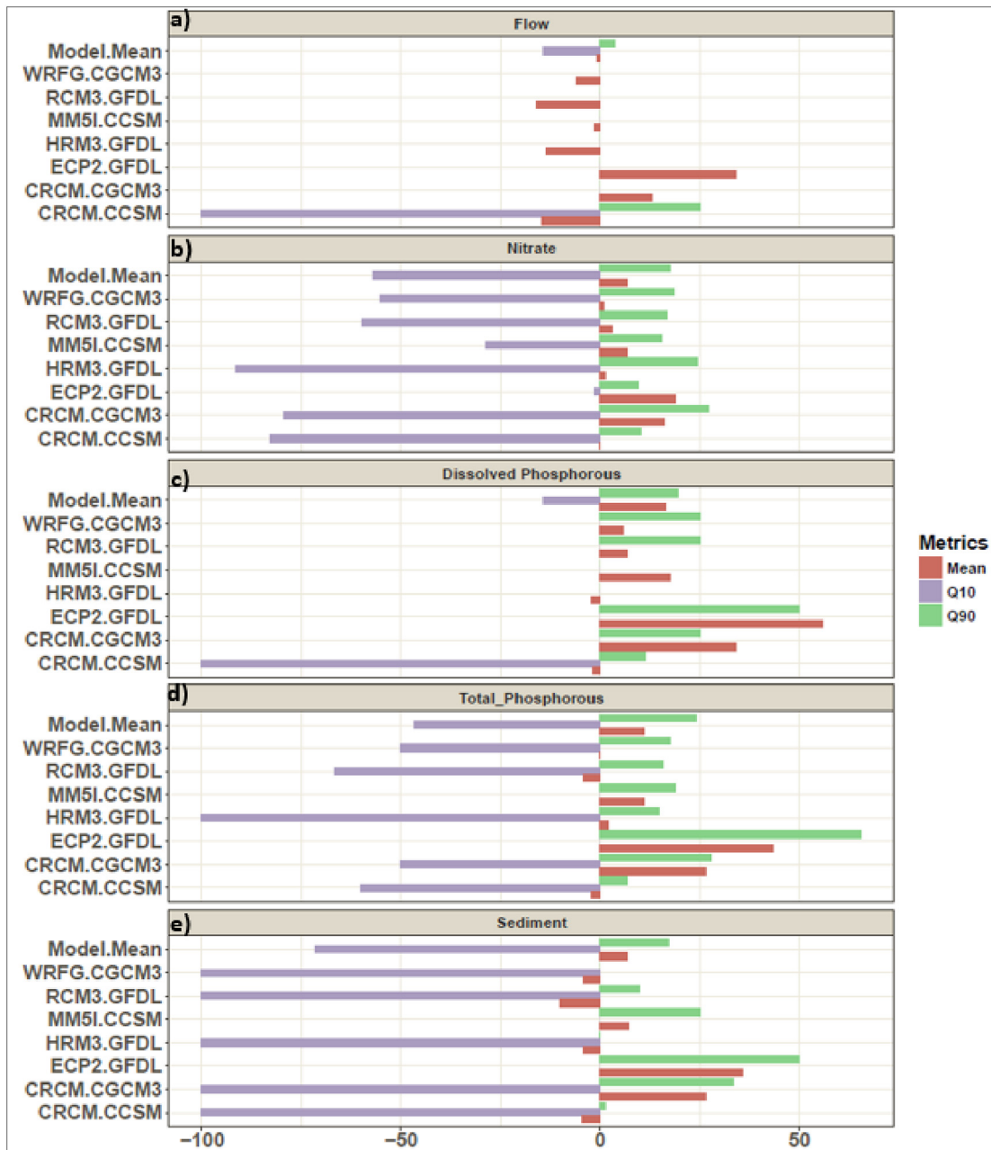
Fig. 2. Percent change in the mean watershed outlet, Q 10 , and Q 90 for daily flow (a), nitrate (b), dissolved P (c), total P (d), and sediment (e) export for seven climate models relative to the historical scenario (1975–1998) for the future time period (2045–2068).
