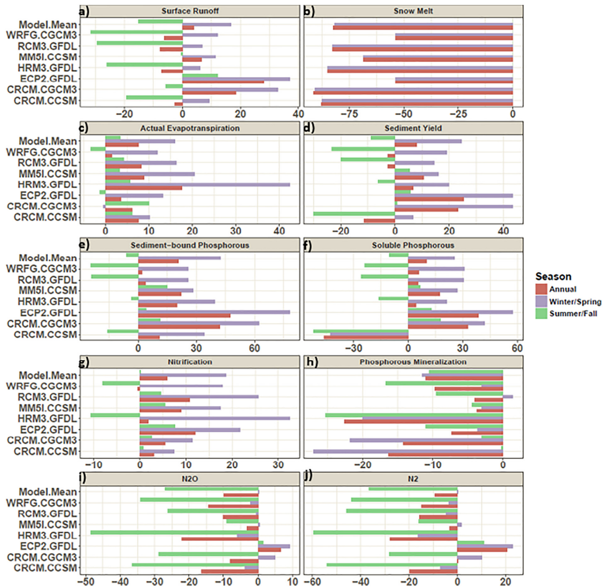
Fig. 4. Annual and seasonal changes (%) for surface runoff (a), snowmelt (b), actual evapotranspiration (c), sediment yield (d), sediment-bound P export (e), dissolved P export (f), nitrification rate (g), phosphorus mineralization rate (h), N_2O emission rate (i), and N_2 (j) emission rate averaged across agricultural HRUs for seven climate models relative to historical scenario (1975–1998) for the future time period (2045–2068).
