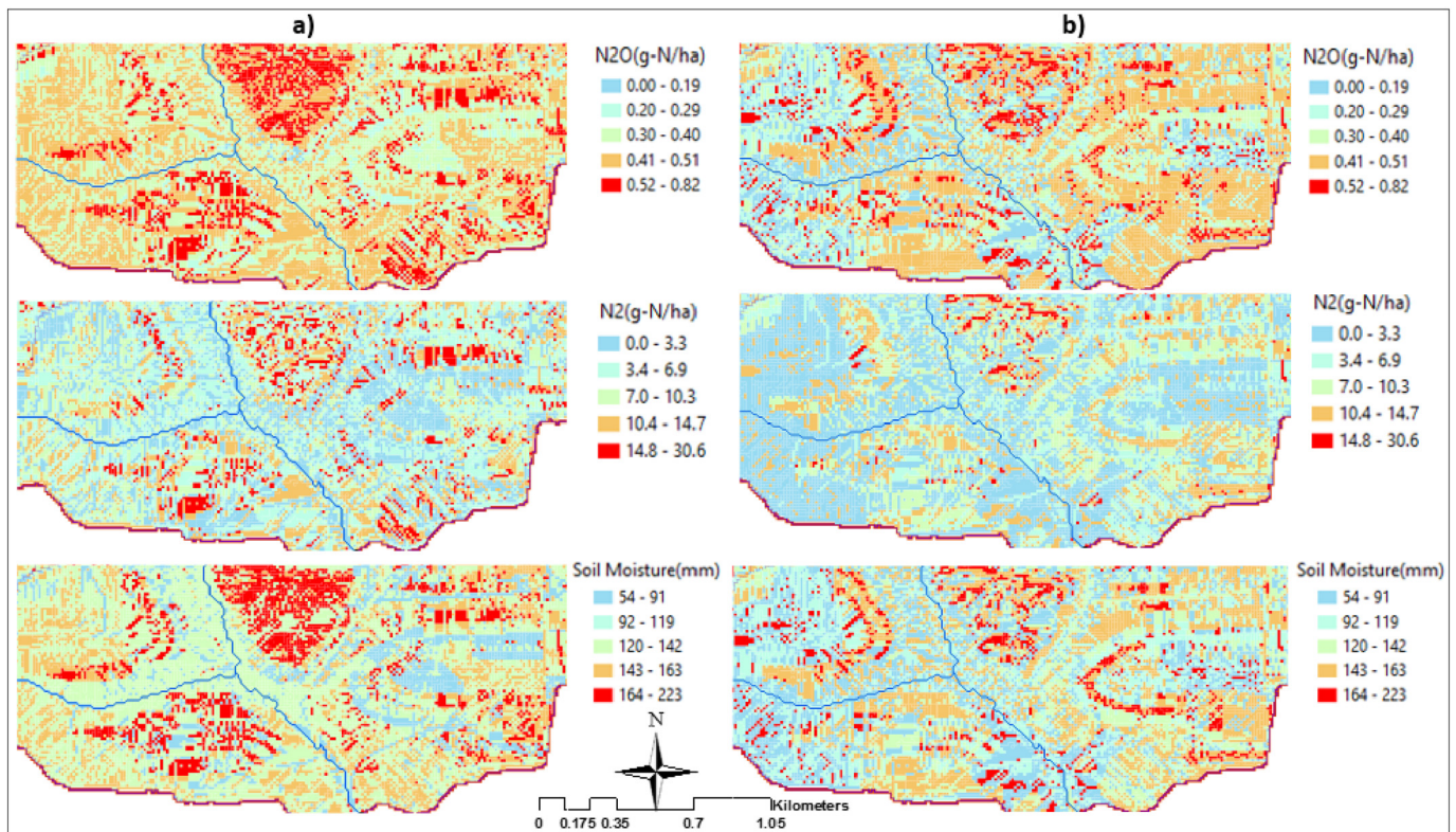
Fig. 6. Spatial comparison of wet (a) and dry (b) weather periods on mean daily N_2O and N_2 flux, and soil moisture conditions for the future ensemble model mean.
