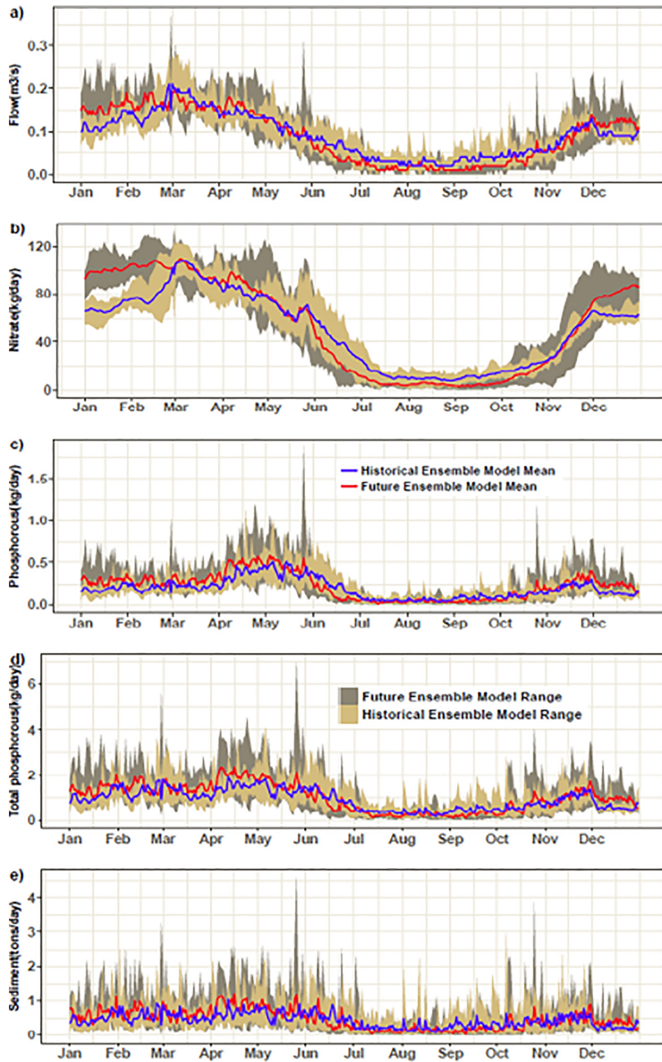
Fig. 3. Historical (1975–1998) and future (2045–2068) average-by-day from the ensemble model mean and the ensemble model range for streamflow (a), and the export of nitrate (b), dissolved P (c), total P (d), and sediment (e) for the seven regional climate models.
