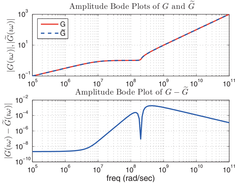
FIG. 3.1. Amplitude plots of \mathbf{G}(i\omega) and \tilde{\mathbf{G}}(i\omega) (upper); the absolute error |\mathbf{G}(i\omega) - \tilde{\mathbf{G}}(i\omega)| (lower).
