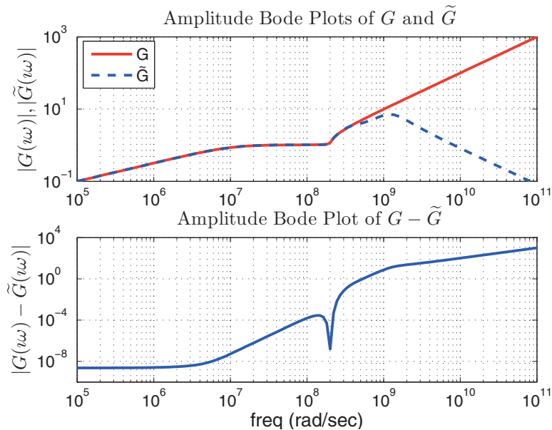
FIG. 2.2. Example 2.1: amplitude plots of \mathbf{G}(j\omega) and \tilde{\mathbf{G}}(j\omega) (upper); the absolute error |\mathbf{G}(j\omega) - \tilde{\mathbf{G}}(j\omega)| (lower).
