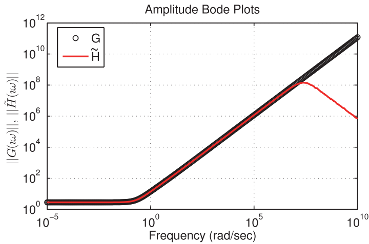
FIG. 6.4. Oseen equation: amplitude Bode plots of the full model \mathbf{G} and the reduced model \tilde{\mathbf{H}} , where \tilde{\mathbf{H}} is obtained without taking the underlying DAE structure into account.
