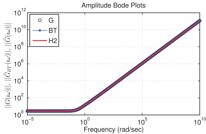
FIG. 6.1. Oseen equation: amplitude Bode plots of the full and reduced models.
