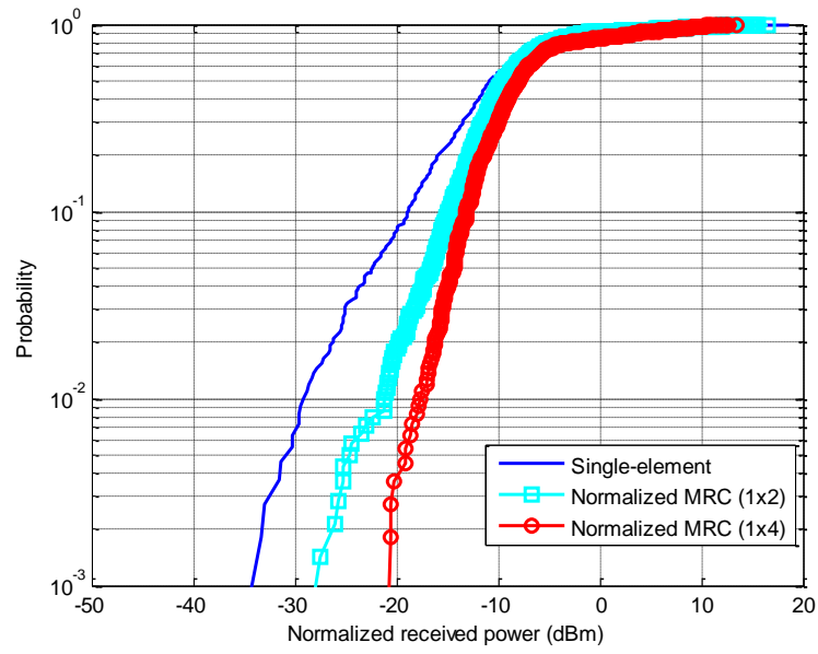
Figure 4.15: SIMO diversity: normalized received power CDF for Scenario 4 (Hospital)
