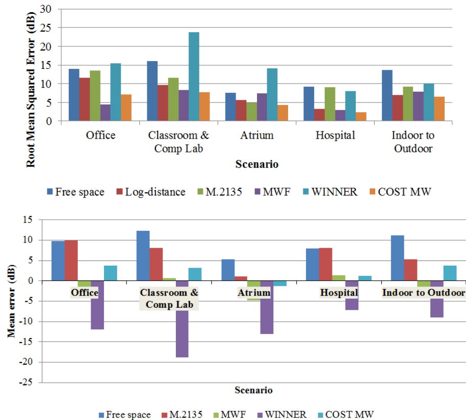
Figure 5.1: Prediction error of path loss models and measured path loss data. Top: RMSE Bottom: Mean Error
