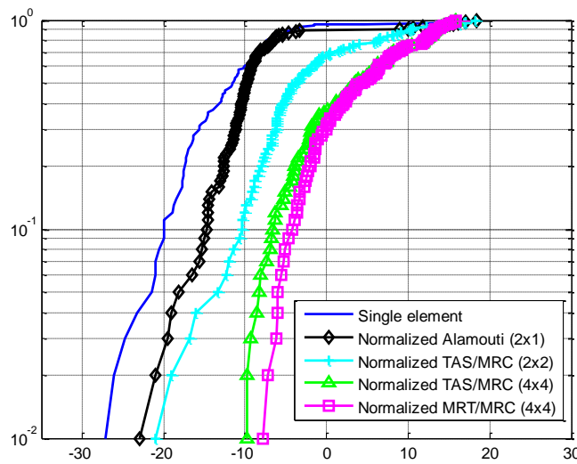
Figure 4.20: MIMO diversity: normalized received power CDF for Scenario 2 (Classroom/Comp Lab)
