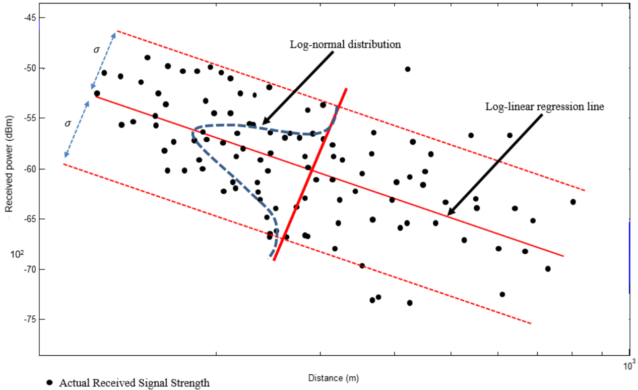
Figure 2.6: Sample received power measurements with log-normal shadowing
