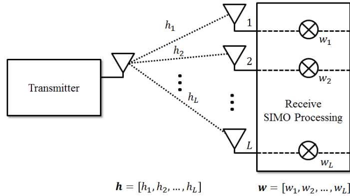
Figure 4.11: SIMO receive diversity processing
