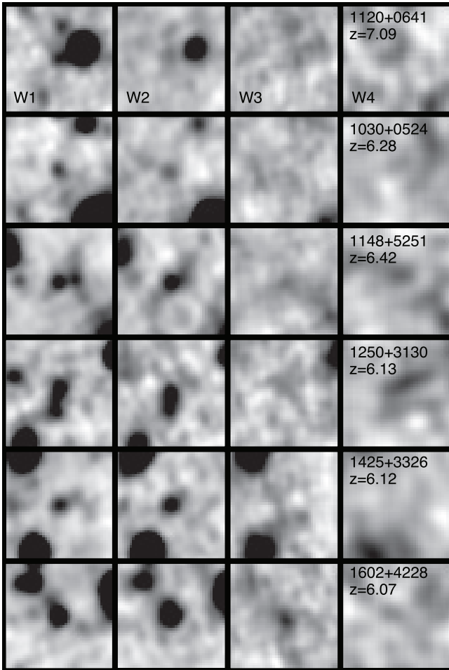
Figure 2. Postage stamp images, 60 arcseconds on a side, centered on the QSO position in WISE bands W1, W2, W3, W4 (from left to right along each row). From top to bottom, we show a different QSO in each row (labeled in the last column with their redshifts): ULAS J1120+0641, SDSS J1030+0524, SDSS J1148+5251, QSO J1250+3130, QSO B1425+3326/SDWFS J1427+3312, and SDSS J1602+4228. QSO J1250+3130 has a nearby companion, but far enough away from the WISE counterpart to ensure that the photometry remains accurate. The grayscale intensity is chosen to give an effective representation of the noise and so bright sources are saturated black.
