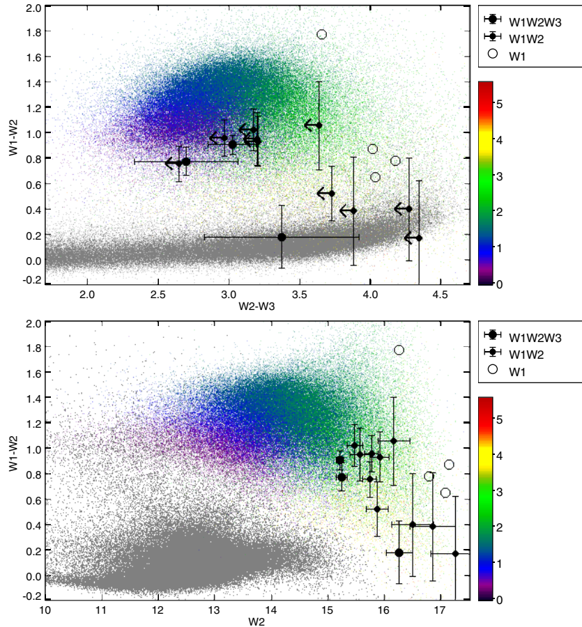
Figure 1. WISE color–color and color–magnitude diagrams for z > 6 QSOs (filled black circles) and a large sample of QSOs matched between SDSS and WISE (colored points) that are detected in all three relevant WISE bands. Large solid circles represent z > 6 QSOs with detections in all three of the bands W1/W2/W3. Smaller solid circles represent two-band detections in W1/W2. Open circles represent detections in W1 alone and are included for completeness only. Small filled circles with limit arrows represent the W2–W3 color if the W3 flux is at the limit listed in Table 1. The mid-IR properties of the SDSS QSO sample at z < 5.4 (colored field; Schneider et al. 2007) were obtained from a cross match with the WISE All-sky Data Release catalog. Cataloged WISE objects within 3.5 arcseconds of the reported SDSS QSO survey positions were assumed to be correct identifications. The gray (lower) cloud of points represents a sample of low-redshift galaxies (see Wright et al. 2010; Jarrett et al. 2011) to illustrate the underlying galaxy populations.
