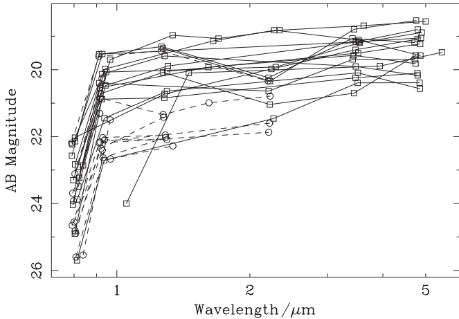
Figure 6. Observed-frame optical–mid-IR SEDs of z > 6 QSOs from the i -band ( 0.8 \mu\text{m} ) to WISE W2 at 4.6 \mu\text{m} . The two rightmost clouds of points represent WISE bands W1 and W2. The relative wavelength of different points in the clouds represent the relative redshift for each QSO, offset from the wavelength of the band center at a precise redshift z = 6 . There are only three significant detections at longer wavelengths from WISE , so we plot the SEDs only to reframe 5 \mu\text{m} . WISE -detected QSOs have SEDs that extend longward of 3 \mu\text{m} on the plot and are represented by square data points connected by solid lines, whereas WISE non-detected QSOs are represented by circular data points connected by dashed lines. Note that WISE -detected examples have typically slightly redder observed i - z colors (see Figure 5). Note that at z = 6(7) , \text{Ly}\alpha is at 0.85 ( 0.97 ) \mu\text{m} , potentially increasing the optical magnitudes, while \text{H}\alpha potentially enhances the W2 flux according to the template in vanden Berk et al. (2001), as shown by the Assef et al. (2010) template curves in Figure 4.
