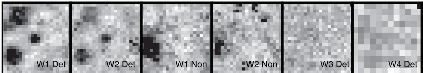
Figure 3. Results of stacking various combinations of the WISE images of z > 6 QSOs. From left to right, a stack of the W1 and W2 images for 16/17 of the W1-detected QSOs are shown as a comparison (W1 Det and W2 Det). Stacked W1 and W2 images for 10/14 of the non-detected objects with no nearby bright sources are then shown (W1 Non and W2 Non). Finally, W3 and W4 images are stacked from 13/14 W1-detected objects without W3 detections (W3 Det and W4 Det). Sources were excluded from the stacks on the grounds of a nearby brighter source that contributed light at the center of the stack; ULAS 1120+0641 alone was excluded from the detected (Det) sources. The total number of 8 s duration WISE single-exposure image frames combined in these stacks is 300, 300, 188, 188, 297, and 297 respectively.
