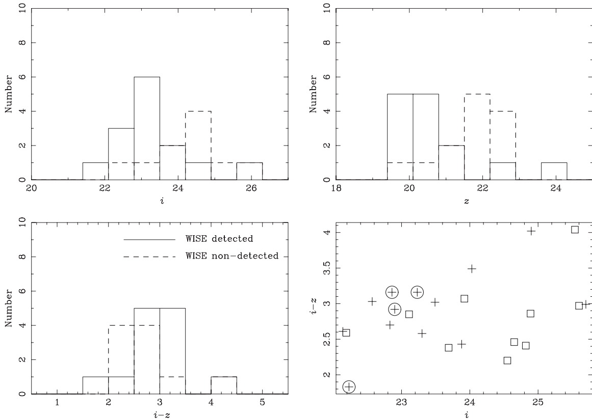
Figure 5. Observed-frame optical and IR properties of z > 6 QSOs with i - and/or z -band data. In the histograms, the WISE -detected (solid lines) and WISE -non-detected (dashed lines) QSOs have distinct properties, with the WISE -detected QSOs being brighter and redder at restframe 0.15 \mu\text{m} . The color–magnitude diagram shows all 24 of the z > 6 QSOs with i - and z -band data. Crosses show the 14 WISE -detected QSOs listed in Table 1. Boxes represent WISE -non-detected QSOs with i - and z -band data (10 in total). Circles highlight the QSOs with detections with Spitzer (Hines et al. 2006; Jiang et al. 2006; McGreer et al. 2006; Stern et al. 2007; Jiang et al. 2010; see Table 1). An outlier, QSO J1630+4012, has been removed (Kim et al. 2009). All magnitudes are AB.
