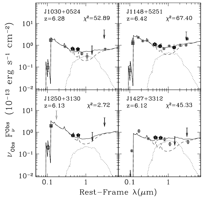
Figure 4. SEDs of four secure WISE 2/3 band detections from the z > 6 QSO sample. A combination of different SED component templates (Assef et al. 2010), which were developed for data in the NDWFS Bötotes field and are adequate to describe the WISE data, are also shown for an AGN (solid line) and an evolved stellar population (dotted line). The addition of other template components, for example, for a star-forming galaxy (Sbc/Im) component, does not improve the fits. The WISE data is highlighted by filled black pentagons and upper limits at the longer wavelengths. SDSS data is represented by gray squares and Spitzer and other sources by gray circles. J1250+3130 provides a good example of how data from WISE can provide a valuable insight into the relative strengths of different SED components from a typical WISE -detected example without Spitzer data. The sources of the data are referenced in Table 1. In all four cases, the WISE data and limits in W1 and W2 clearly limit the possible contribution from an evolved stellar population, while the information from W3 and W4 provides a valuable limit to the possible normalization and/or slope of the power-law mid-IR AGN component in the event that Spitzer data was not available, as is the case for J1250+3130. Clearly, the availability of Spitzer data provides much more information.
