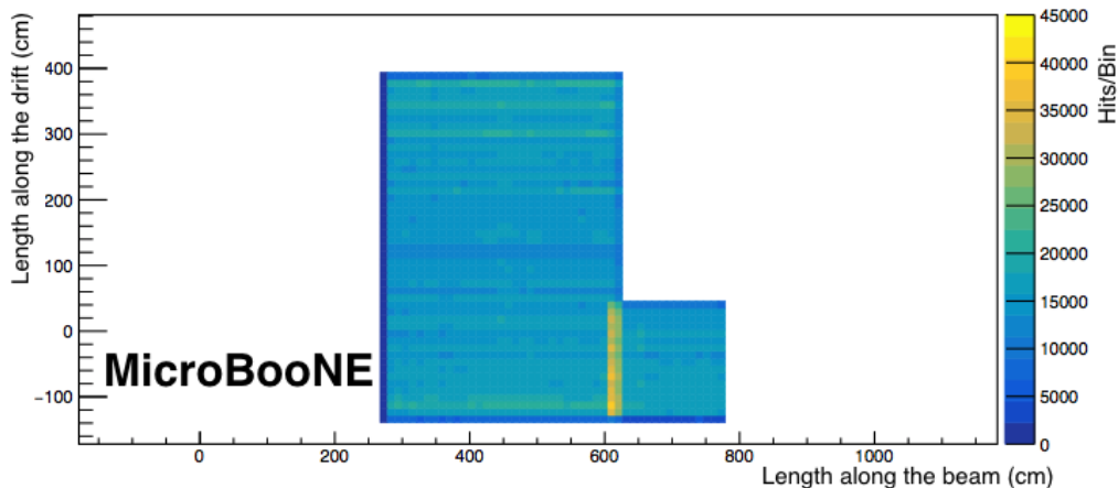
Figure 27. Map of CRT hits in the bottom plane (color version online). The overlap of modules (hotter zones) and the cryostat shadow are visible compared to figure 2.
