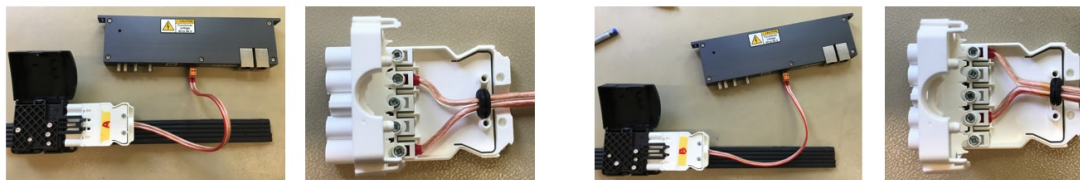
Figure 21. Connection between the flat cable and FEB. Cable adapters are installed on the cable for two modes A and B. Corresponding male connectors are applied to match the FEB audio cable.
