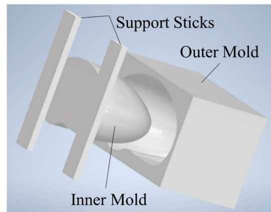
Fig. 2 Hemispheric bilayer mold configuration
