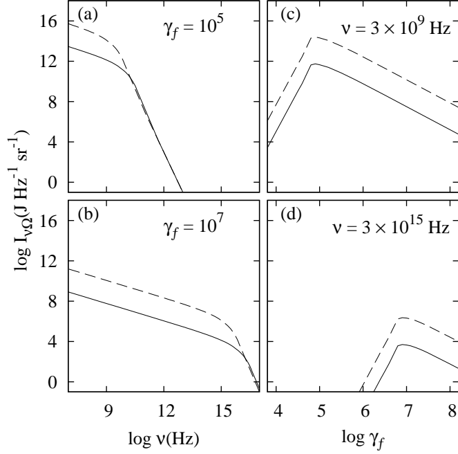
Figure 1: Electromagnetic-pulse energy spectrum for a topological phase transition (solid curves, efficiency \eta \approx 0.01 ), and a final explosive burst as described by Rees and Blandford (dashed curves, efficiency \eta \approx 1 ). (a) shows the pulse energy per unit frequency interval, versus frequency, for a fireball Lorentz factor \gamma_f = 10^5 . (b) is for \gamma_f = 10^7 . (c) shows the pulse energy per unit frequency interval versus \gamma_f , at frequency 3 \times 10^9 Hz. (d) is for frequency 3 \times 10^{15} Hz. Note that the curves in (c) and (d) peak sharply at a specific \gamma_f , dependent on the observing frequency (full-width at half-maximum \approx 1/3 , in \log \gamma_f ). So, choosing an observing frequency enables searching for events of a particular \gamma_f . For a topological phase transition, a \gamma_f is associated with an extra dimension of a particular size (see text). Pulses for the cases \eta \approx 0.01 and \eta \approx 1 can be distinguished. In (c), for example, the output energy is dramatically different for the two cases, at the \gamma_f of peak output. Thus, a distance to the object (e.g., from pulse dispersion measure for radio observations) would distinguish the two cases. A pulse for \eta \approx 1 can have the same energy as for \eta \approx 0.01 only for a significantly different \gamma_f , which could be determined by sampling the spectrum at multiple wavelengths.
