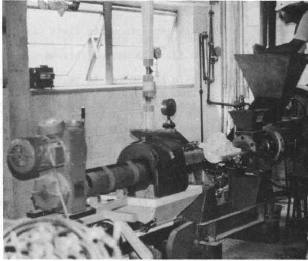
Figure 5. Processing of experimental floating diets for caged catfish
