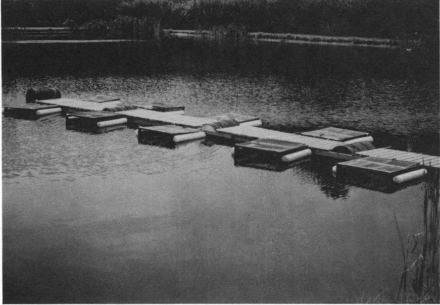
Figure 4. Layout of cages used in field experiment
