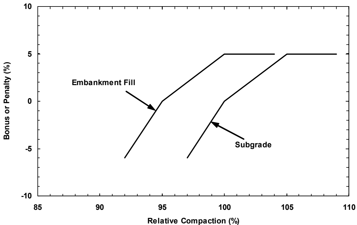
Figure 2. Bonus or Penalty versus Relative Compaction
