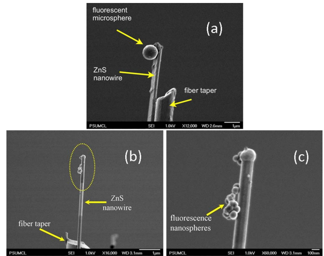
FIG. 2. (Color online) [(a) and (b)] field emission scanning electron microscope images of a nanoprobe attached with a single fluorescent microsphere ( \sim 1 \mu\text{m} diameter) and a nanoprobe attached with multiple fluorescent nanospheres ( \sim 100 \text{ nm} diameter), respectively; (c) zoomed-in view of the tip of the two photon nanoprobe shown in (b).
