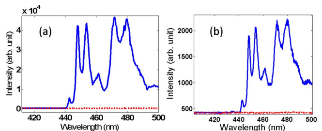
FIG. 3. (Color online) (a) two-photon fluorescence spectrum of a type I nanoprobe with a single 1 \mu\text{m} sphere (solid blue curve) and spectrum of ZnS nanowire only (dotted red curve), (b) two-photon fluorescence spectrum of a type II nanoprobe with multiple fluorescent nanospheres ( \sim 100 \text{ nm} diameter) (solid blue curve) and spectrum of ZnS nanowire only (dotted red curve).
