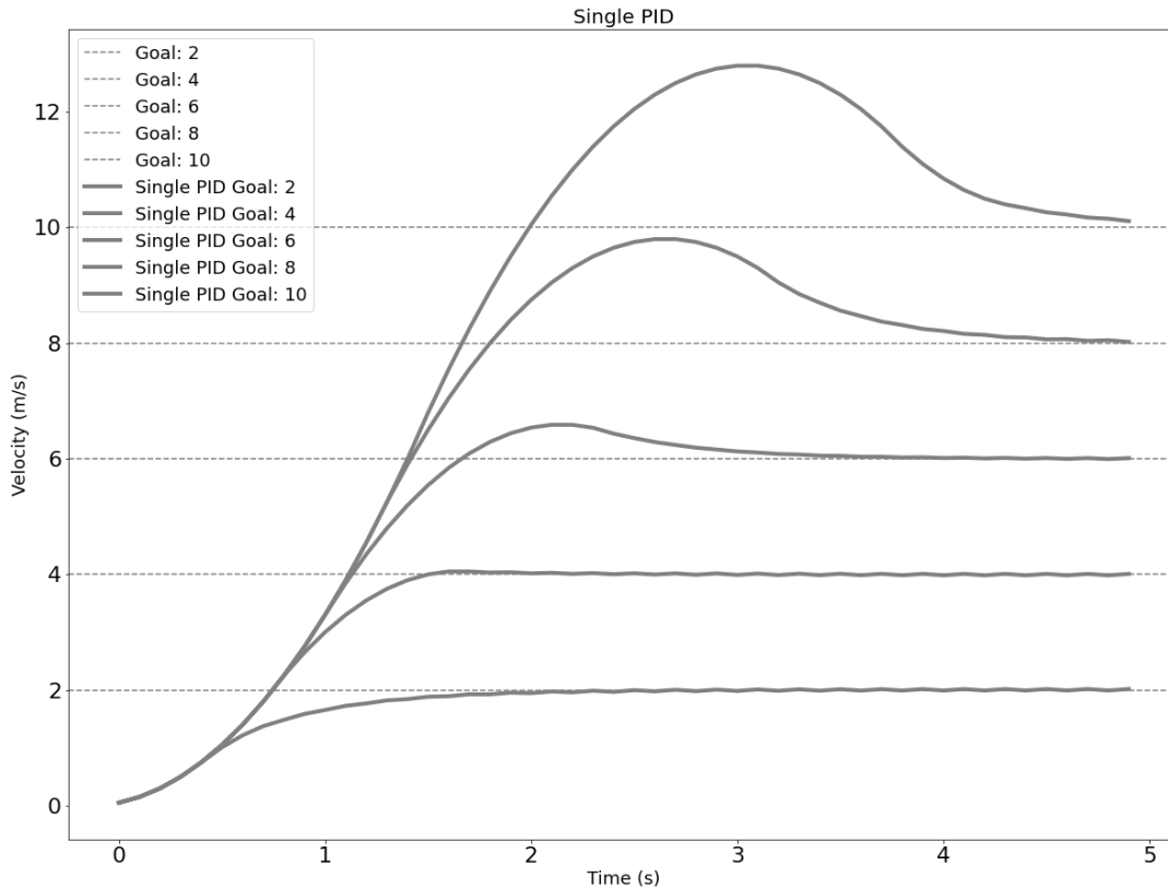
Figure XX: Velocity given a set of single PID Values
