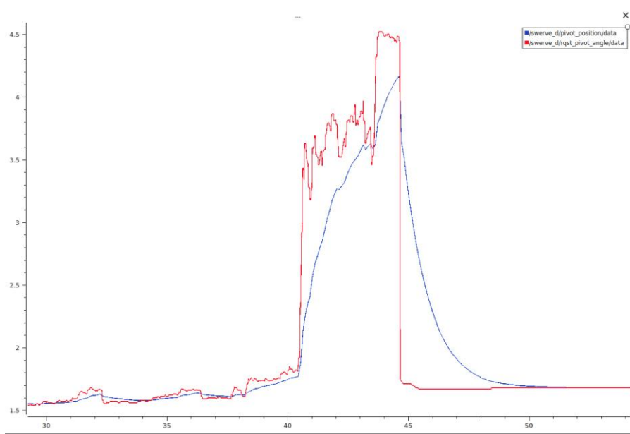
Figure XXV: PID Controller of Pivot Angle
