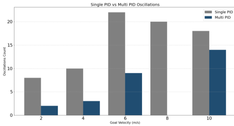
Figure XXIII: Oscillation Comparison
