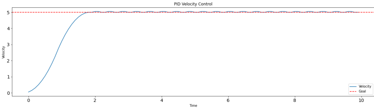
Figure XVIII: Manual tuning within select range of values
