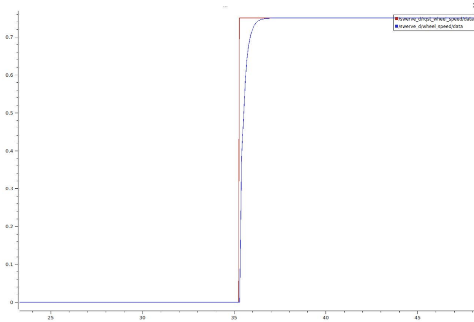
Figure XXVI: Wheel Speed PID Example
