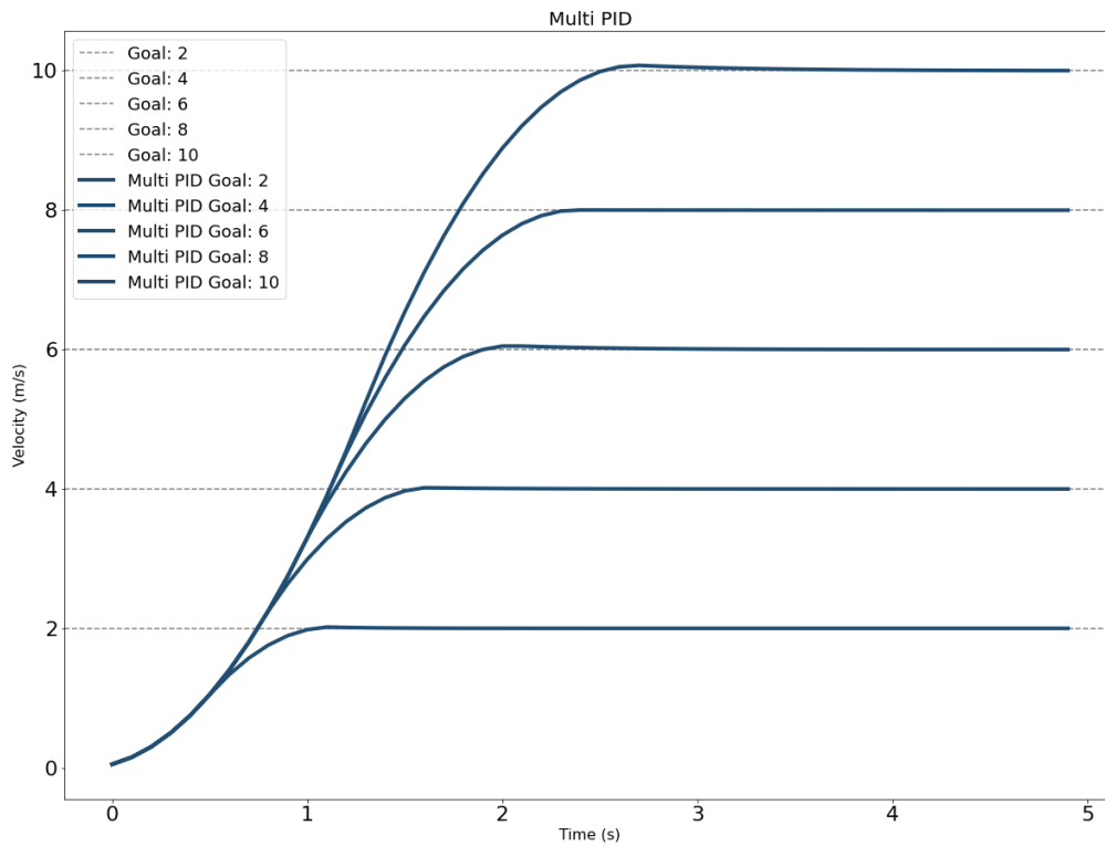
Figure XXI: Multi-Tuned Discrete PID
