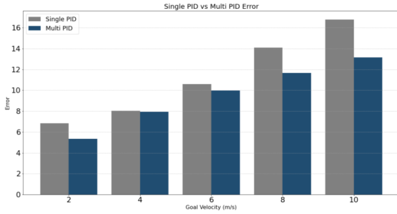
Figure XXII: Normalized Error Comparison
