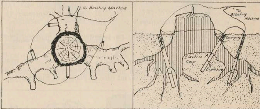
Fig. 7—Electric Method of Loading Distributed Charges Under and Around a Large Lateral-root Stump
