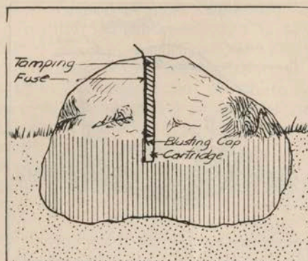
Fig. 8—Block Holing Method of Loading Charge
