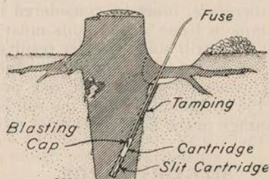
Fig. 2—Location of Bore Hole and Cap-and-Fuse Charge in a Tap-Root Stump
