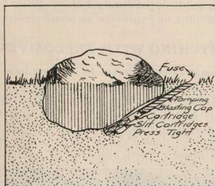
Fig. 9—Snake Holing Method of Loading Charge
