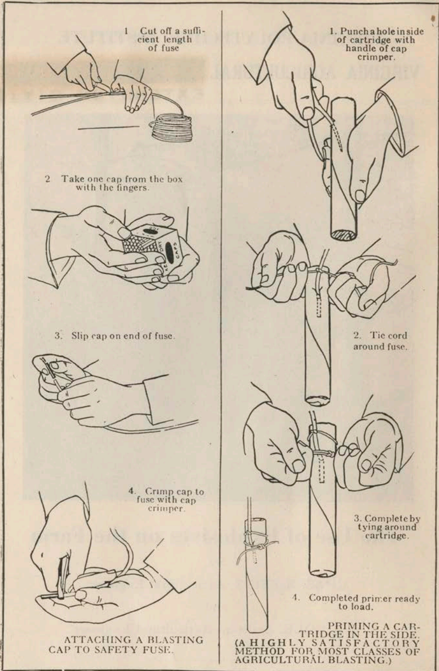
Fig. 1—Approved Method of Attaching Blasting Cap to Fuse and Priming a Cartridge
