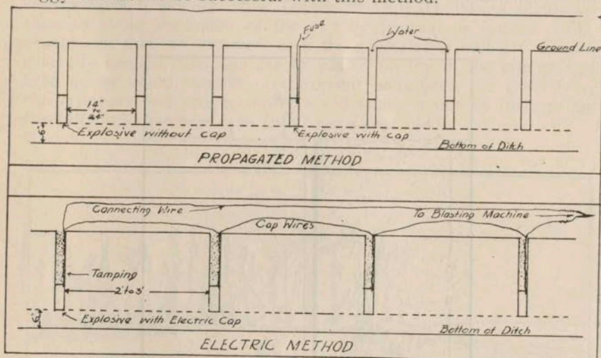
Fig. 12—System of Loading for Propagated and Electric Methods of Ditching
