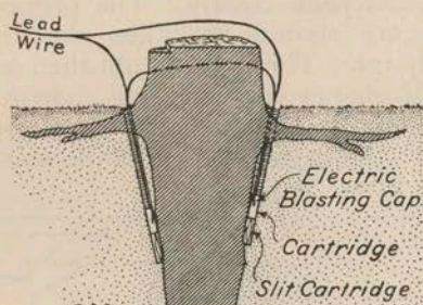
Fig. 3—Method of Loading for Blasting Tap-root Stump with Distributed Charges Electrically Fired
