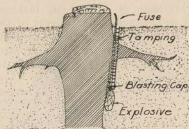
Fig. 4—Method of Loading for Blasting Tap-root Stump with Cap and Fuse Charge
