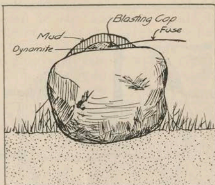
Fig. 10—Mud Capping Method of Loading Charge
