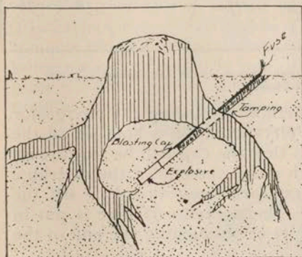
Fig. 5—Method of Loading a Lateral-root Stump with a Single Charge
