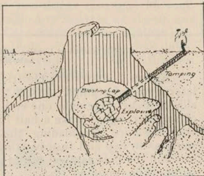
Fig. 6—Method of Loading Large Lateral-root Stump
