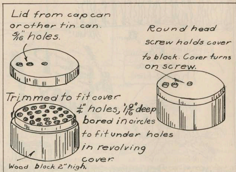
Fig. 14—A Home Made Safe Cap Box
