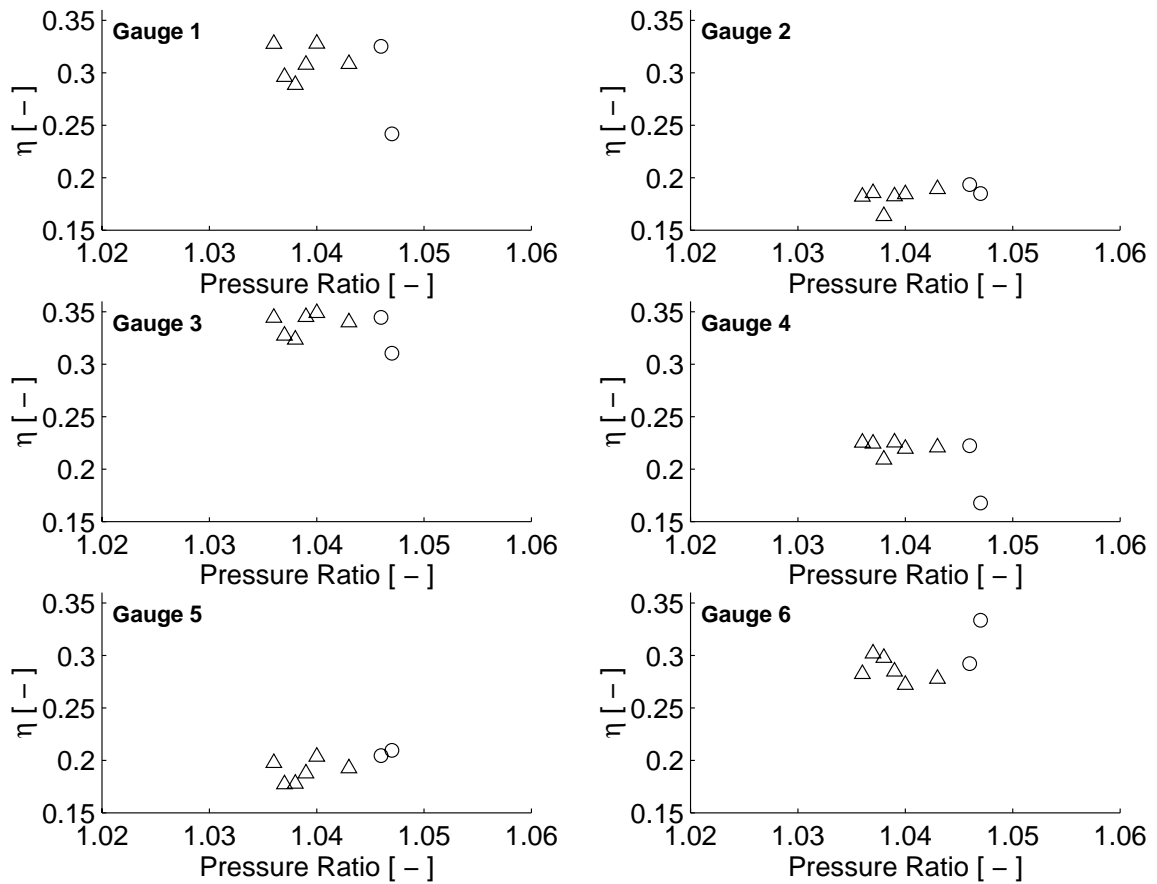
Figure E.2: Measurement Repeatability of Effectiveness at PR=1.04.
