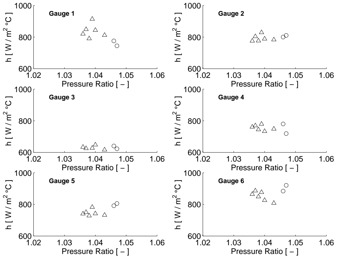
Figure E.1: Measurement Repeatability of Heat Transfer Coefficient at PR=1.04.
