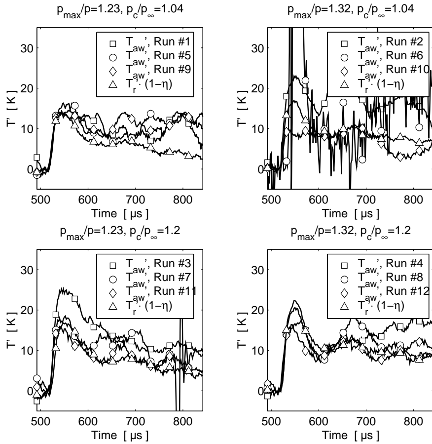
Figure 3.35: Comparison between T'_{aw} and T'_r \cdot (1 - \eta) for all Experiments with Film Cooling. Results from Gauge #3.
