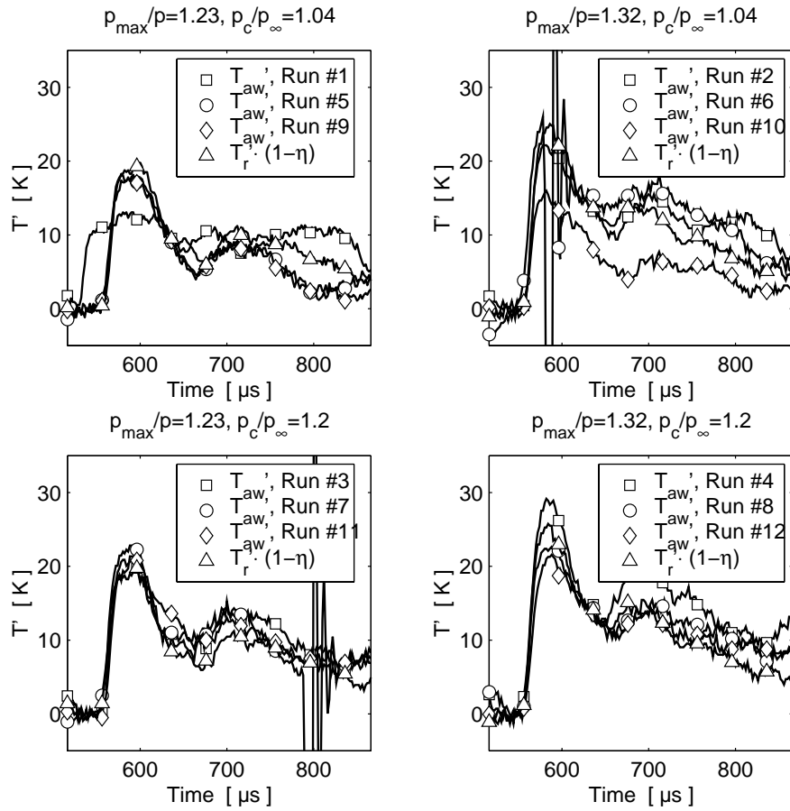
Figure 3.34: Comparison between T'_{aw} and T'_r \cdot (1 - \eta) for all Experiments with Film Cooling. Results from Gauge #2.
