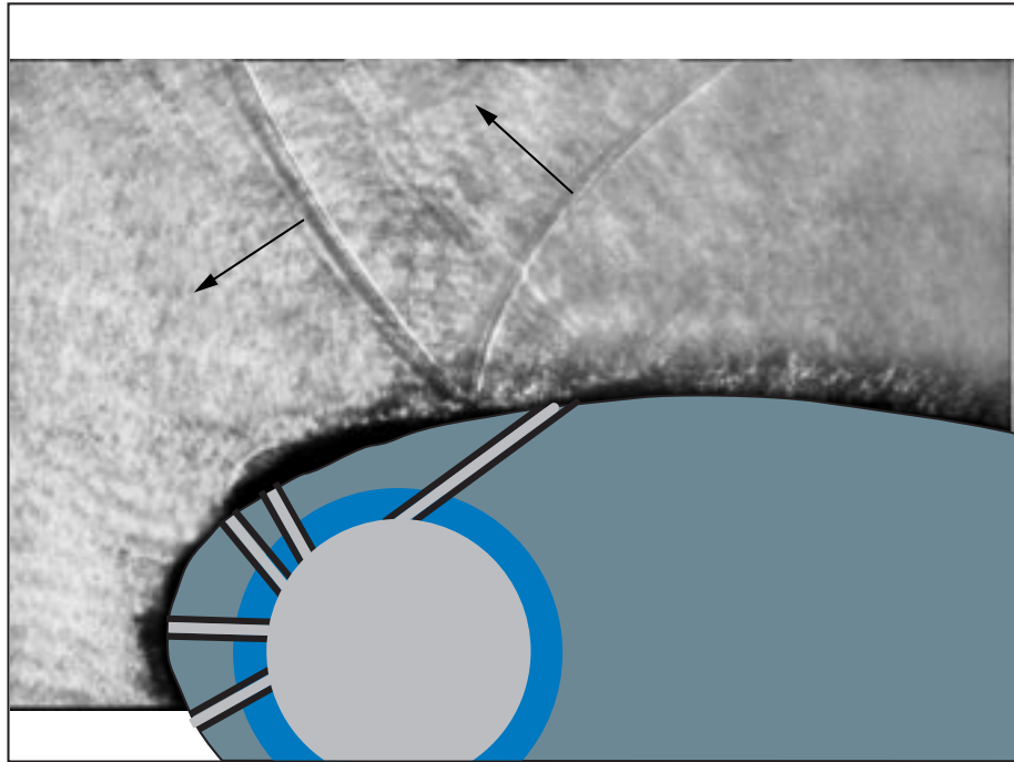
Figure A.7: Shock Progression: Still # 7, time \approx 622\mu s .
