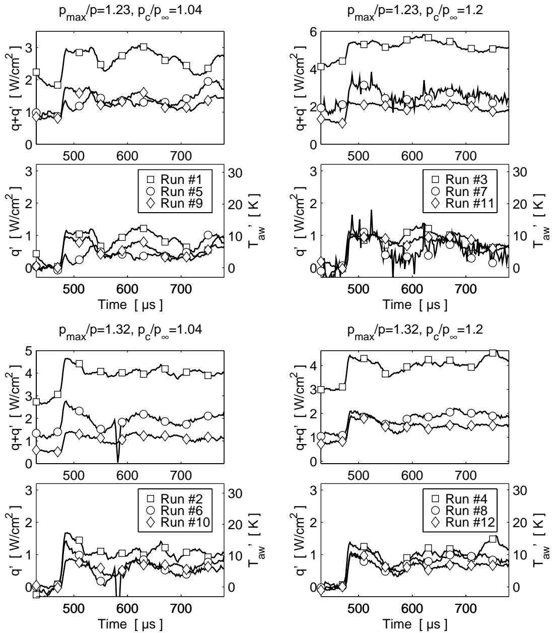
Figure 3.31: Shock Passing Events for Gauge # 5 at Different Shock Conditions with Film Cooling. Three Experiments at Different Levels of Initial Heat Flux for Each Shock and Cooling Strength. Top Graphs: Absolute Values. Bottom Graph: Initial Value Subtracted.
