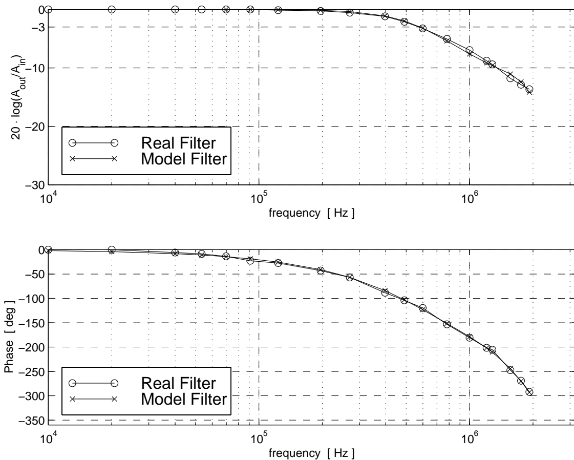
Figure B.2: Transfer Function of the Measurements Group 2310 Strain Gauge Conditioner and Signal Amplifier at a gain of 1.
