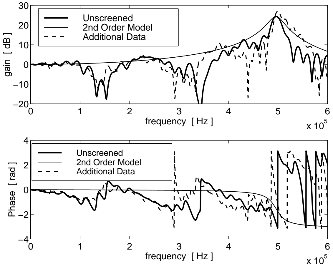
Figure B.9: Bode Plot of Transfer Function of Unscreened Sensor.
