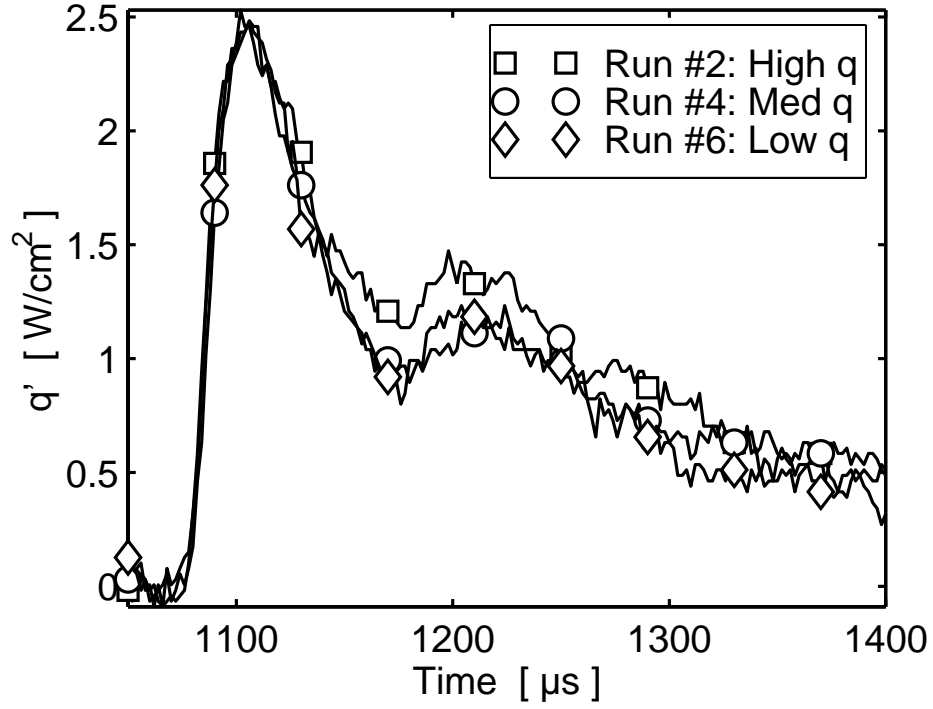
Figure 3.17: Shock Passing Events for Gauge # 2 at Increased Shock Strength without Film Cooling. Three Experiments at Different Levels of Initial Heat Flux. Initial Level of Heat Flux Removed.
