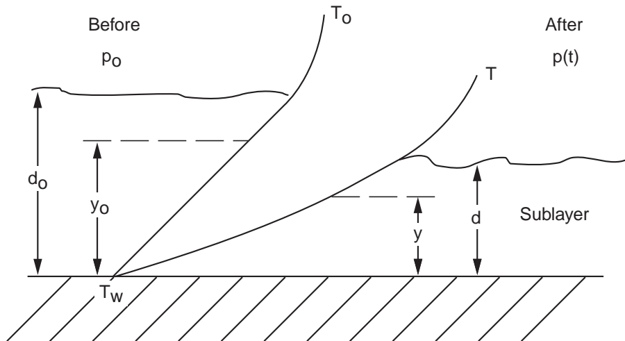
Figure 3.51: Change in Laminar Sublayer Temperature Profile from T_o to T Due to Compression and Heating Induced by Pressure Change. From Rigby et al. (1989).
