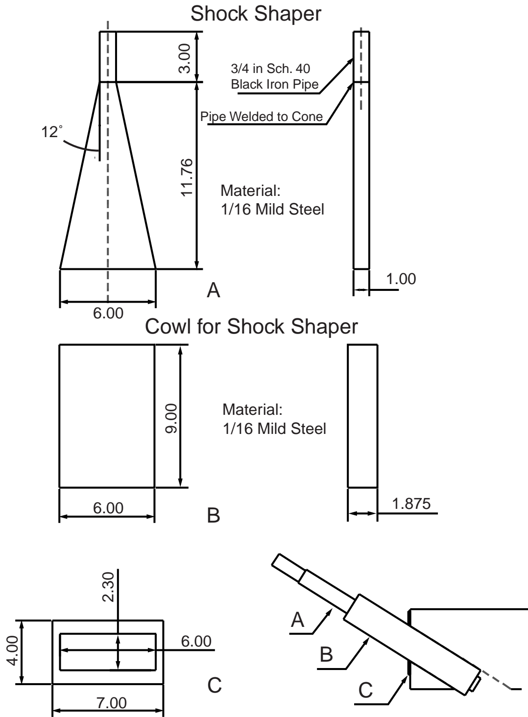
Figure 3.2: Shock Shaper Design.
