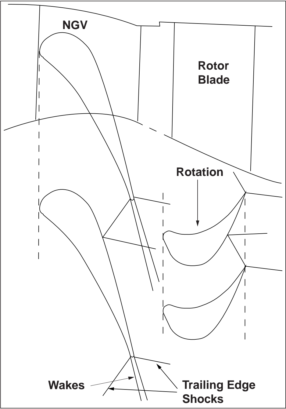
Figure 1.2: Schematical Depiction of the Non-Uniformity of the Flowfield Downstream of a Modern NGV Row.
