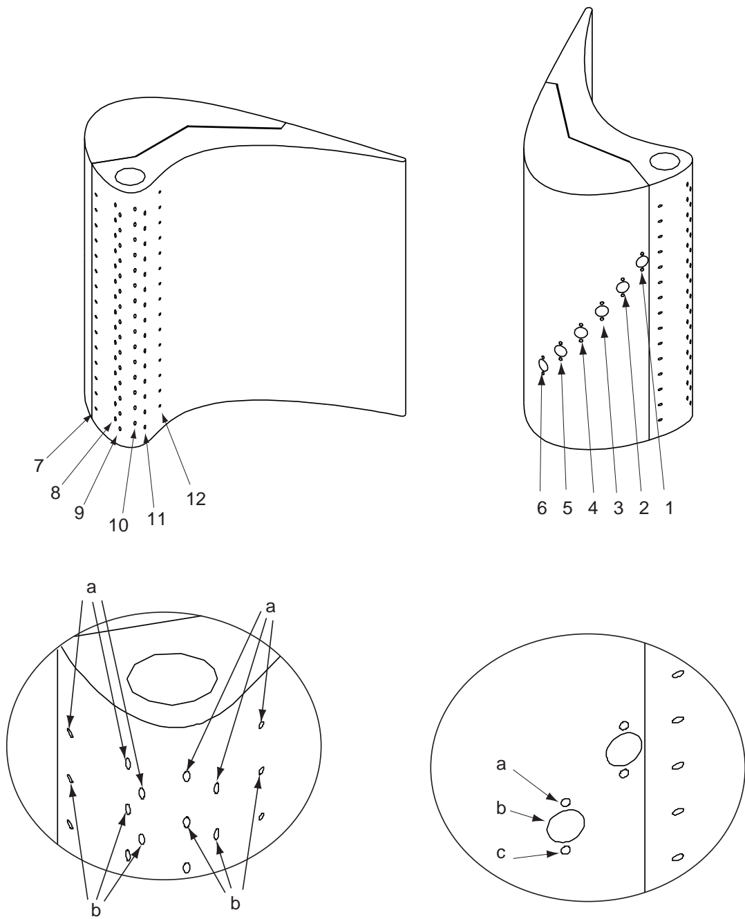
Coolant Exit Enlargement
