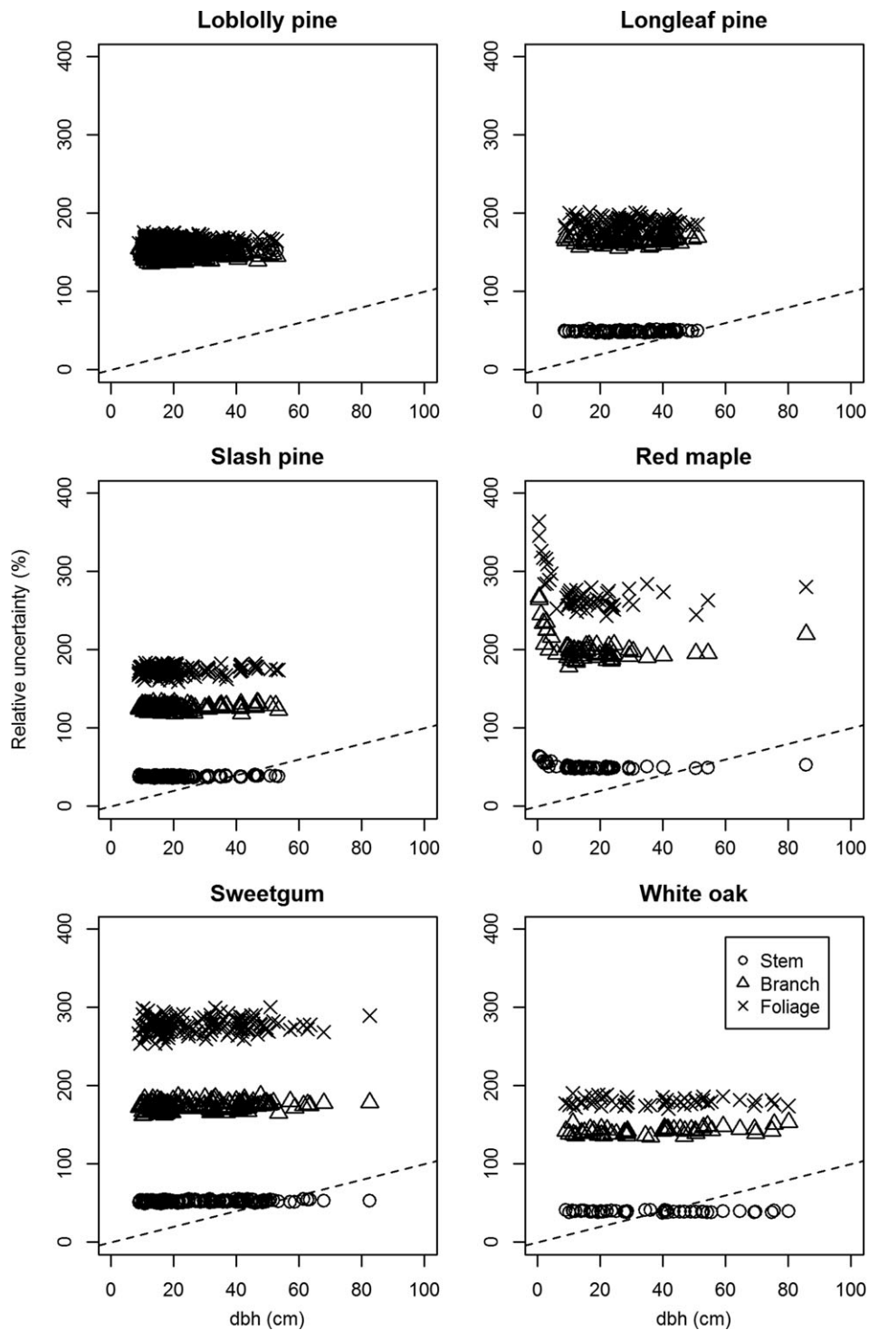
Figure 3 Relative uncertainty of component biomass predictions (95% posterior uncertainty interval/posterior mean) vs dbh.
