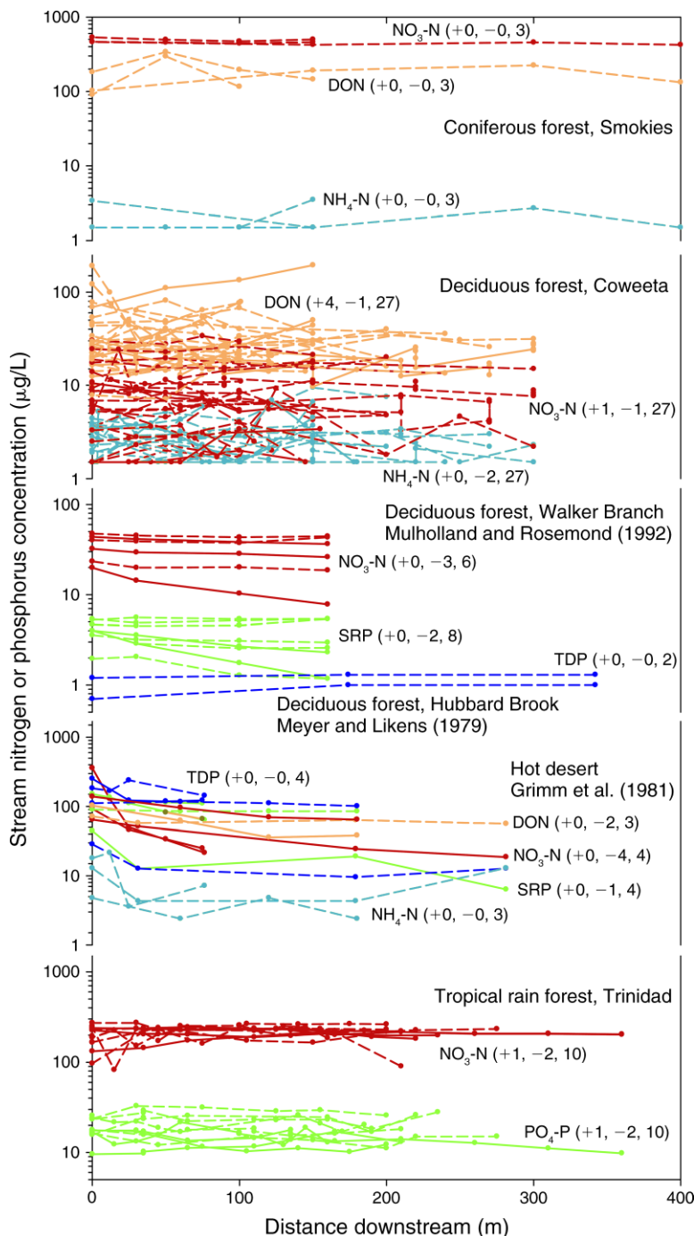
FIG. 1. Longitudinal profiles of ambient stream nitrogen and phosphorus chemistry collected in watershed streams. Profiles are for \text{NO}_3^- (nitrate), \text{NH}_4^+ (ammonium), DON (dissolved organic N), SRP (soluble reactive P), \text{PO}_4^{3-} (phosphate), and TDP (total dissolved P). Values are original data or are taken directly or digitized from publications. Numbers in parentheses represent, in order, (1) the number of significant ( P < 0.05 ) regressions with positive (+), and (2) negative (-) slopes, and (3) the total number of longitudinal profiles. Statistically significant profiles are shown as solid lines, and nonsignificant profiles as dashed lines.
