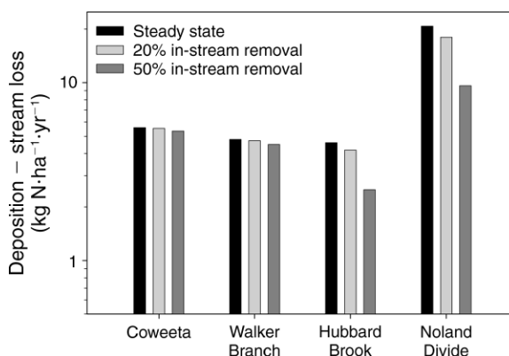
FIG. 3. Potential contribution of in-stream N removal to watershed N balance for sites with long-term N budgets. We consider three scenarios: (1) at steady state, Q_G[N]_G = Q[N] (where Q_G is net groundwater inflow, Q[N] is the long-term mean N export, and [N]_G is the groundwater concentration of N) and therefore watershed balance equals observed atmospheric N deposition minus observed stream N losses; (2) Q[N] = 0.8 \times Q_G[N]_G , or 20% removal; and (3) streams remove half of terrestrial N losses.
