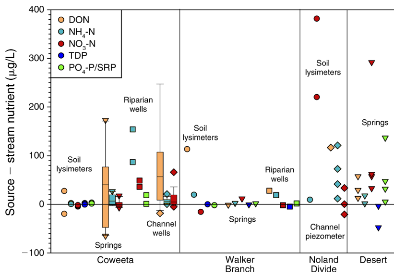
FIG. 2. Potential sources of [M]_G (groundwater concentration of nutrient mass) for streams examined in this study. Samples are from zero-tension lysimeters placed below B and C horizons (circles), springs (triangles), permanent near-stream riparian wells (squares) and hyporheic wells and stream sediment piezometry (diamonds). Symbol colors in circles apply to all sample (and symbol) types. Data for desert streams represent upstream groundwater source (spring) chemistry. Data are individual samples or box plots with 95% confidence limits and outliers, displayed as potential source minus mean stream concentrations.
