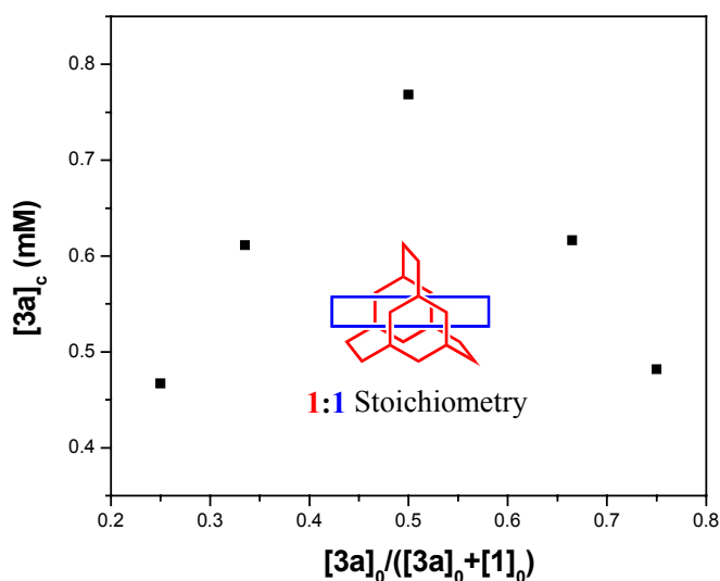
Figure 2. Job plot: the stoichiometry of the complex between 3a and 1 in CD_3COCD_3 solution using data for the aromatic hydrogen atom of 3a . [3a]_c is the concentration of complexed 3a . [3a]_0 + [1]_0 = 2.00 mM.
