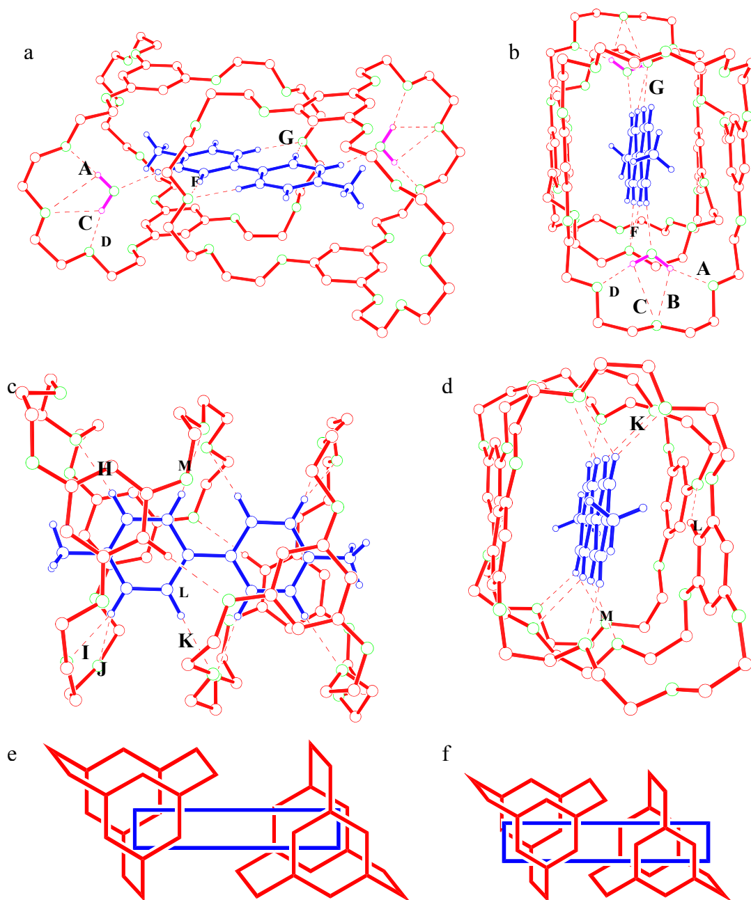
Figure 4. Solid state structures of 3b•1•3b (a and b) and 3a•1•3a (c and d) and cartoon representations of 3b•1•3b (e) and 3a•1•3a (f). Hosts ( 3a or 3b ) are red, the guest ( 1 ) is blue, and water molecules are magenta. (a) and (b) Four water molecules, two acetone molecules, two \text{PF}_6^- ions, and hydrogens except the ones in paraquat and water molecules have been omitted for clarity. Hydrogen-bond and face-to face \pi -stacking parameters are listed in Tables 1 and 2. (c) and (d) One disordered acetone molecule, two \text{PF}_6^- ions, and
