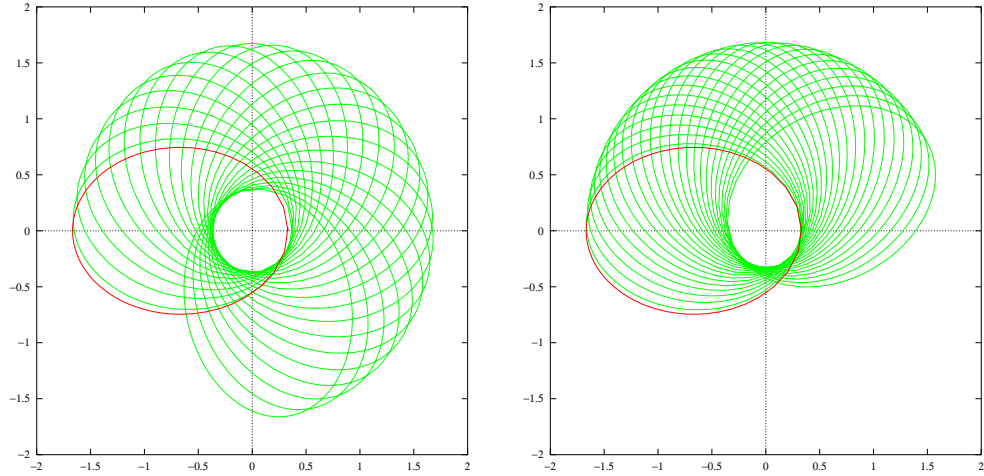
FIG. 2: The trajectory of a mass in a coulomb potential with r_+/r_- = 5 , 2m|E|\beta = 0.01 , \beta' = 0 (left), and \beta = 0 , 2m|E|\beta' = 0.01 (right). The length scale is in units of (r_+ + r_-)/2 . The red line indicates the orbit when \beta = \beta' = 0 . The motion is counter clockwise along the trajectory starting from the perihelion on the positive x axis. 25 complete revolutions are shown. For both cases, the trajectory is precessing clockwise.
