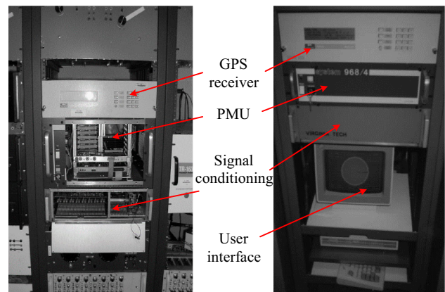
Fig. 2 First set of PMUs built at Virginia Tech
