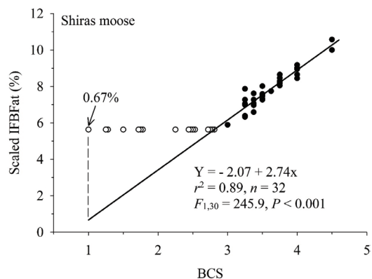
Fig. 1. Ingesta-free body fat (IFBFat) relative to body condition score (BCS) of adult female Shiras moose during mid-February 2012, Sublette County, western Wyoming, USA. Solid circles represent individuals with measurable subcutaneous rump fat and open circles represent individuals without measurable rump fat.
