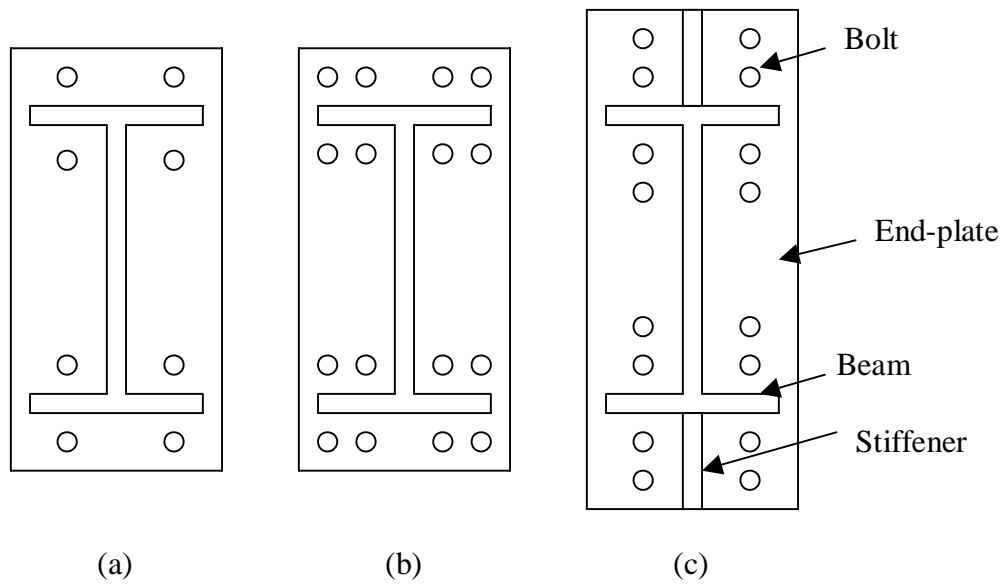
FIGURE 1-2. Typical moment end-plate configurations; (a) four-bolt extended, (b) four-bolt wide, (c) eight-bolt extended stiffened.
