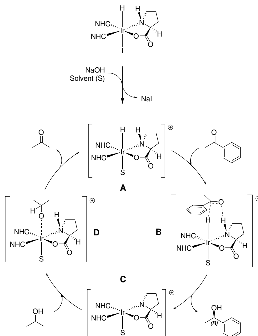
Scheme 4. Proposed catalytic cycle for ATH of aryl ketones in this system, where S is representative of the solvent (IPA). Steps: A . solvent complexed cationic resting state of catalyst; B . positioning of substrate with hydride attacking the carbonyl carbon and N-H bonding to carbonyl oxygen; C . elimination of reduced product; D . coordination of isopropanol followed by reductive elimination to regenerate metal hydride (A). Metal-ligand bifunctional catalysts of this type typically operate through an outer-sphere mechanism, where the substrate does not directly bind to the metal center.
