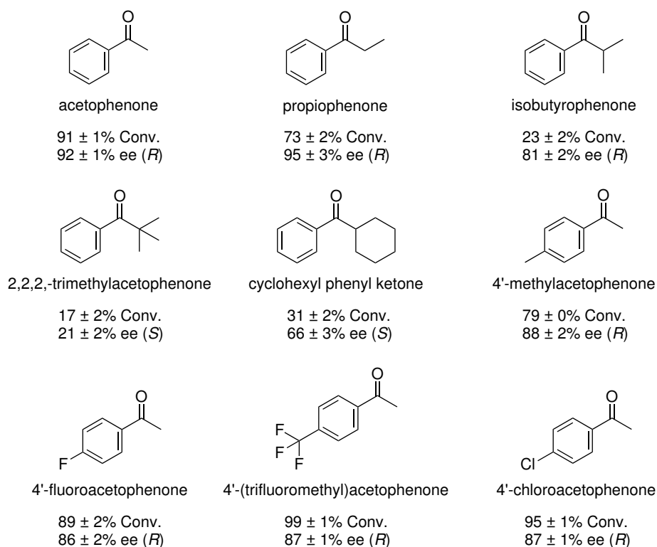
Figure 13. Substrate scope for ATH of ketones catalyzed by \text{Ir}(\text{IME})_2(\text{L-Pro})(\text{H})(\text{I}) . All reactions were carried out using the optimized catalytic conditions.
