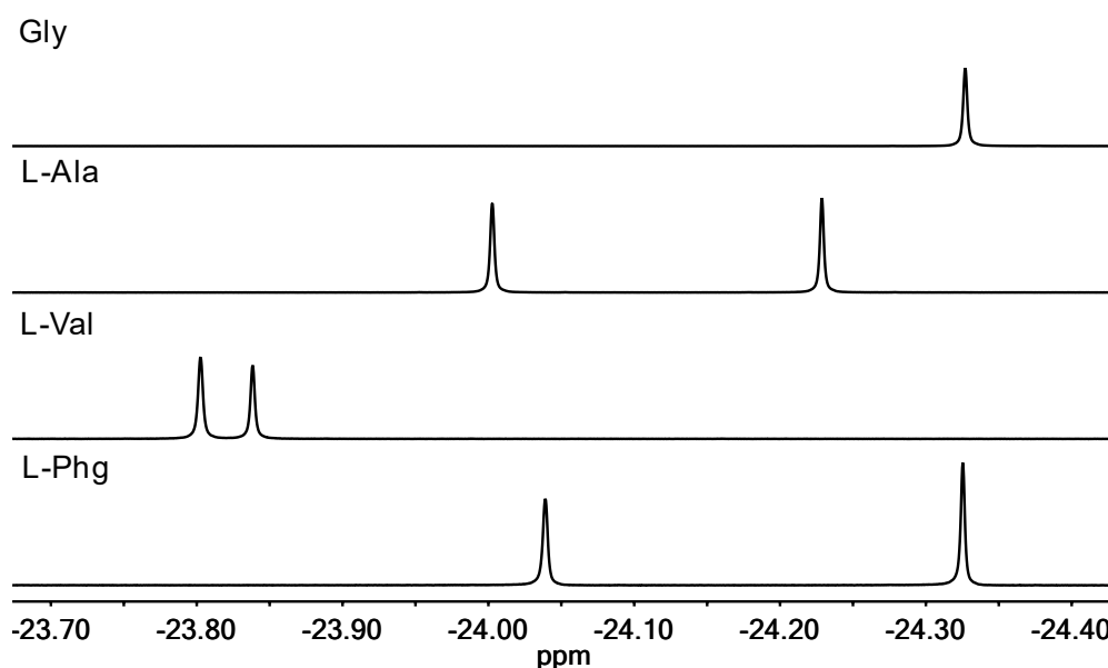
Figure 7. ^1\text{H} NMR spectra (400 MHz, \text{DMSO-}d_6 ) showing the hydride resonances for complexes of the form \text{Ir}(\text{IME})_2(\text{aa})(\text{H})(\text{I}) , where aa = glycine, L-alanine, L-valine, and L-phenylglycine.
