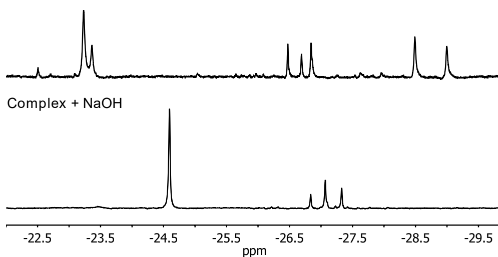
Figure 8. 1 H NMR spectra (400 MHz, IPA, DMSO- d 6 insert) showing the hydride resonances of Ir(IMe) 2 (L-Pro)(H)(I) before ( top ) and after ( bottom ) the addition of NaOH.
