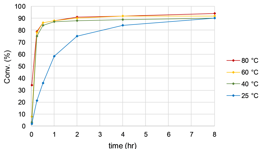
Figure 9. Conversion of acetophenone over time at various temperatures. All conversions appeared to level off after a period of 8 h.
