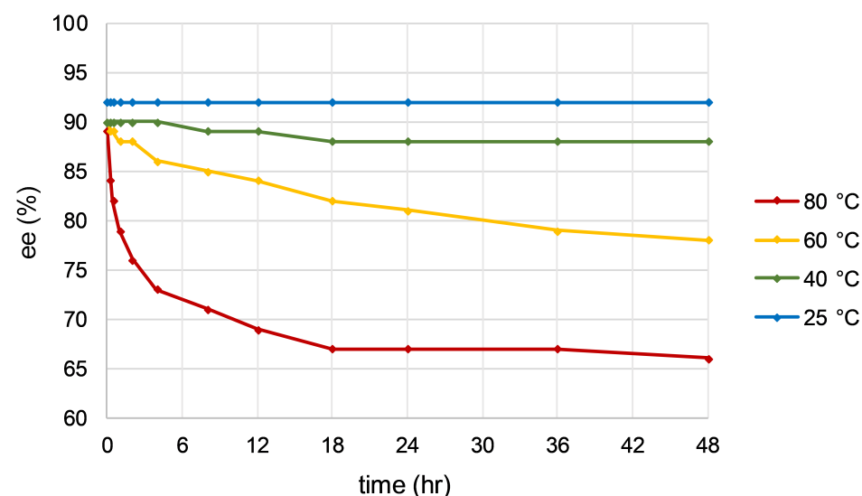
Figure 10. Enantiomeric excess of 1-phenylethanol over time at various temperatures. Enantioselectivity degraded over time at temperatures above 25 \text{ }^\circ\text{C} .
