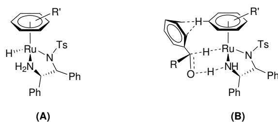
Figure 1. (A) Structure of Noyori's ruthenium arene TsDPEN active catalyst for ATH of ketones. (B) Noyori's catalyst operates through a concerted outer-sphere mechanism where the substrate does not directly bind to the metal center. For aryl ketone substrates, the transition state is stabilized by CH/ \pi interactions between the catalyst and ketone.
