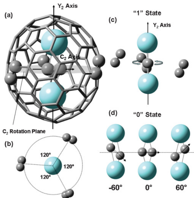
FIG. 5. (Color online) (a) Y_2C_2@D_3(85)-C_{92} with planar Y_2C_2 unit and 6-6-5 cage intersections identified as gray spheres of the cage. The C_2 axis is parallel to the C_2 rotation plane (defined by the 6-6-5 cage intersections) and perpendicular to the Y_2 axis, which is orthogonal to the C_2 rotation plane. The Y_2 axis and C_2 axis are defined as the axis connecting the homopolar ( A_2 , A = Y, C ) molecule which is coincident with the chemical bond. (b) Top view of the C_2 rotation plane, which indicates a repulsive interaction between the C_2 rotor and the 6-6-5 cage intersections after every 120^\circ of rotation about the Y_2 axis. (c) "1" state; all C_2 rotations about the Y_2 axis remain parallel to the C_2 rotation plane due to an applied voltage (100 meV) which removes the effect of the rotational barrier V(\theta) . (d) "0" state; C_2 rotations about the Y_2 axis alternate between three states, -60^\circ , 0^\circ , and 60^\circ , which tunnel through the C_2 rotation plane due to the rotational barrier V(\theta) .
