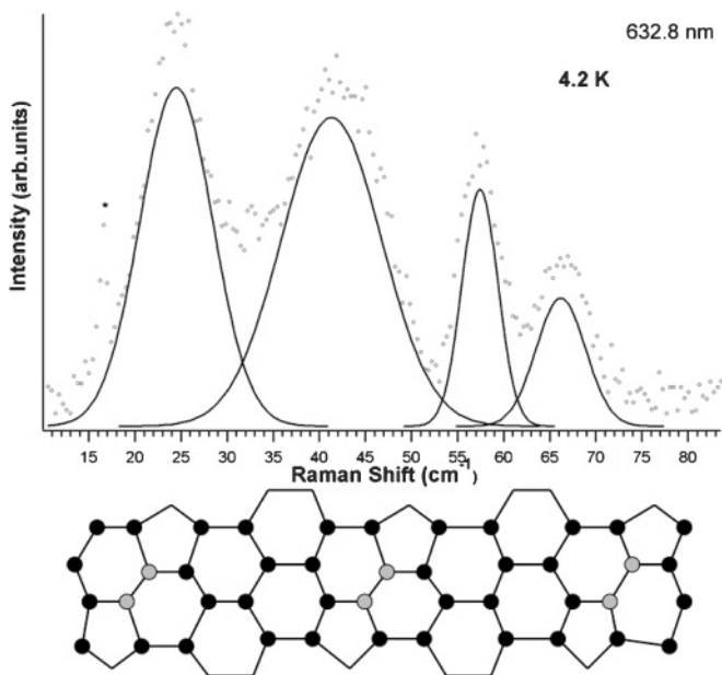
FIG. 4. (Top) Analysis of low-energy Raman rotational lines of Y_2C_2@C_{92} taken at 4.2 K indicating the even rotational levels of a free nonrigid C_2 rotor (asterisk indicates a plasma line). (Bottom) Motif of 6-6-5 cage intersections (identified in gray), which provide a repulsive rotational barrier to the Y_2C_2 complex.
