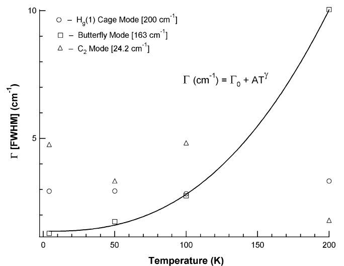
FIG. 3. The width (FWHM) of three Raman modes plotted against temperature. The butterfly mode ( 163.6\text{ cm}^{-1} ) undergoes a mode narrowing as the temperature decreases and can be modeled by a power law. Other modes show no significant change in width or intensity as the temperature is lowered.
