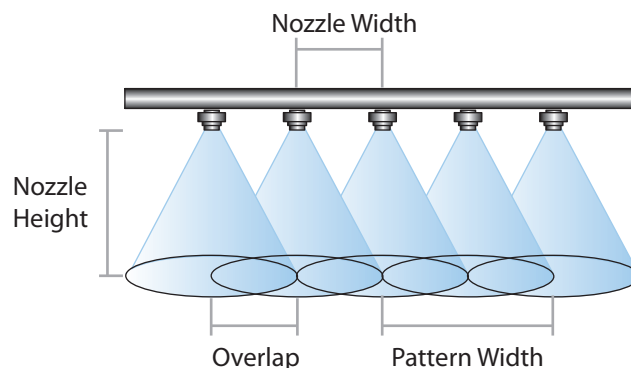
Figure 4. Nozzle overlap of 100 percent.
