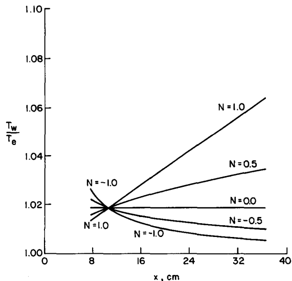
FIG. 2. Temperature distributions.
