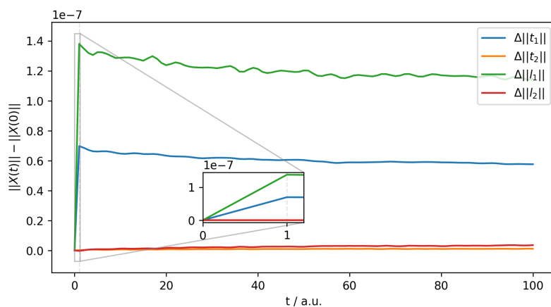
Figure C.1: Time-dependent change in the norm of the amplitude tensors relative to the ground-state amplitudes, using a PNO cut-off of 1 \times 10^{-9} . (Amplitudes have been back-transformed to the MO space for comparison to MO-basis amplitude norms. Field and step parameters remain unchanged, and the amplitude norm is taken at every 1 a.u.)
