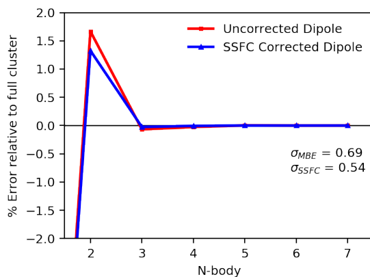
Figure A.16: MBE and SSFC of dipole moment for ( S )-methylthiirane in a six-water solvent shell. Computed with B3LYP/aDZ.
