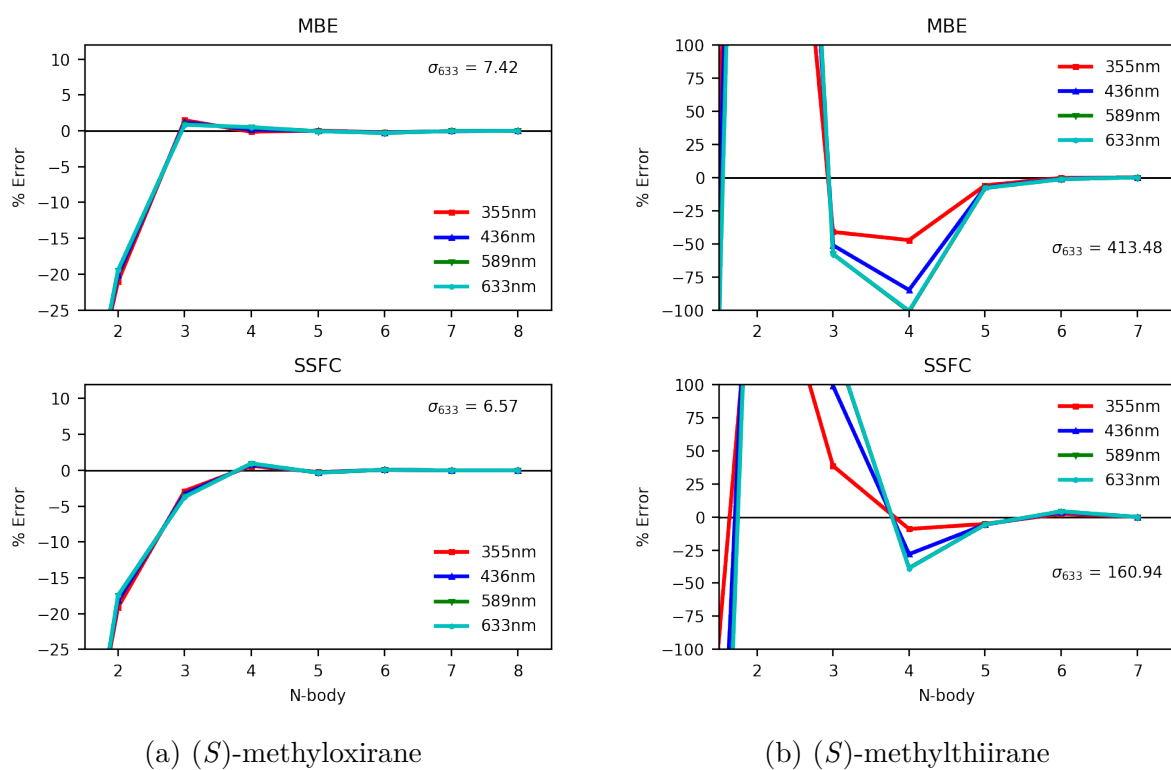
Figure 3.9: MBE and SSFC of solute-fragment-only specific rotation for (a) (S) -methyloxirane in a seven-water solvent shell and (b) (S) -methylthiirane in a six-water solvent shell. Computed with CAM-B3LYP/aDZ.
