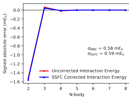
Figure A.3: MBE and SSFC of interaction energy for ( S )-methyloxirane in a seven-water solvent shell. Computed with B3LYP/aTZ.
