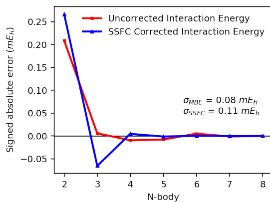
Figure A.26: MBE and SSFC of interaction energy for ( M )-dimethylallene in a seven-water solvent shell. Computed with CAM-B3LYP/aDZ.
