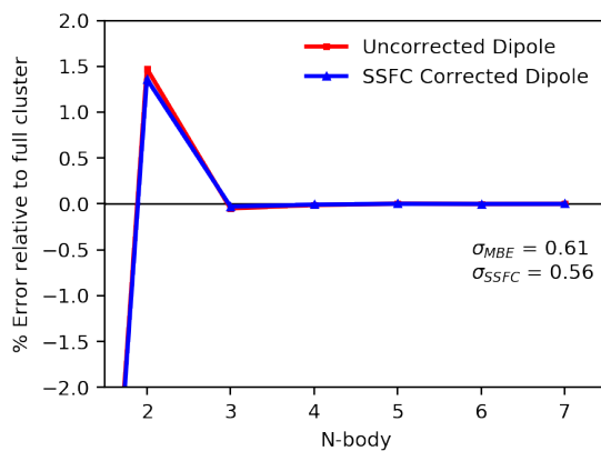
Figure A.18: MBE and SSFC of dipole moment for ( S )-methylthiirane in a six-water solvent shell. Computed with B3LYP/aTZ.
