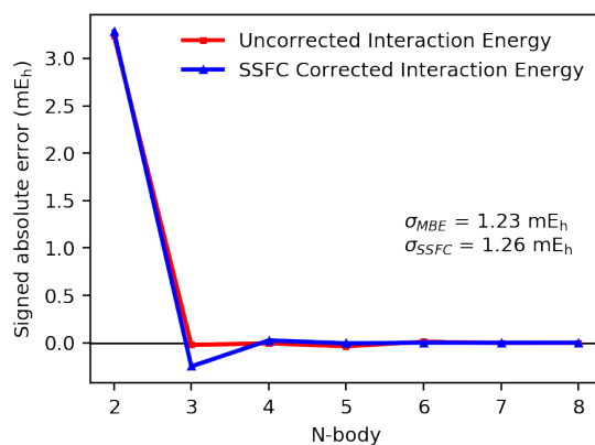
Figure A.8: MBE and SSFC of interaction energy for snapshot #2 of ( S )-methyloxirane in a seven-water solvent shell. Computed with CAM-B3LYP/aDZ.
