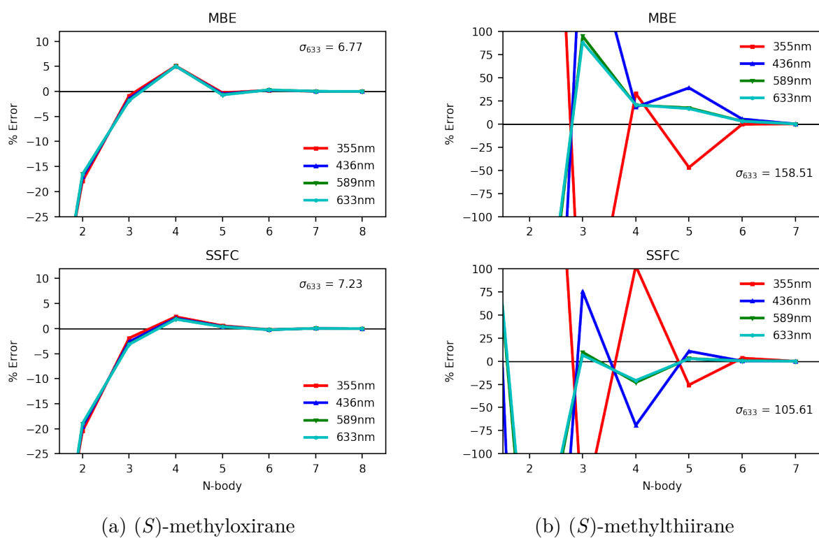
Figure 3.5: MBE and SSFC of specific rotation for (a) (S) -methyloxirane in a seven-water solvent shell and (b) (S) -methylthiirane in a six-water solvent shell. Computed with B3LYP/aTZ.
