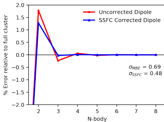
Figure A.6: MBE and SSFC of dipole moment for ( S )-methyloxirane in a seven-water solvent shell. Computed with CAM-B3LYP/aDZ.
