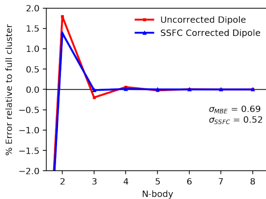
Figure A.2: MBE and SSFC of dipole moment for ( S )-methyloxirane in a seven-water solvent shell. Computed with B3LYP/aDZ.
