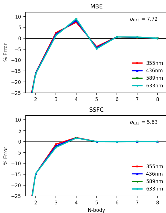
Figure A.7: MBE and SSFC of specific rotation for ( S )-methyloxirane in a seven-water solvent shell. Computed with CAM-B3LYP/aDZ.
