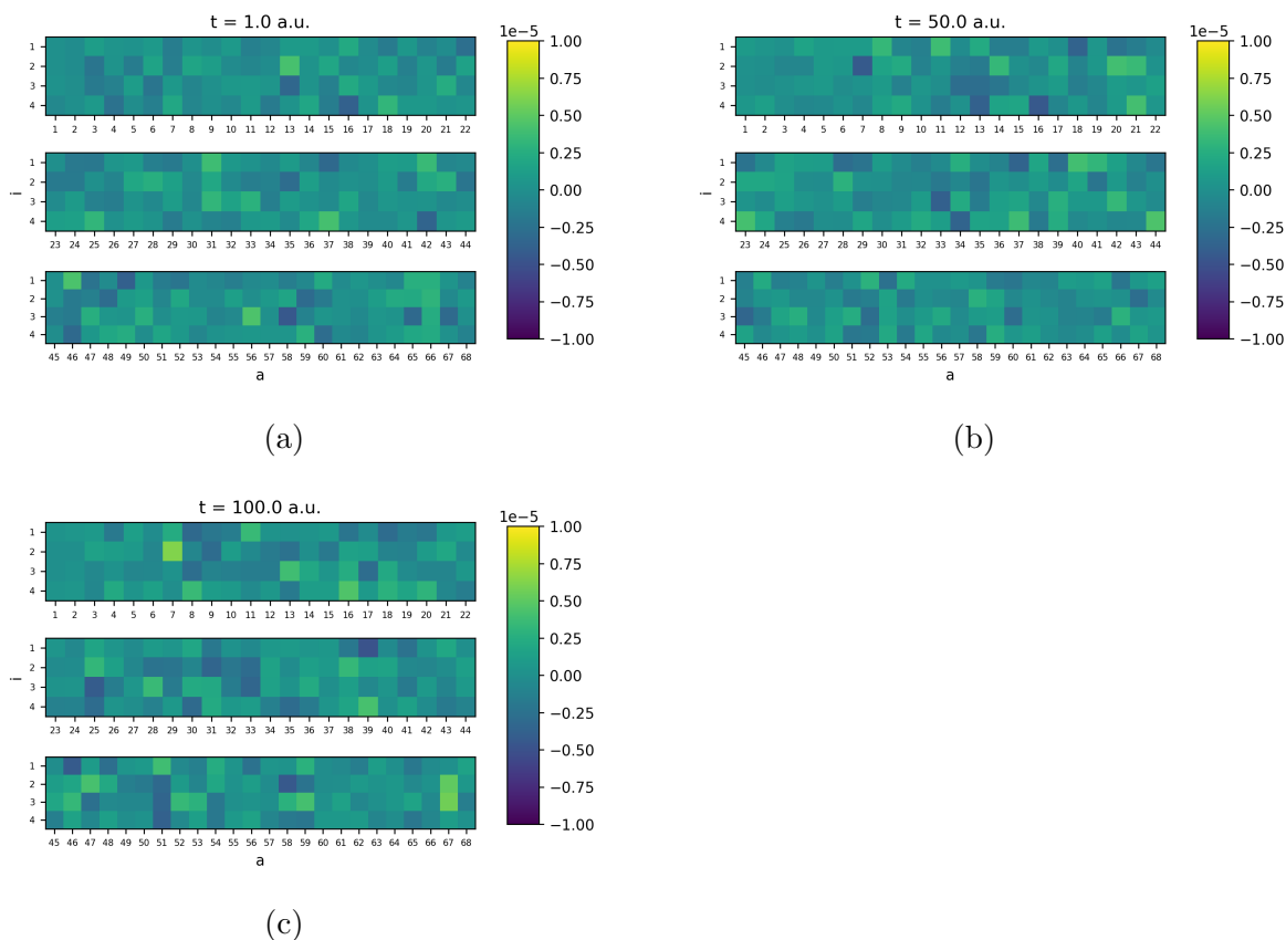
Figure 5.7: PNO-basis t_1 amplitude deviations from t = 0 after (a) 1 a.u., (b) 50 a.u., and (c) 100 a.u. of time propagation. Each row contains the same four occupied orbital indices and a subset of virtual indices as indicated by the x-axis labels.
