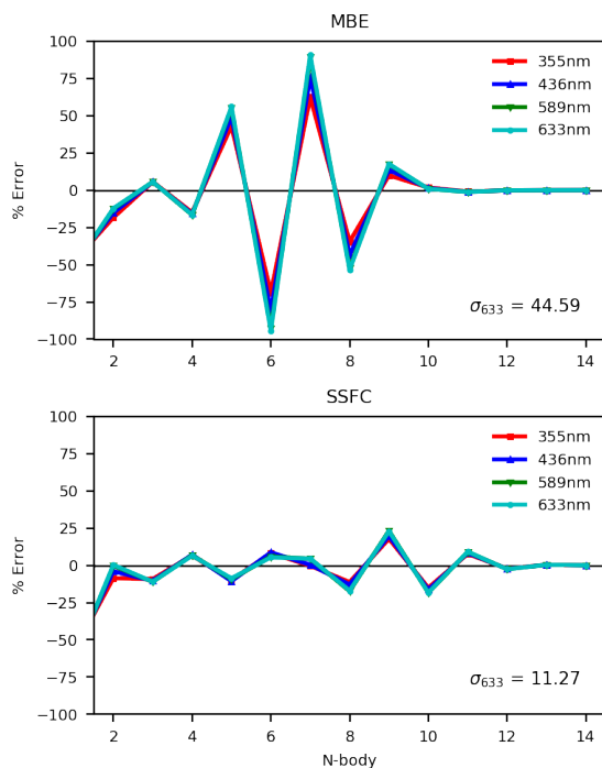
Figure 3.8: MBE and SSFC of specific rotation for ( S )-methyloxirane in a 13-water solvent shell. Computed with CAM-B3LYP/aDZ.
