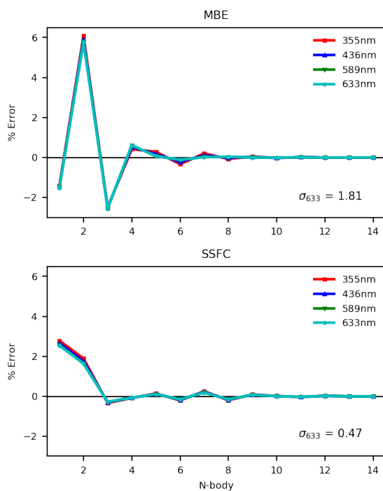
Figure 3.3: MBE and SSFC of dynamic polarizabilities for ( S )-methyloxirane in a 13-water solvent shell. Computed with CAM-B3LYP/aDZ.
