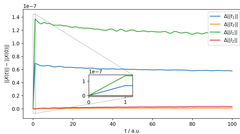
Figure C.2: Time-dependent change in the norm of the amplitude tensors relative to the ground-state amplitudes, using a PAO cut-off of 1 \times 10^{-3} . (Amplitudes have been back-transformed to the MO space for comparison to MO-basis amplitude norms. Field and step parameters remain unchanged, and the amplitude norm is taken at every 1 a.u.)
