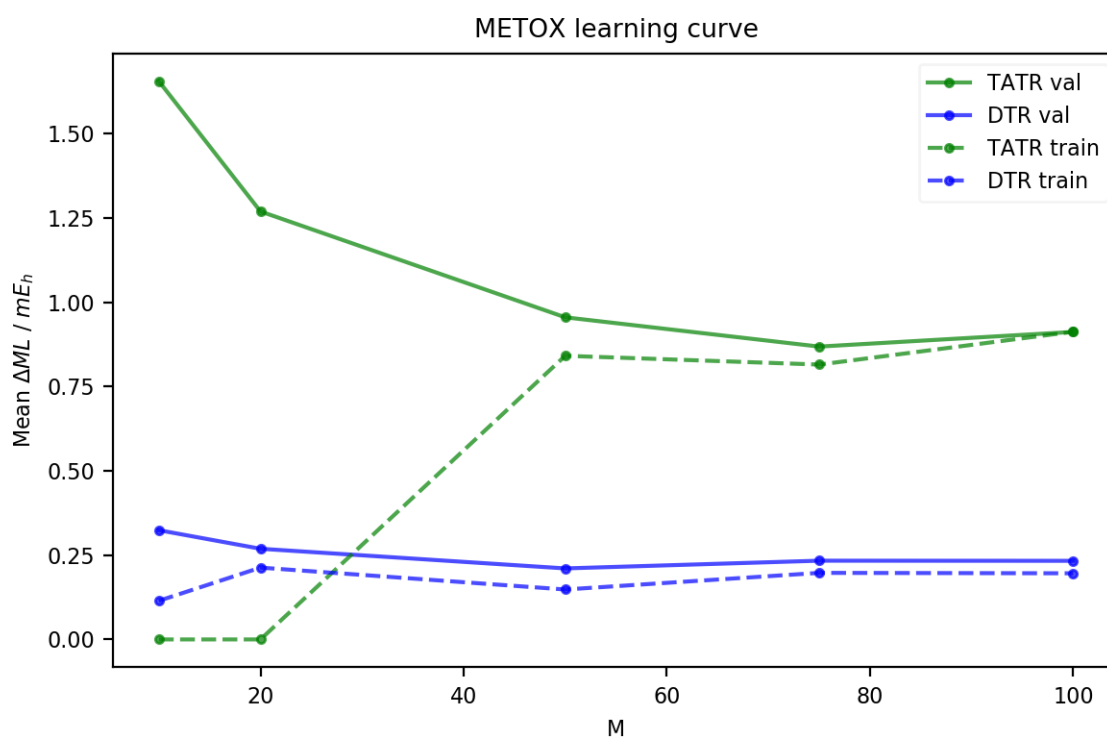
Figure B.11: DTR and TATR learning curves for ( S )-methyloxirane correlation energy.
