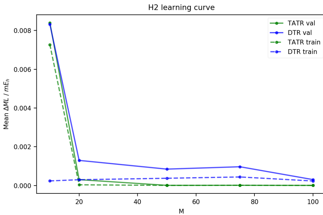
Figure B.4: DTR and TATR learning curves for H_2 correlation energy.
