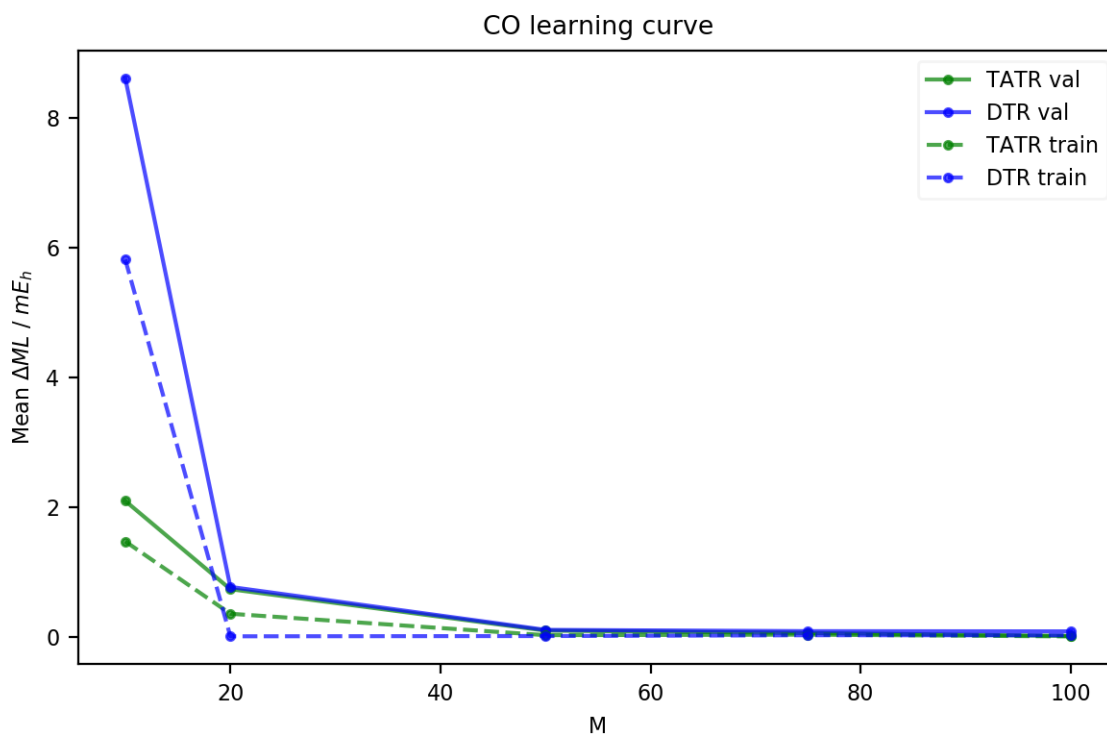
Figure B.6: DTR and TATR learning curves for CO correlation energy.
