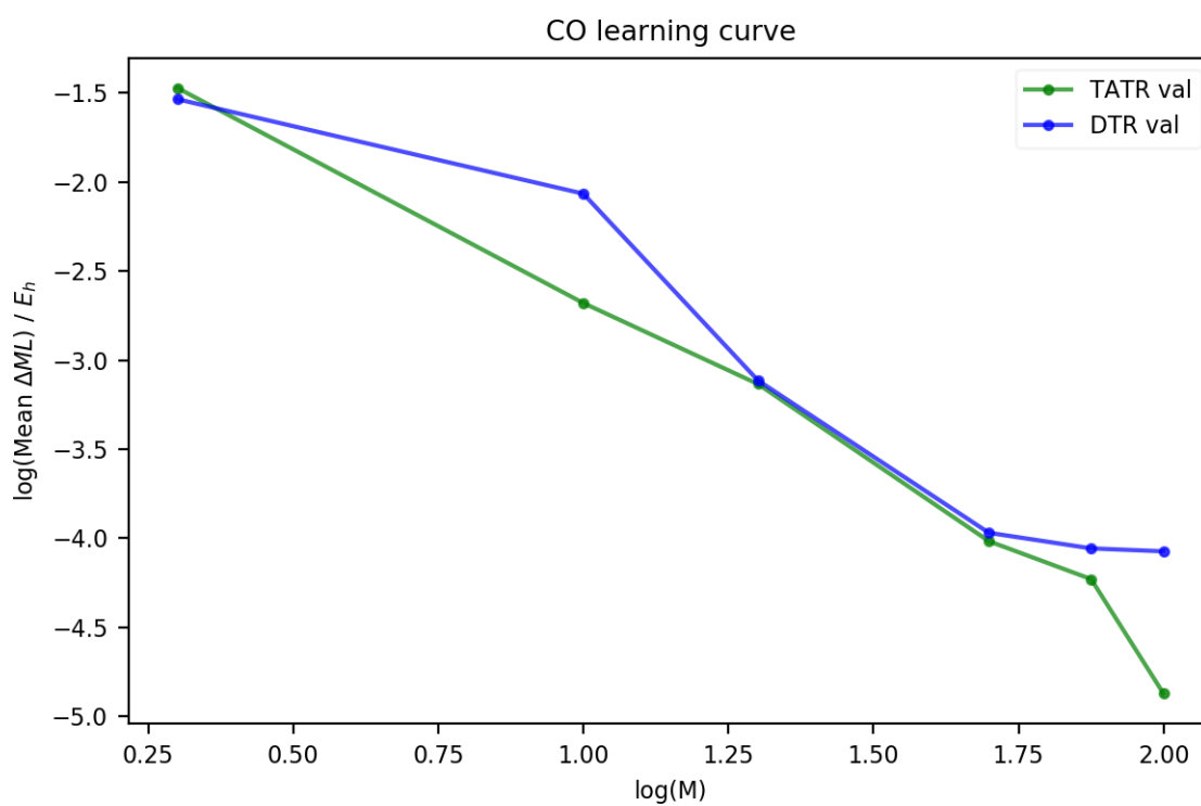
Figure B.22: DTR and TATR validation curves for CO correlation energy.
