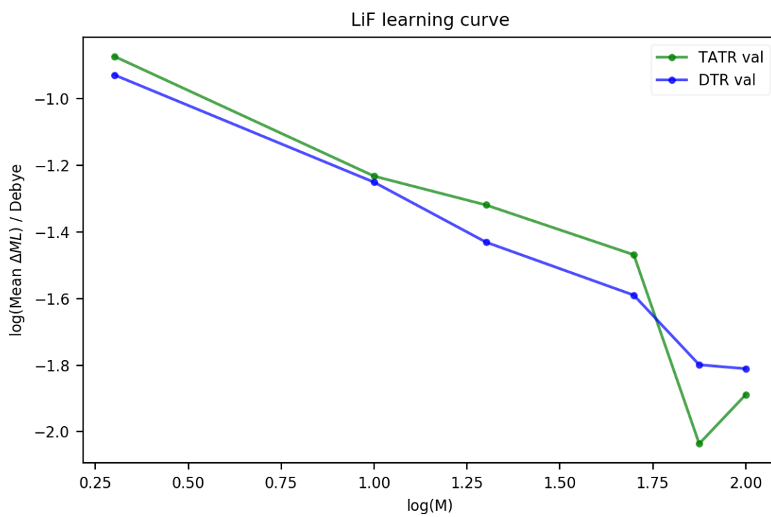
Figure B.31: DTR and TATR validation curves for LiF correlated dipole.
