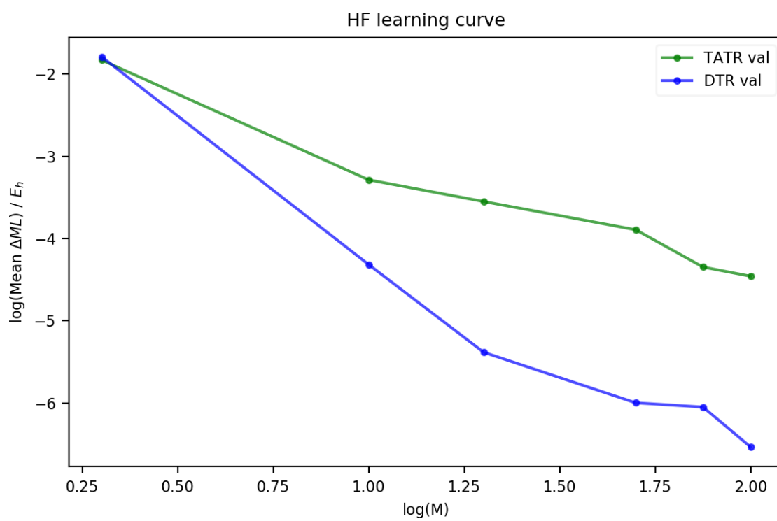
Figure B.21: DTR and TATR validation curves for HF correlation energy.
