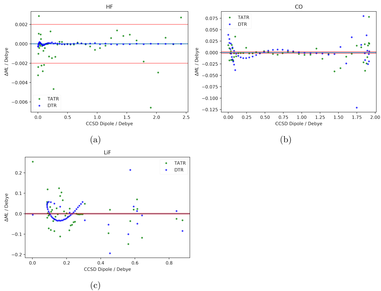
Figure B.2: DTR vs TATR errors in Debye for diatomic datasets: (a) HF, (b) CO, and (c) LiF. Red lines indicate 2 milliDebye.
