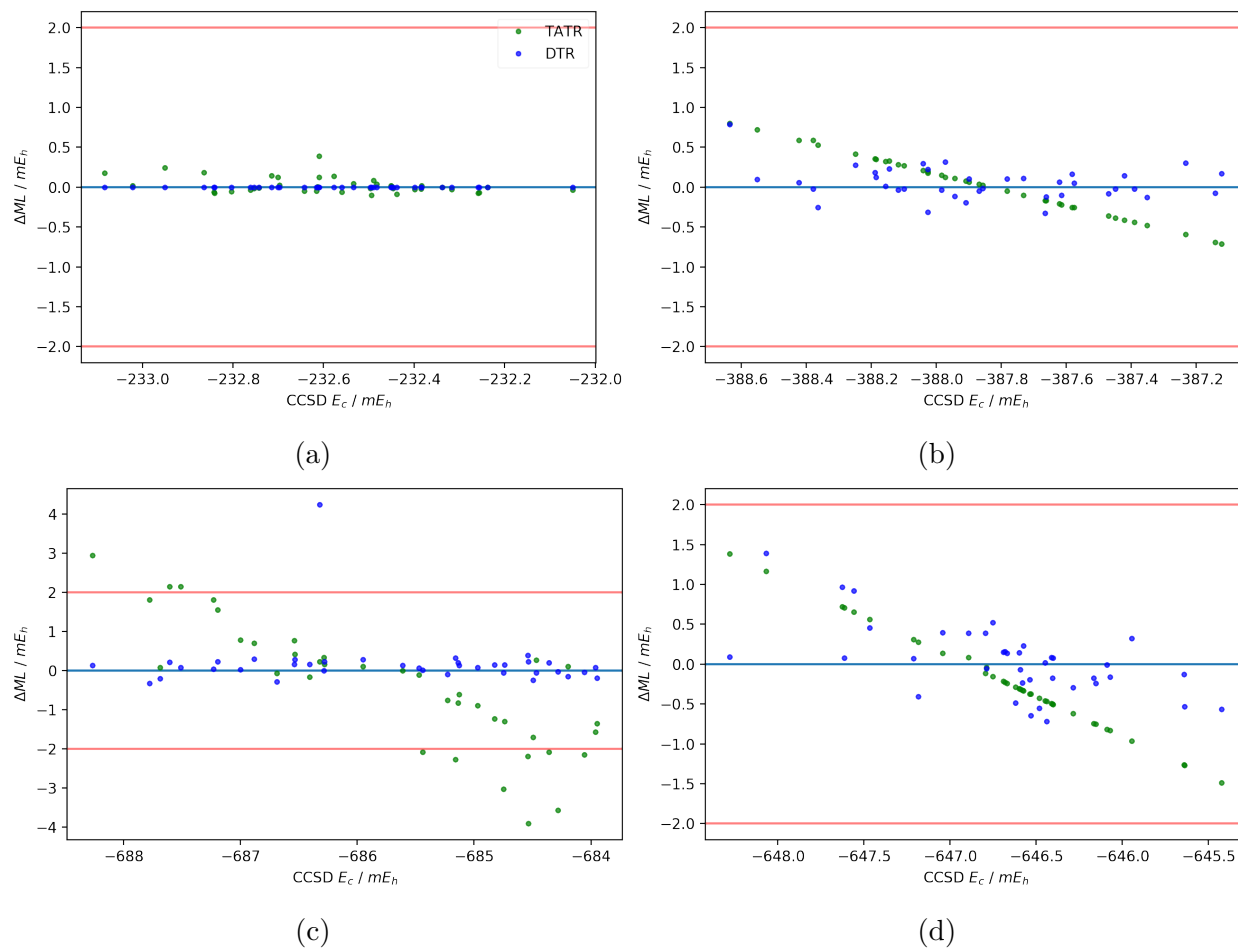
Figure 4.2: DTR vs TATR errors in mE_h for small molecule datasets: (a) H_2O , (b) CH_3OH , (c) ( S )-methyloxirane, and (d) ( R )-methylthiirane. Red lines indicate 2 mE_h .
