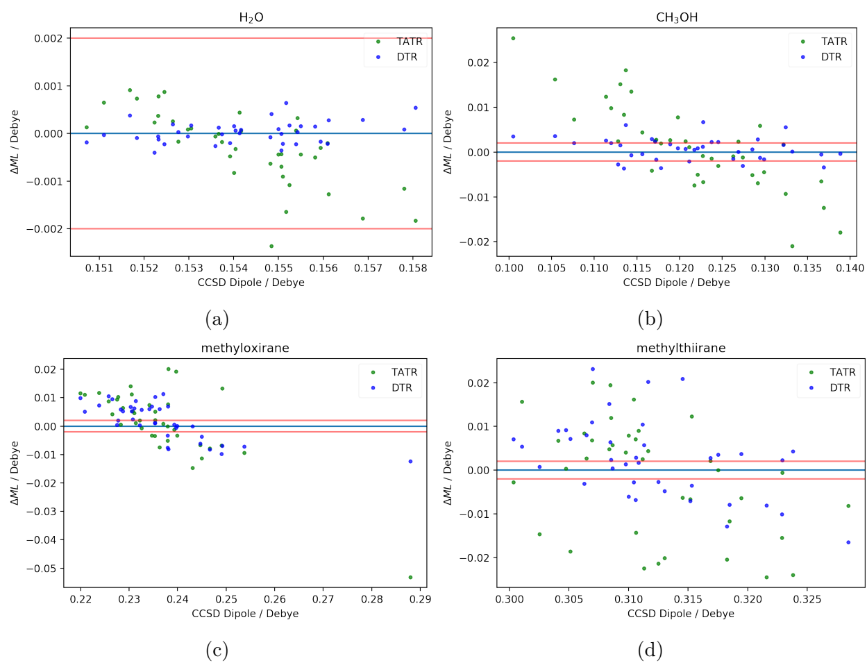
Figure B.3: DTR vs TATR errors in Debye for small molecule datasets: (a) \text{H}_2\text{O} , (b) \text{CH}_3\text{OH} , (c) ( S )-methyloxirane, and (d) ( R )-methylthiirane. Red lines indicate 2 milliDebye.
