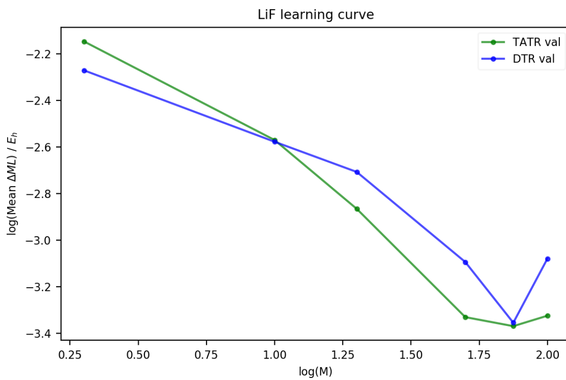
Figure B.23: DTR and TATR validation curves for LiF correlation energy.
