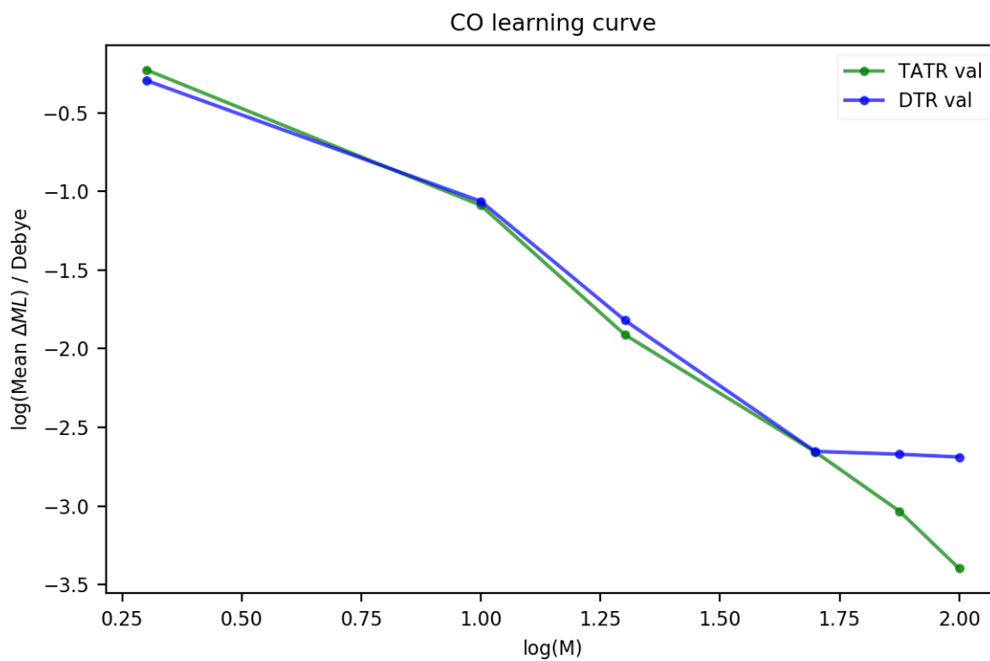
Figure B.30: DTR and TATR validation curves for CO correlated dipole.
