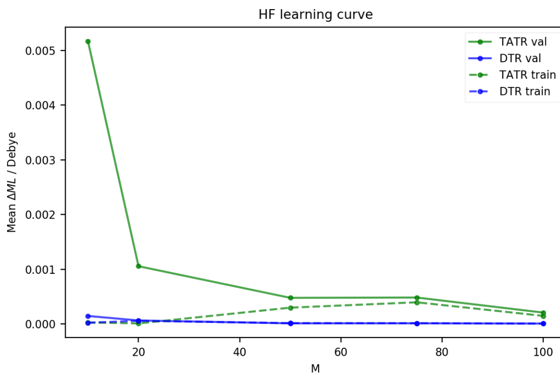
Figure B.13: DTR and TATR learning curves for HF correlated dipole.
