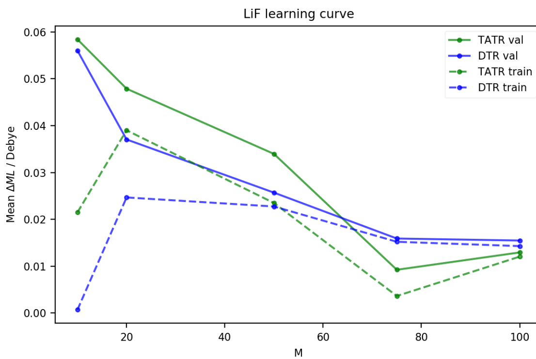
Figure B.15: DTR and TATR learning curves for LiF correlated dipole.
