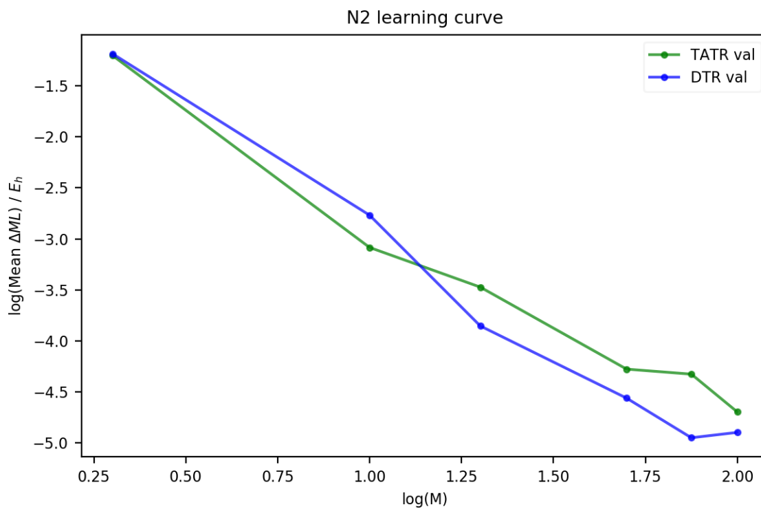
Figure B.24: DTR and TATR validation curves for N 2 correlation energy.
