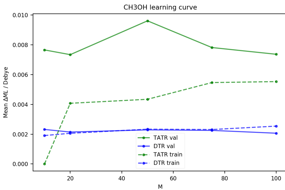
Figure B.17: DTR and TATR learning curves for CH 3 OH correlated dipole.
