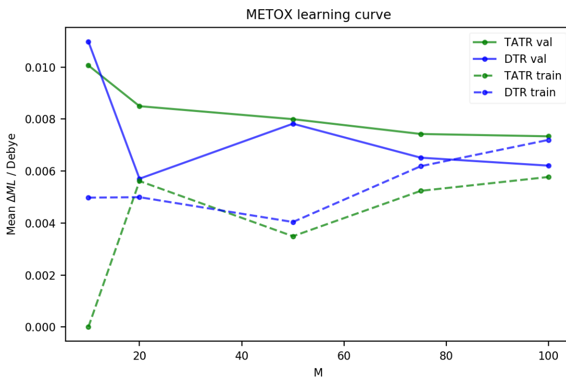
Figure B.18: DTR and TATR learning curves for ( S )-methyloxirane correlated dipole.
