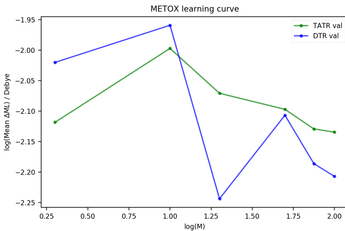
Figure B.34: DTR and TATR validation curves for ( S )-methyloxirane correlated dipole.
