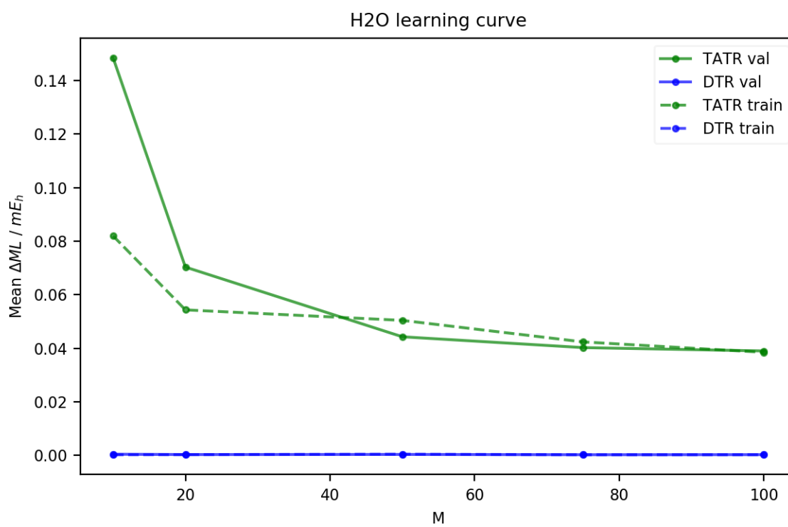
Figure B.9: DTR and TATR learning curves for H 2 O correlation energy.
