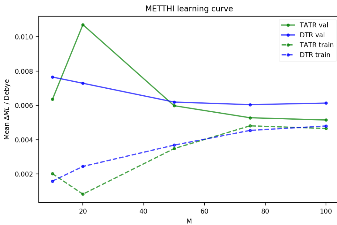
Figure B.19: DTR and TATR learning curves for ( R )-methylthiirane correlated dipole.
