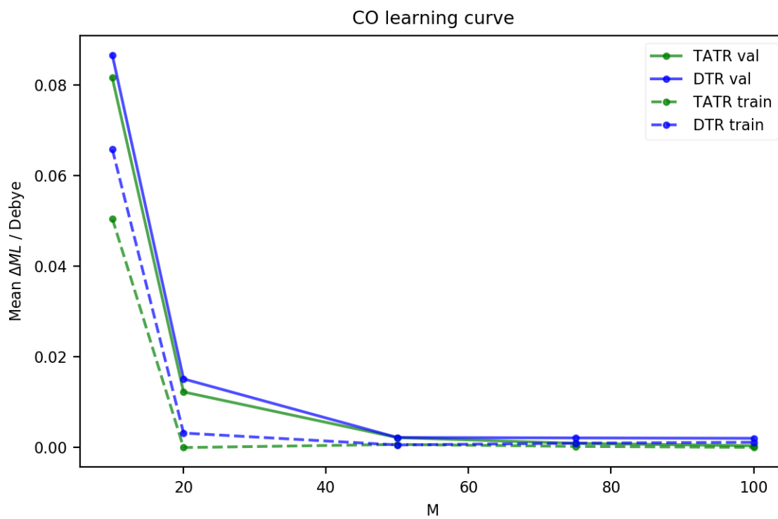
Figure B.14: DTR and TATR learning curves for CO correlated dipole.
