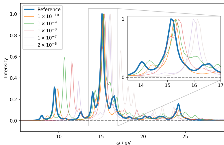
Figure 5.1: Reference and PNO absorption spectra of (H_2)_4 for five cutoffs: [ 1 \times 10^{-10} , 1 \times 10^{-9} , 1 \times 10^{-8} , 1 \times 10^{-7} , 2 \times 10^{-6} ] corresponding to [93%, 82%, 63%, 44%, 24%] of the MO virtual space, respectively.
