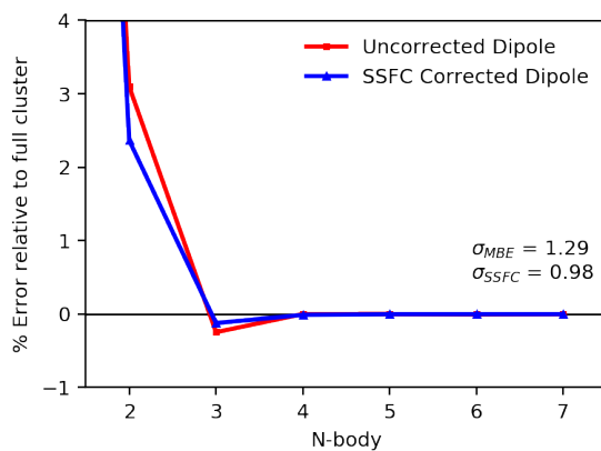
Figure A.22: MBE and SSFC of dipole moment for snapshot #2 of ( S )-methylthiirane in a six-water solvent shell. Computed with CAM-B3LYP/aDZ.
