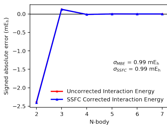
Figure A.17: MBE and SSFC of interaction energy for ( S )-methylthiirane in a six-water solvent shell. Computed with B3LYP/aTZ.
