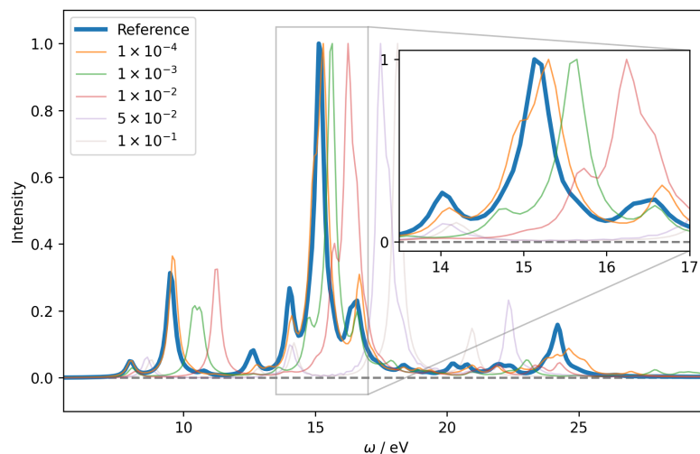
Figure 5.2: Reference and PAO absorption spectra of (H_2)_4 for five cutoffs: [1 \times 10^{-4}, 1 \times 10^{-3}, 1 \times 10^{-2}, 5 \times 10^{-2}, 1 \times 10^{-1}] corresponding to [95\%, 86\%, 63\%, 46\%, 23\%] of the MO virtual space, respectively.
