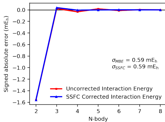
Figure A.1: MBE and SSFC of interaction energy for ( S )-methyloxirane in a seven-water solvent shell. Computed with B3LYP/aDZ.
