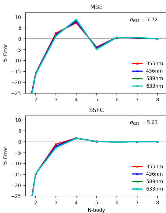
Figure A.13: MBE and SSFC of specific rotation of ( S )-methyloxirane in a seven-water solvent shell using “tight” convergence criteria and “fine” grids. Computed with CAM-B3LYP/aDZ.
