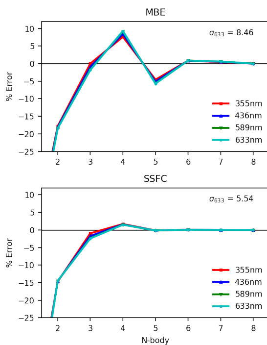
Figure A.14: MBE and SSFC of specific rotation of ( S )-methyloxirane in a seven-water solvent shell and unpruned “fine” grids. Computed with CAM-B3LYP/aDZ.
