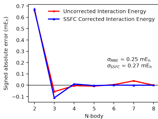
Figure A.24: MBE and SSFC of interaction energy for ( M )-dimethylallene in a seven-water solvent shell. Computed with B3LYP/aDZ.
