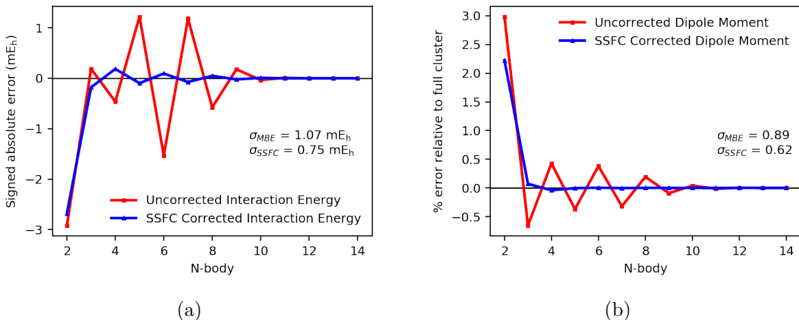
Figure 3.1: MBE and SSFC of (a) interaction energies and (b) dipole moments for ( S )-methyloxirane in a 13-water solvent shell.
