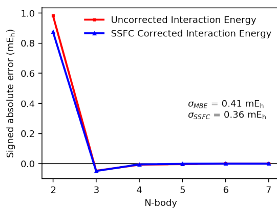
Figure A.21: MBE and SSFC of interaction energy for snapshot #2 of ( S )-methylthiirane in a six-water solvent shell. Computed with CAM-B3LYP/aDZ.
