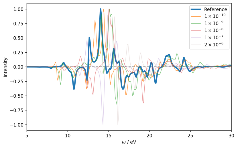
Figure 5.3: Reference and PNO ECD spectra of (H_2)_4 for five cutoffs: [1 \times 10^{-10}, 1 \times 10^{-9}, 1 \times 10^{-8}, 1 \times 10^{-7}, 2 \times 10^{-6}] corresponding to [93%, 82%, 63%, 44%, 24%] of the MO virtual space, respectively.
