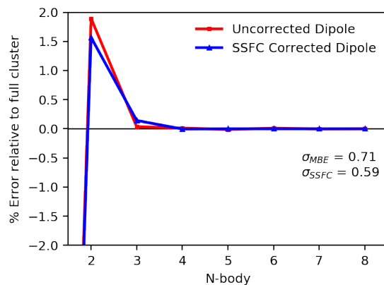
Figure A.9: MBE and SSFC of dipole moment for snapshot #2 of ( S )-methyloxirane in a seven-water solvent shell. Computed with CAM-B3LYP/aDZ.
