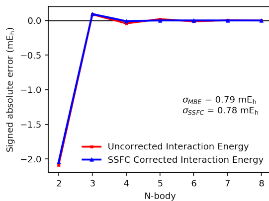
Figure A.5: MBE and SSFC of interaction energy for ( S )-methyloxirane in a seven-water solvent shell. Computed with CAM-B3LYP/aDZ.
