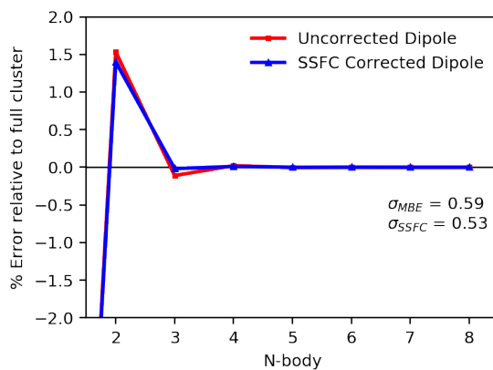
Figure A.4: MBE and SSFC of dipole moment for ( S )-methyloxirane in a seven-water solvent shell. Computed with B3LYP/aTZ.
