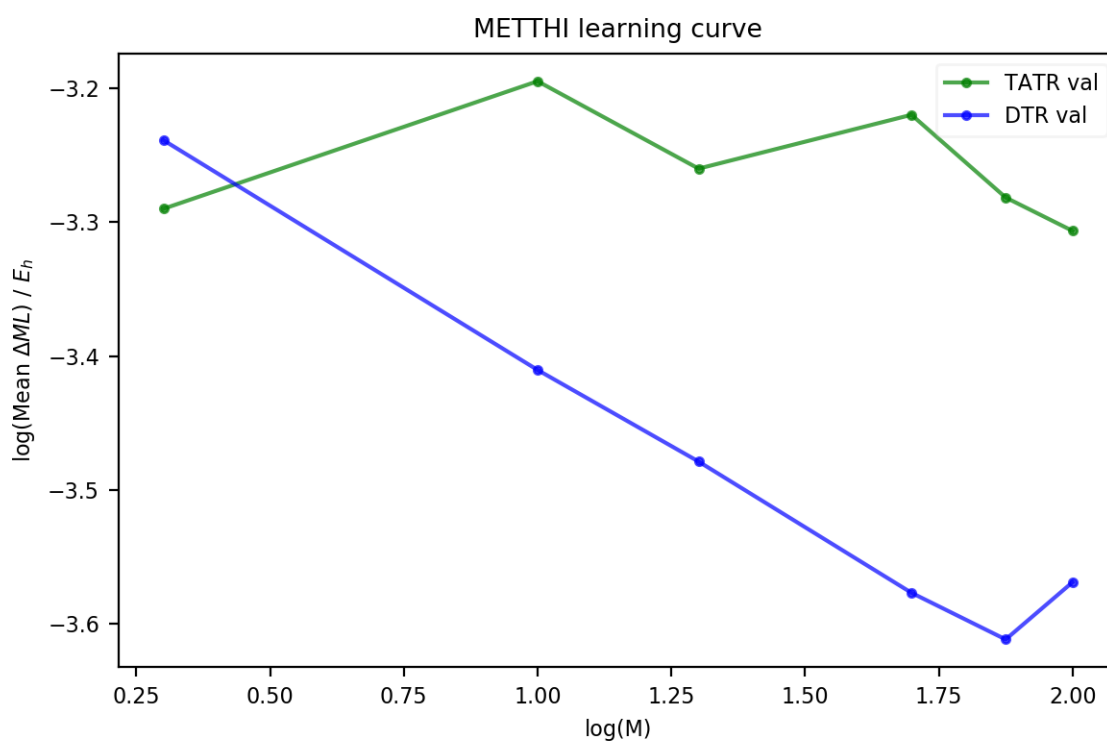
Figure B.28: DTR and TATR validation curves for ( R )-methylthiirane correlation energy.
