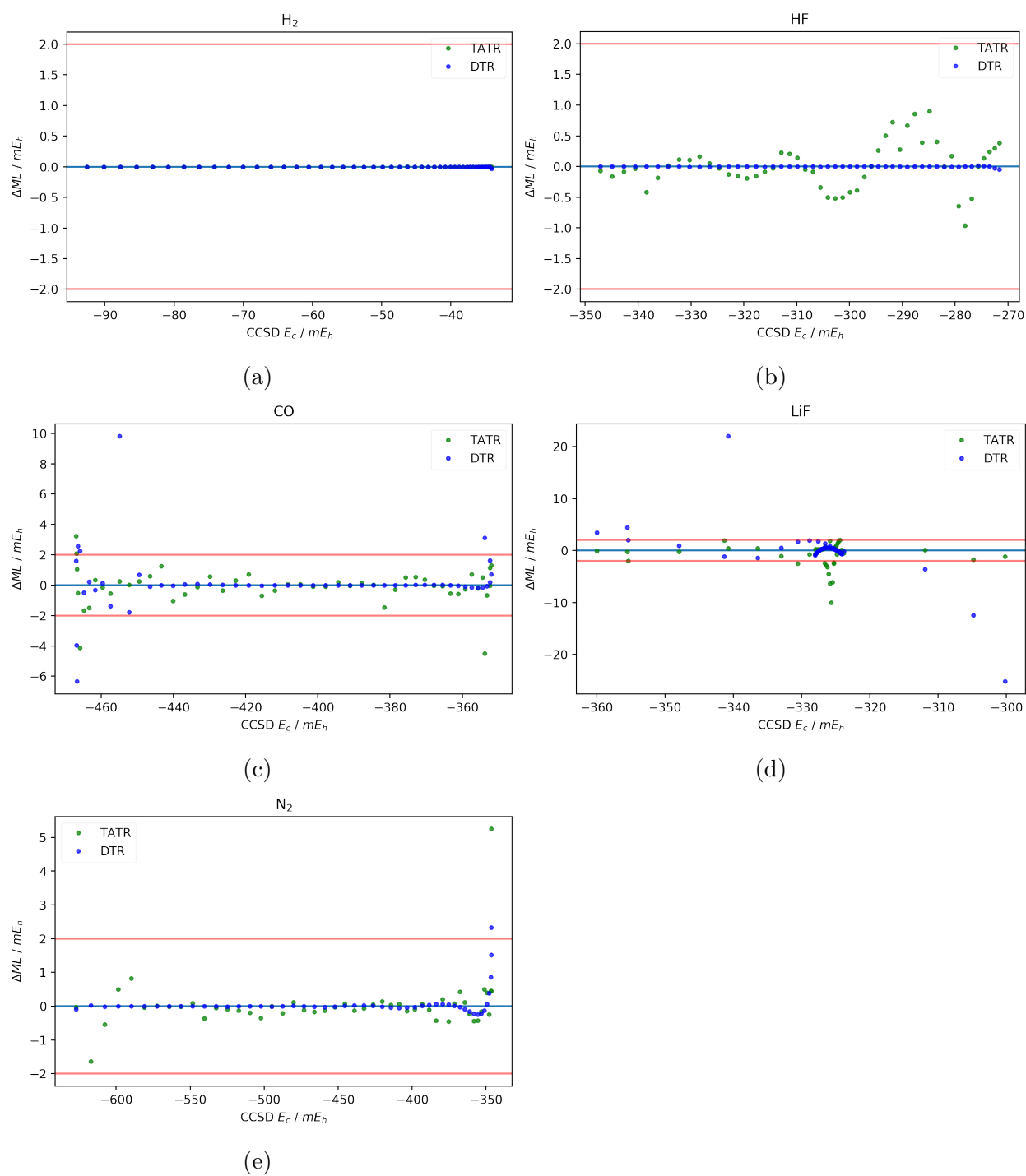
Figure B.1: DTR vs TATR errors in mE_h for diatomic datasets: (a) H_2 , (b) HF , (c) CO , (d) LiF , and (e) N_2 . Red lines indicate 2 mE_h .
