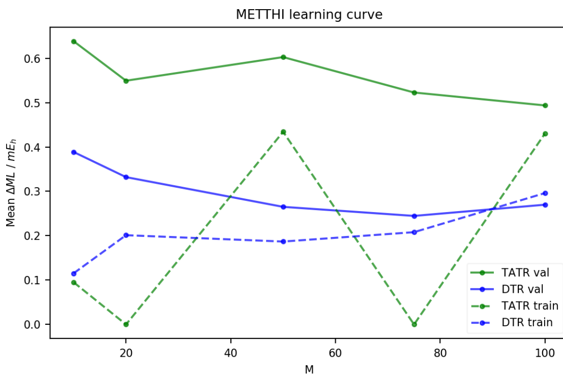
Figure B.12: DTR and TATR learning curves for ( R )-methylthiirane correlation energy.
