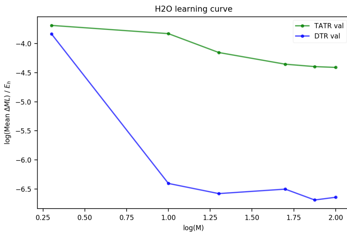
Figure B.25: DTR and TATR validation curves for H 2 O correlation energy.
