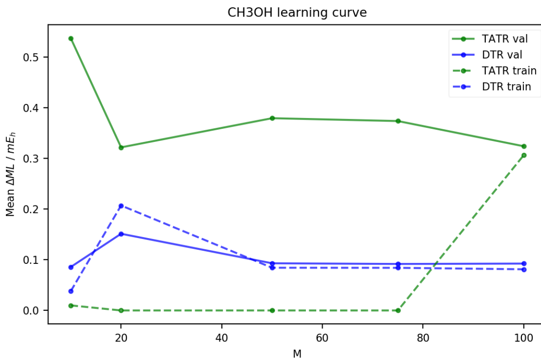
Figure B.10: DTR and TATR learning curves for CH 3 OH correlation energy.
