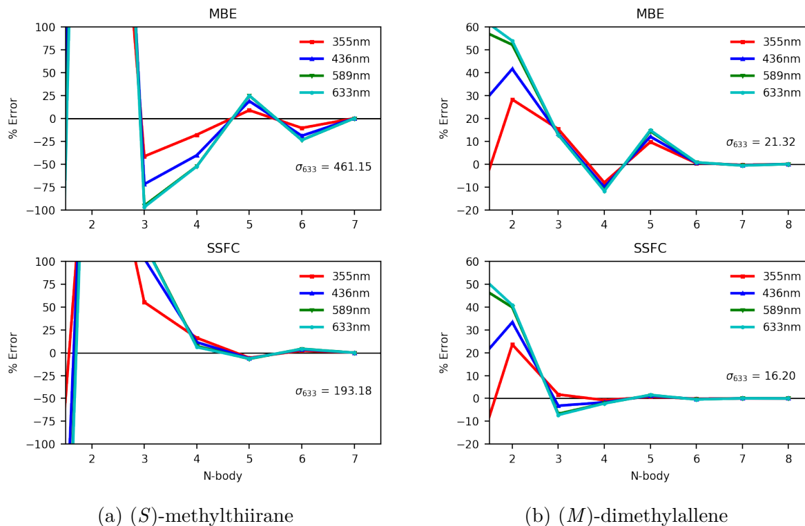
Figure 3.6: MBE and SSFC of specific rotation for (a) ( S )-methylthiirane in a six-water solvent shell and (b) ( M )-dimethylallene in a seven-water solvent shell. Computed with CAM-B3LYP/aDZ.
