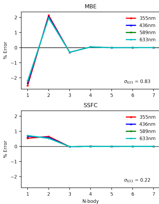
Figure A.23: MBE and SSFC of dynamic polarizabilities for snapshot #2 of ( S )-methylthiirane in a six-water solvent shell. Computed with CAM-B3LYP/aDZ.
