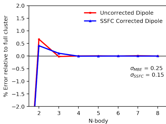
Figure A.27: MBE and SSFC of dipole moment for ( M )-dimethylallene in a seven-water solvent shell. Computed with CAM-B3LYP/aDZ.
