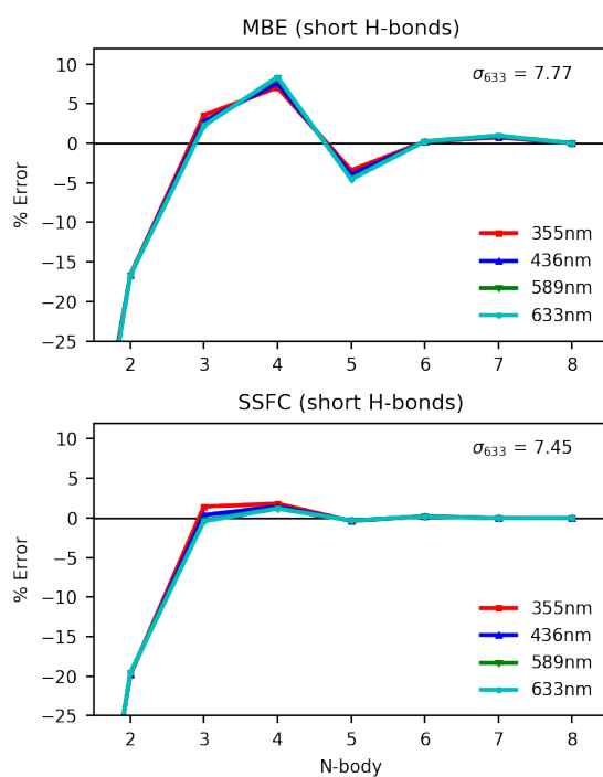
Figure A.12: MBE and SSFC of specific rotation of ( S )-methyloxirane in a seven-water solvent shell and two manually reduced H-bonds. Computed with CAM-B3LYP/aDZ.
