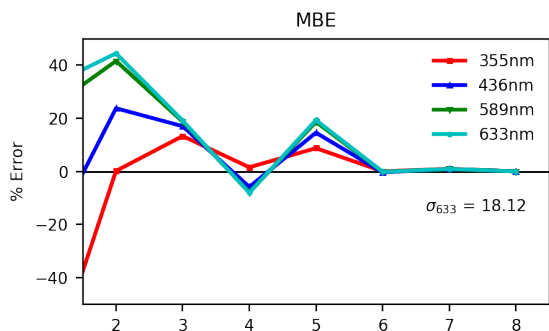
(a) ( S )-methyloxirane
