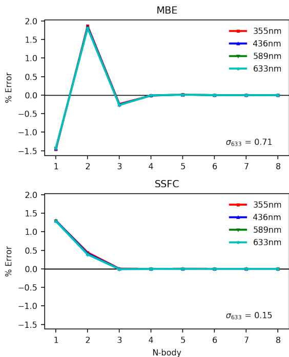
(c) ( M )-dimethylallene
