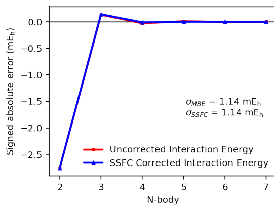
Figure A.19: MBE and SSFC of interaction energy for ( S )-methylthiirane in a six-water solvent shell. Computed with CAM-B3LYP/aDZ.
