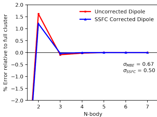
Figure A.20: MBE and SSFC of dipole moment for ( S )-methylthiirane in a six-water solvent shell. Computed with CAM-B3LYP/aDZ.
