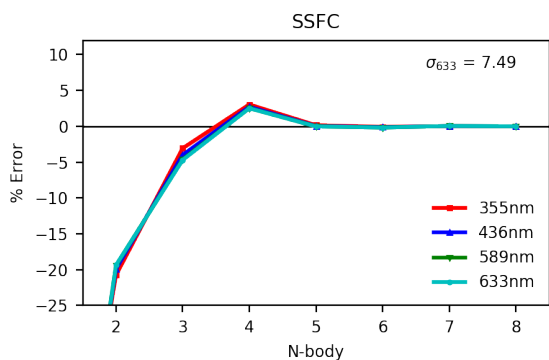
(a) ( S )-methyloxirane
