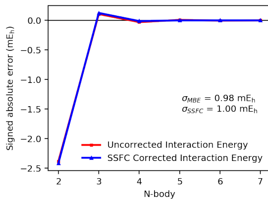
Figure A.15: MBE and SSFC of interaction energy for ( S )-methylthiirane in a six-water solvent shell. Computed with B3LYP/aDZ.
