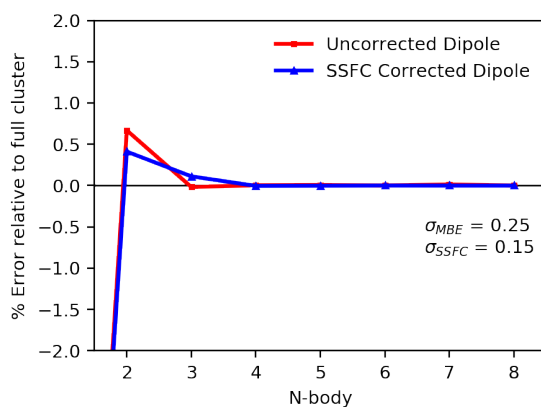
Figure A.25: MBE and SSFC of dipole moment for ( M )-dimethylallene in a seven-water solvent shell. Computed with B3LYP/aDZ.
