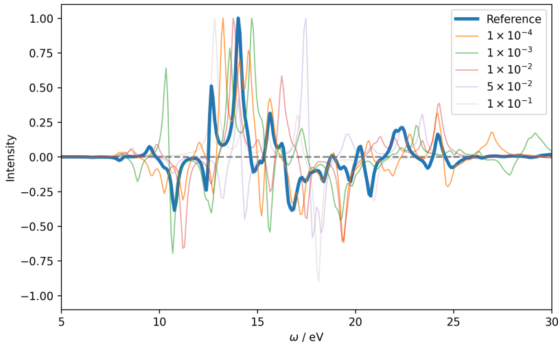
Figure 5.4: Reference and PAO ECD spectra of (H_2)_4 for five cutoffs: [1 \times 10^{-4}, 1 \times 10^{-3}, 1 \times 10^{-2}, 5 \times 10^{-2}, 1 \times 10^{-1}] corresponding to [95\%, 86\%, 63\%, 46\%, 23\%] of the MO virtual space, respectively.
