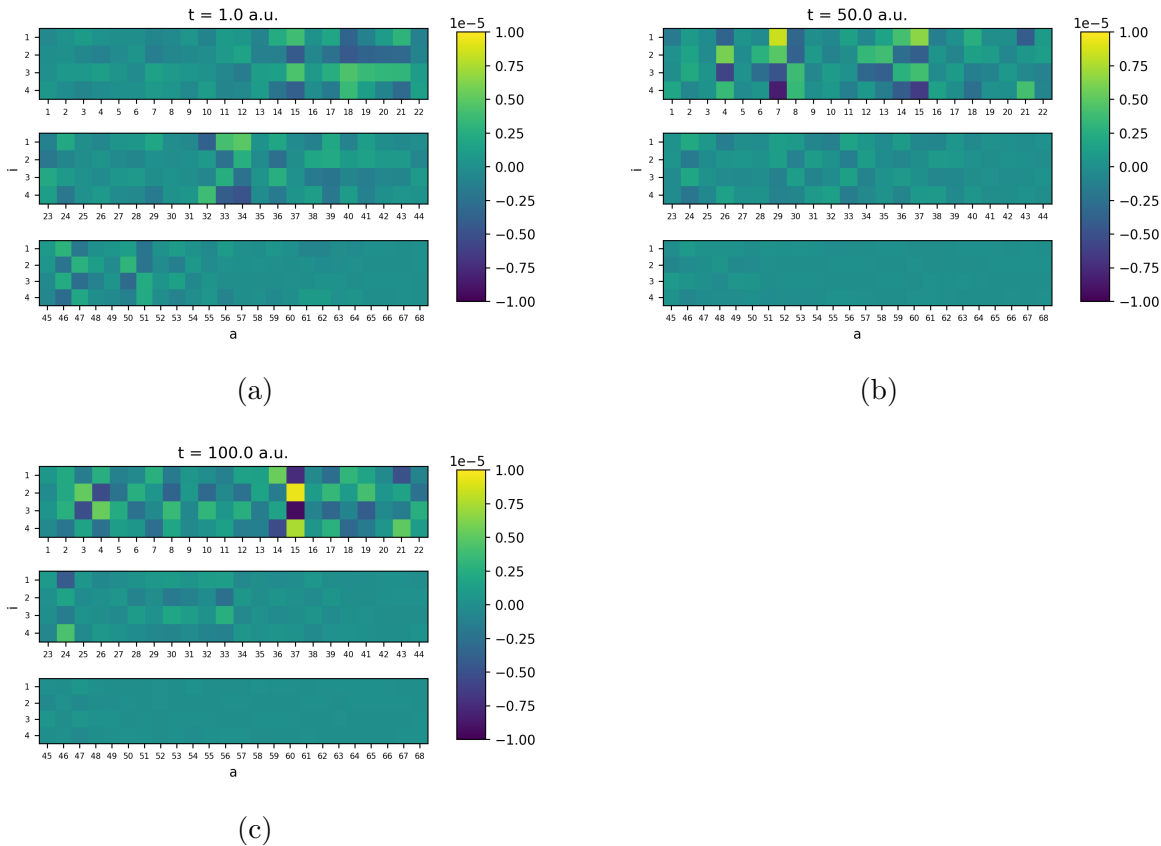
Figure 5.6: MO-basis t_1 amplitude deviations from t = 0 after (a) 1 a.u., (b) 50 a.u., and (c) 100 a.u. of time propagation. Each row contains the same four occupied orbital indices and a subset of virtual indices as indicated by the x-axis labels.
