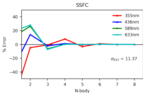
(c) ( M )-dimethylallene
