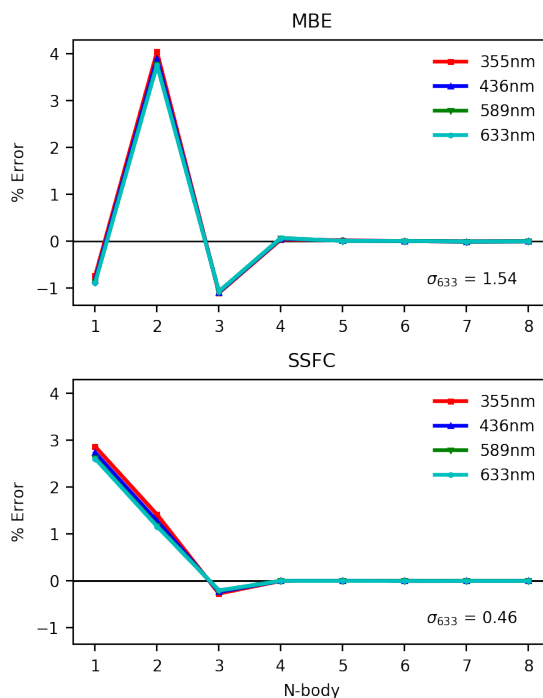
Figure A.10: ( S )-methyloxirane
