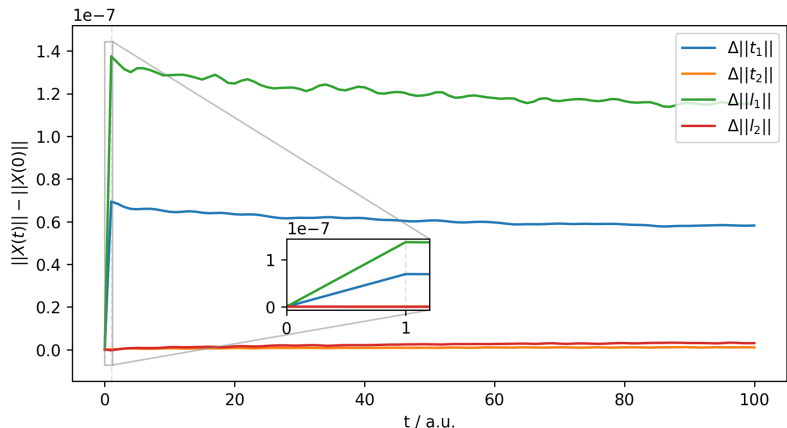
Figure 5.5: Time-dependent change in the norm of the amplitude tensors relative to the ground-state amplitudes. (Field and step parameters remain unchanged, and the amplitude norm is taken at every 1 a.u.)
