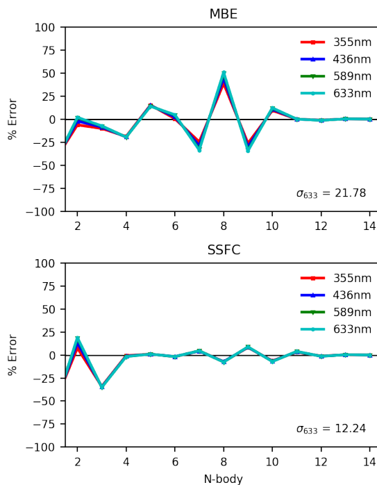
Figure 3.10: MBE and SSFC of solute-fragment-only specific rotation for ( S )-methyloxirane in a 13-water solvent shell. Computed with CAM-B3LYP/aDZ.
