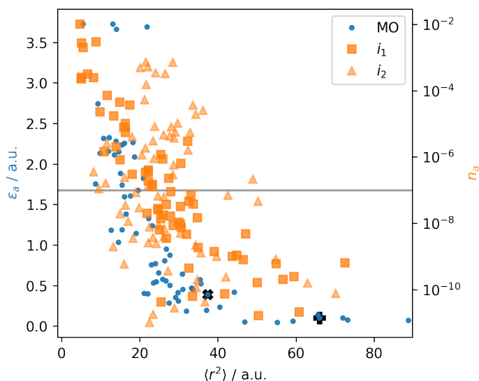
Figure 5.8: Virtual MO energy \epsilon_a and the occupation number n_a (plotted on a log scale) for unique PNO spaces i_1 and i_2 versus orbital extent. Virtual MOs 7 and 15 are denoted by a solid + and \times , respectively. The horizontal line denotes a PNO cutoff of 1 \times 10^{-7} .
