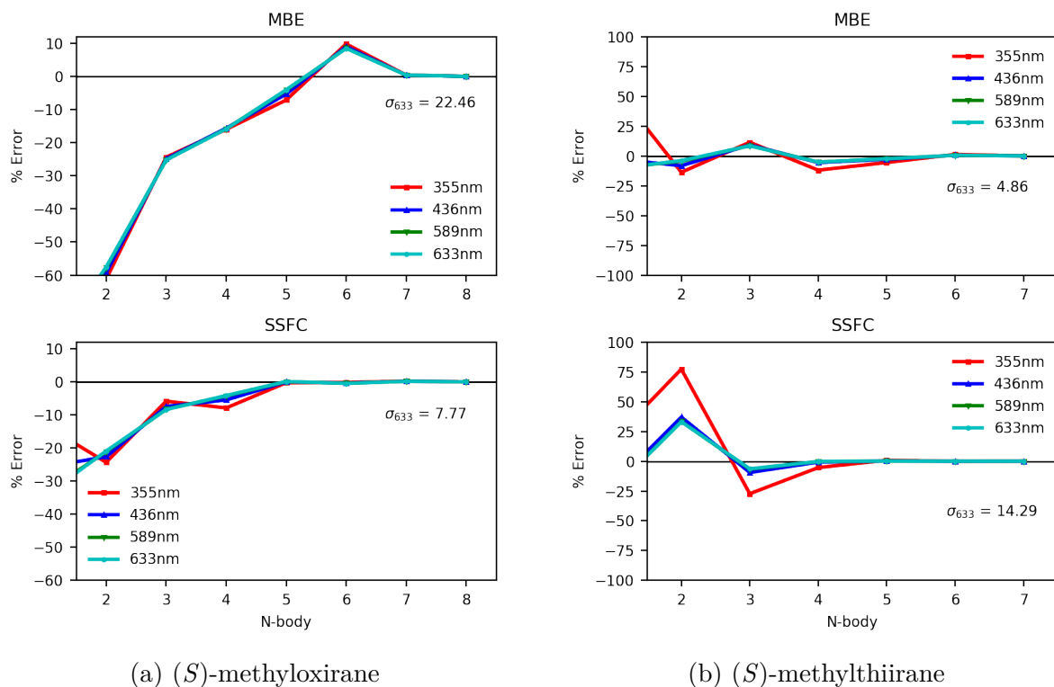
Figure 3.7: MBE and SSFC of specific rotation for additional snapshots of (a) (S) -methyloxirane in a seven-water solvent shell and (b) (S) -methylthiirane in a six-water solvent shell. Computed with CAM-B3LYP/aDZ.
