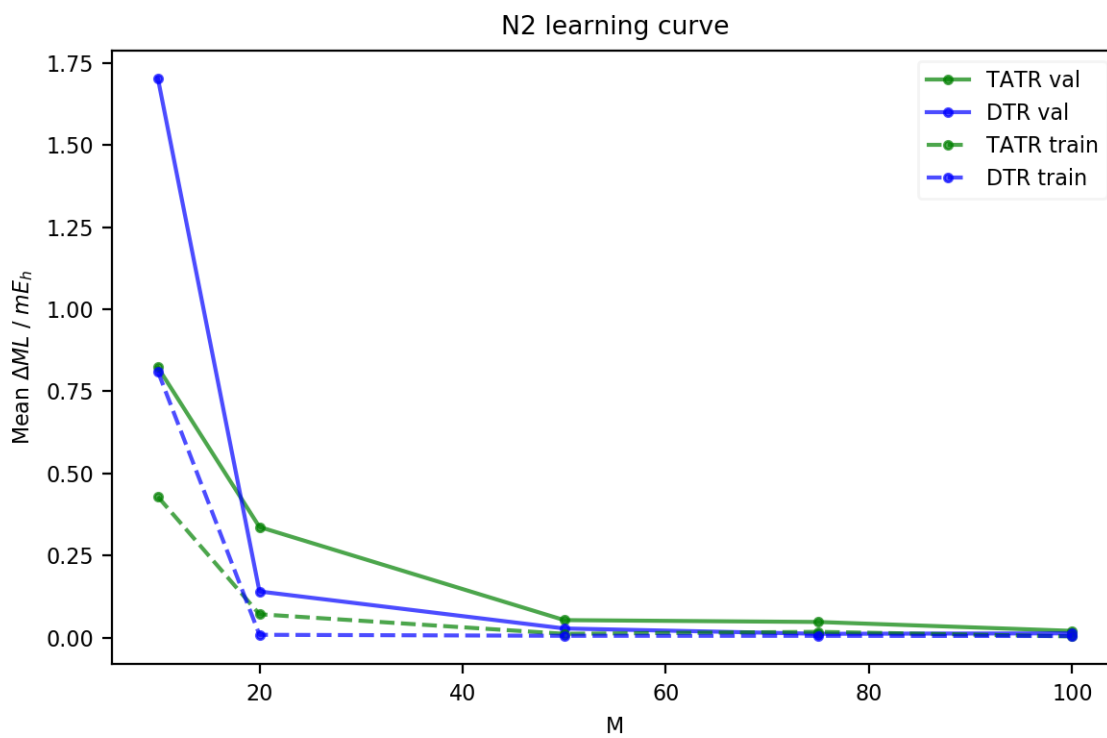
Figure B.8: DTR and TATR learning curves for N 2 correlation energy.
