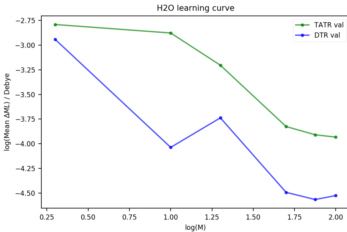
Figure B.32: DTR and TATR validation curves for H 2 O correlated dipole.
