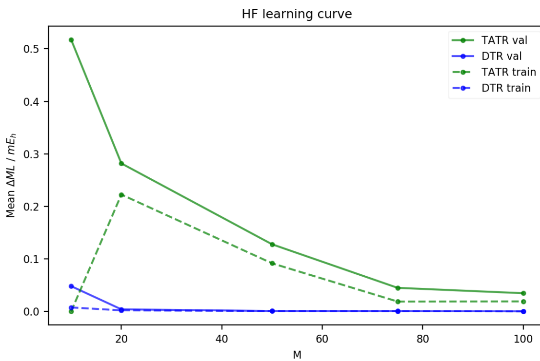
Figure B.5: DTR and TATR learning curves for HF correlation energy.
