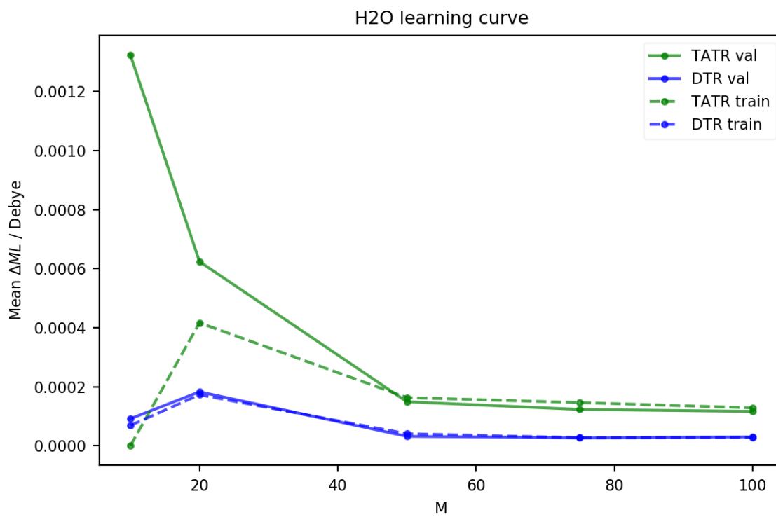
Figure B.16: DTR and TATR learning curves for H 2 O correlated dipole.
