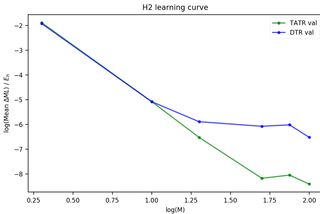
Figure B.20: DTR and TATR validation curves for H 2 correlation energy.
