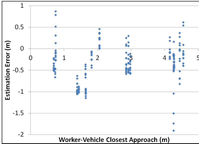
Figure 5. Linear estimator error when predicting closest approach of worker and vehicle.
