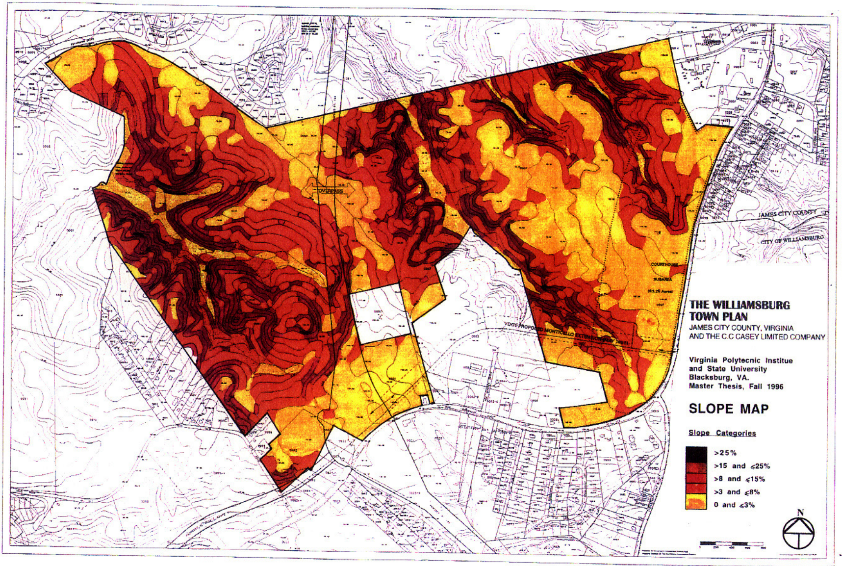
Figure 4.18 Slope map
