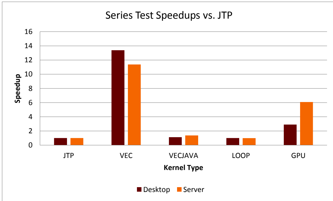
Figure 53: Series Test Speedups vs. JTP
