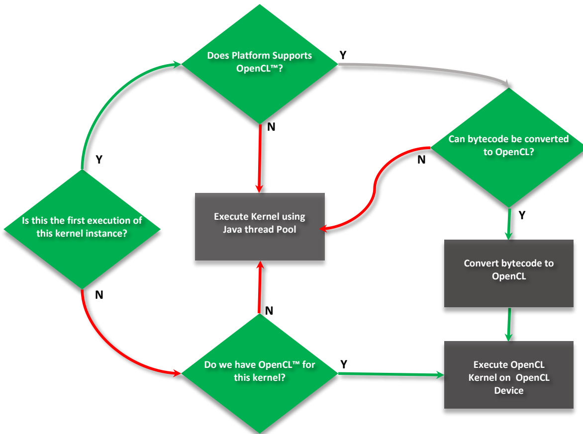
Figure 10: Aparapi Execution Logic G. Frost, "Aparapi: An Open Source tool for extending the Java promise of 'Write Once Run Anywhere' to include the GPU," Open Source Convention (OSCON), 2012. Used under fair use, 2014
