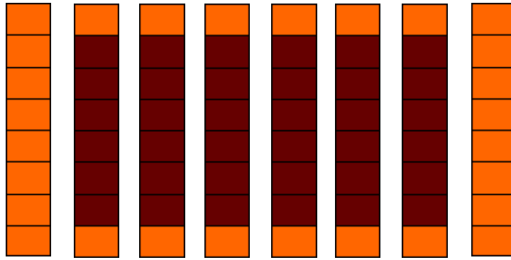
Figure 33: Auto-Vectorized Groupings
