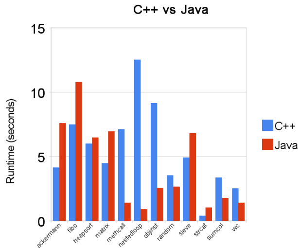
Figure 2: C++ vs Java Performance Benchmarks. C. Felde, "C++ vs Java performance: It's a tie!" 27 June 2010. [Online]. Available: http://blog.cfelde.com/2010/06/c-vs-java-performance/ . [Accessed 4 February 2014]. Used under fair use, 2014
