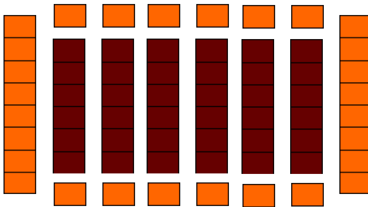
Figure 34: Hand-Vectorized Groupings
