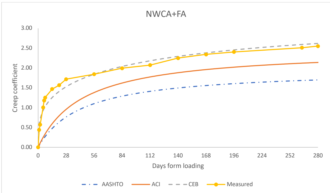
Figure 5-57: Comparison of creep coefficient calculated with predicted models of NWCA+ FA mix
