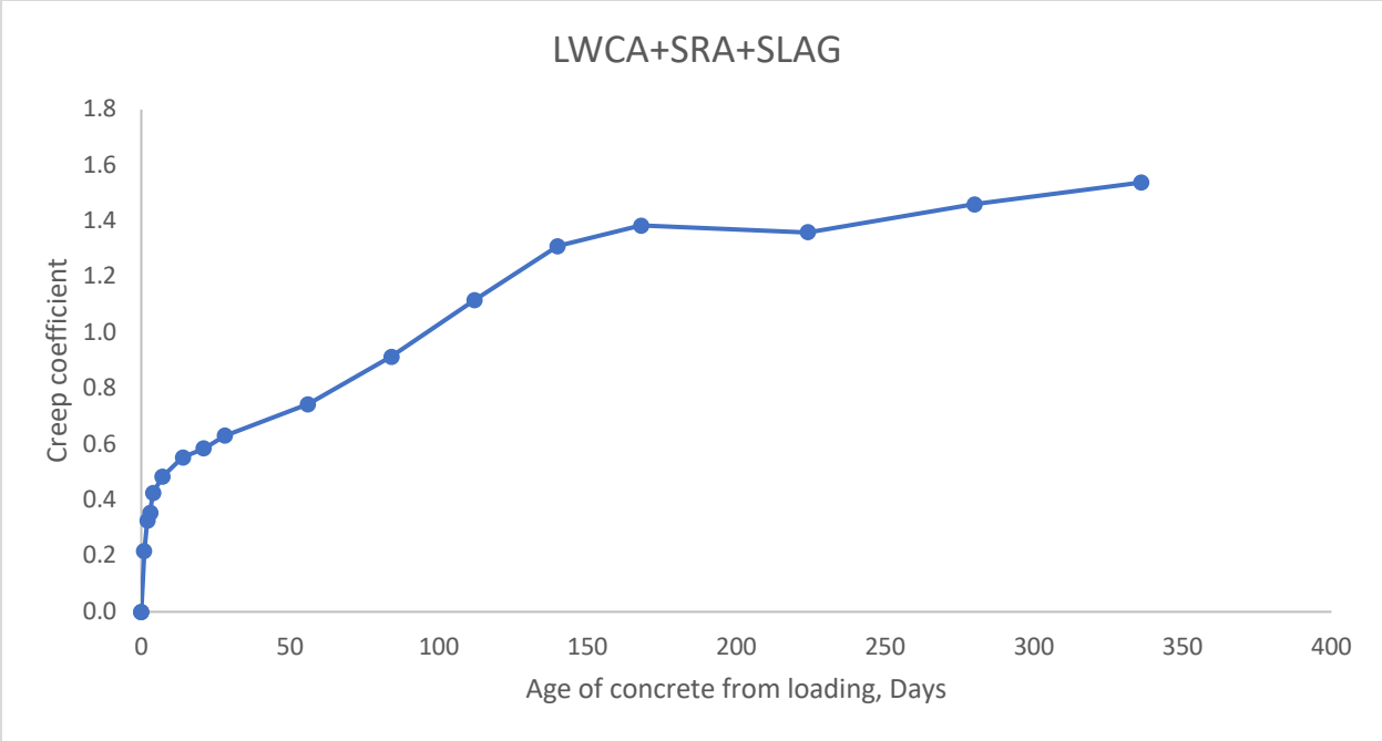
Figure 4-6: Creep coefficient, LWCA+ SRA+ SLAG
