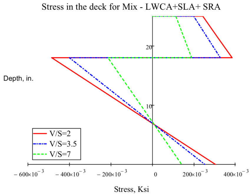
Figure 5-60: Stresses in deck for varying V/S ratio – LWCA+ SRA+ SLAG
