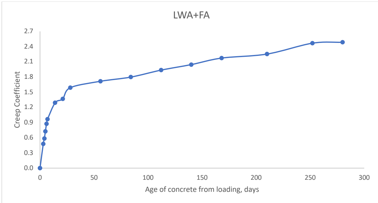
Figure 4-8: Creep coefficient, LWCA+ FA
