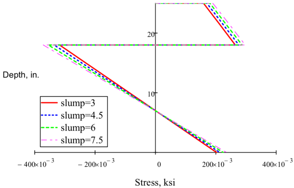
Figure 5-66: Stresses in deck for varying slump of the deck mix – NWCA+SRA+SLAG
