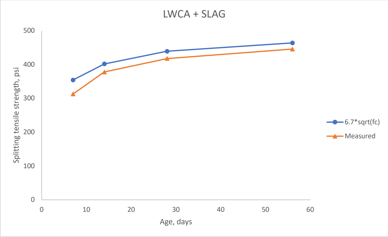
Figure 5-9: Splitting tensile strength LWCA + SLAG
