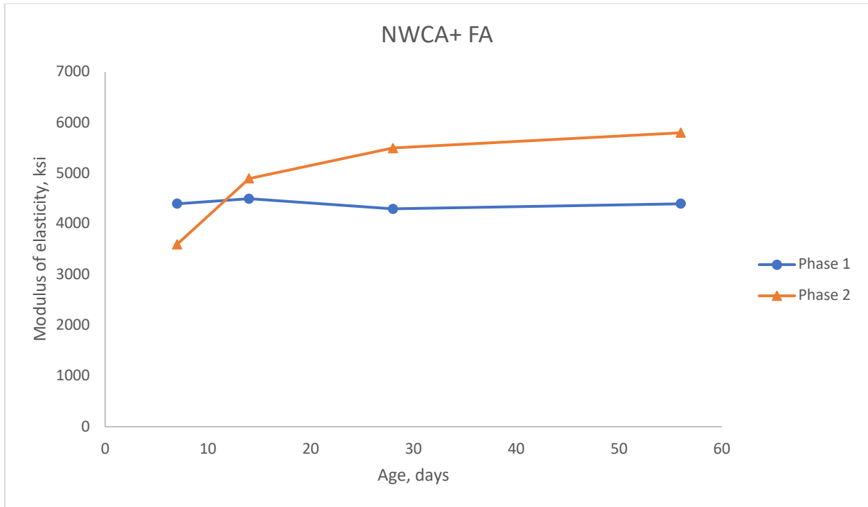
Figure 5-48: Comparison of modulus of elasticity of NWCA+ FA mix in phase I & II
