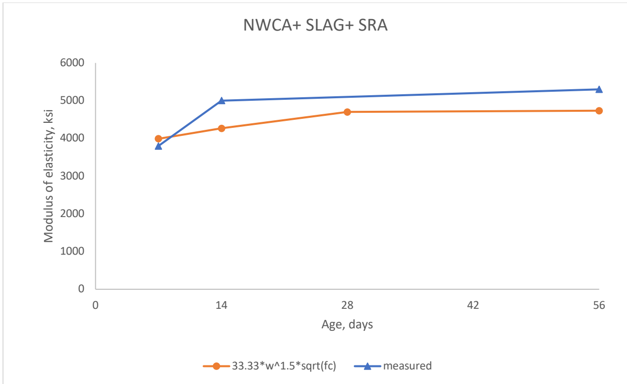
Figure 5-42: Modulus of elasticity, NWCA+ SLAG+ SRA
