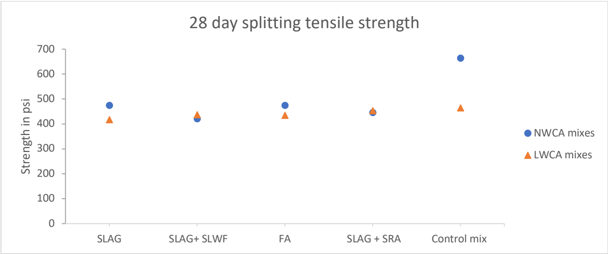
Figure 5-2: Comparison of 28-day Splitting tensile strength, phase I
