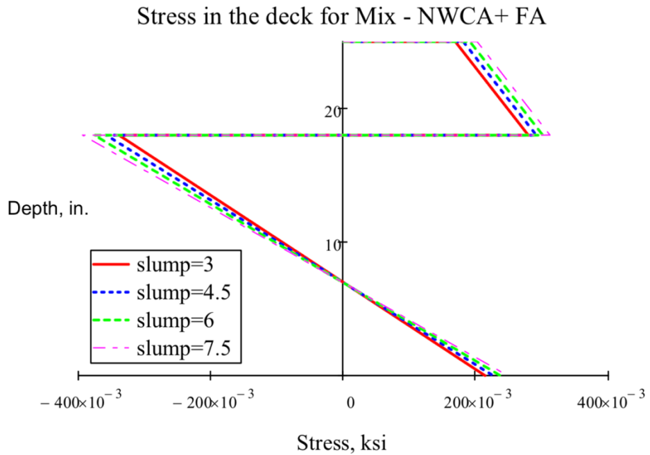
Figure 5-68: Stresses in deck for varying slump of the deck mix – NWCA+FA
