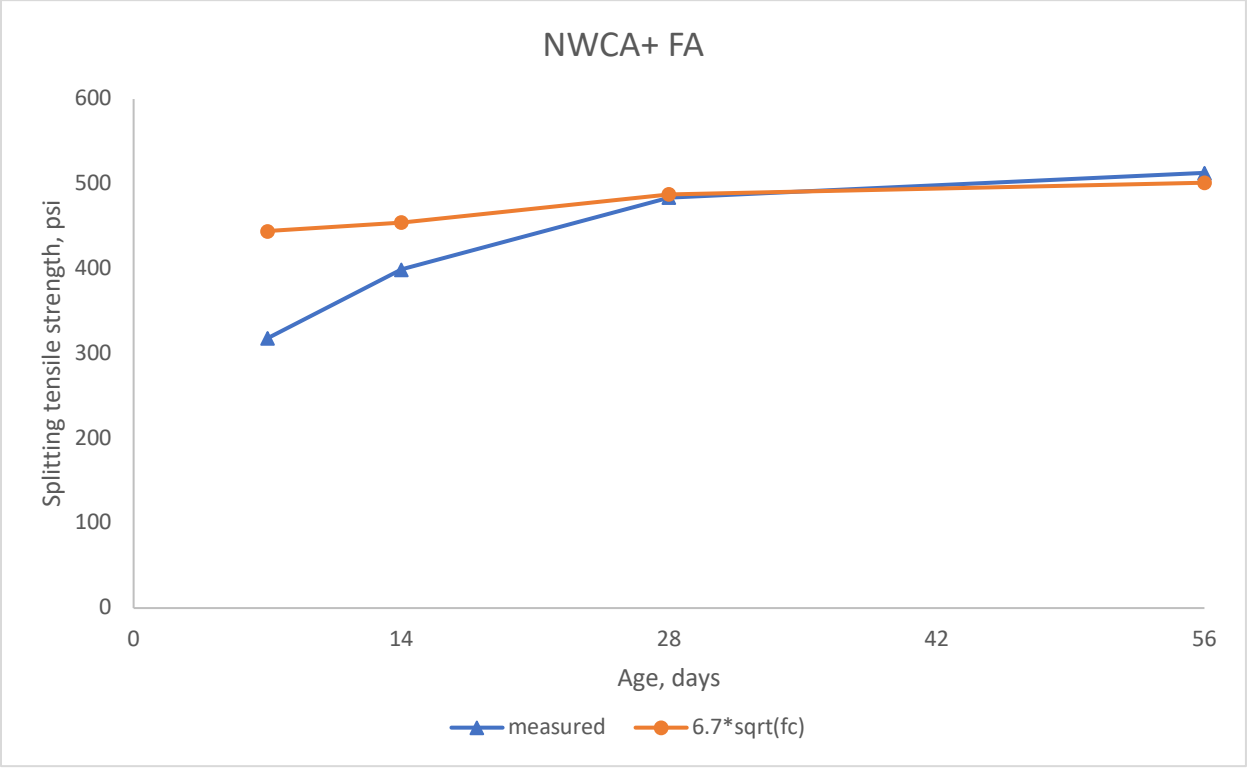
Figure 5-35: Splitting tensile strength of NWCA+ FA
