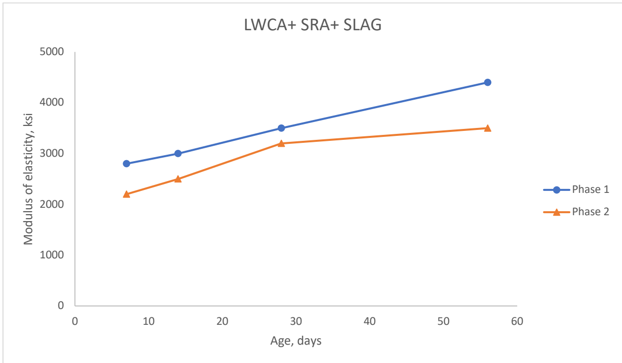
Figure 5-45: Comparison of modulus of elasticity of LWCA+ SRA+ SLAG mix in phase I & II
