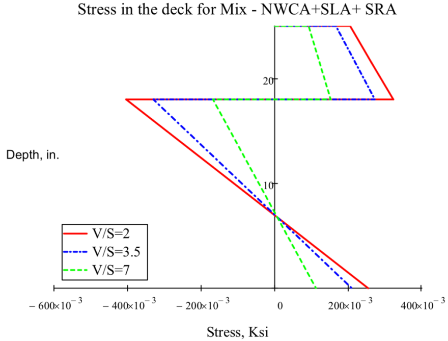
Figure 5-61: Stresses in deck for varying V/S ratio – NWCA+ SRA+ SLAG
