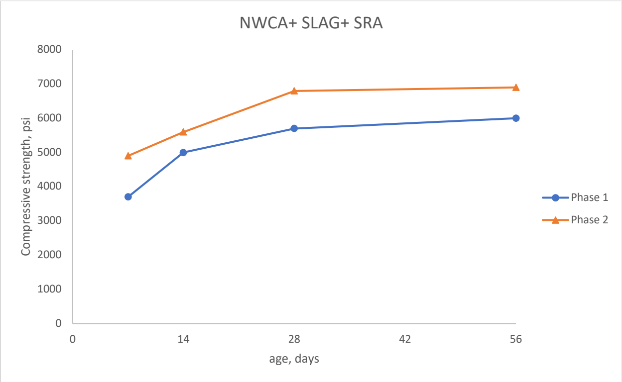
Figure 5-28: Comparison of compressive strength of NWCA+ SLAG+ SRA mix in phase I & phase II
