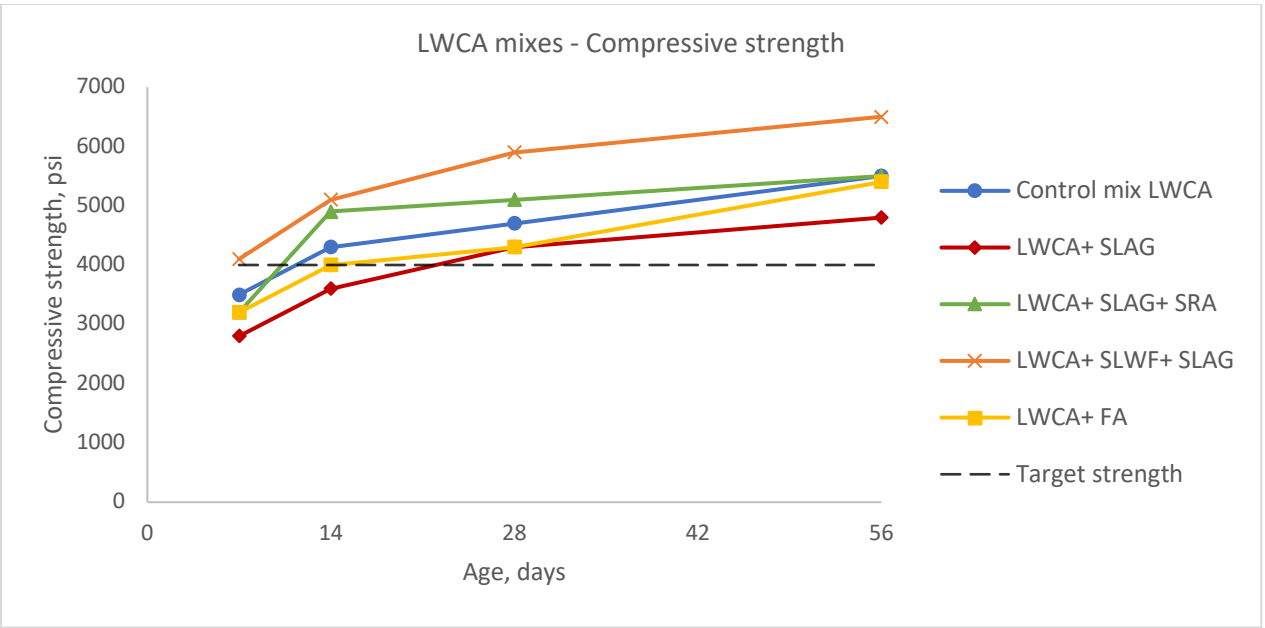
Figure 4-2 Compressive strength, LWCA mixes
