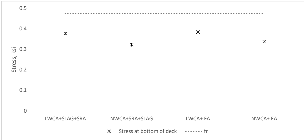
Figure 5-59: Stresses at bottom of deck for mixes in phase II
