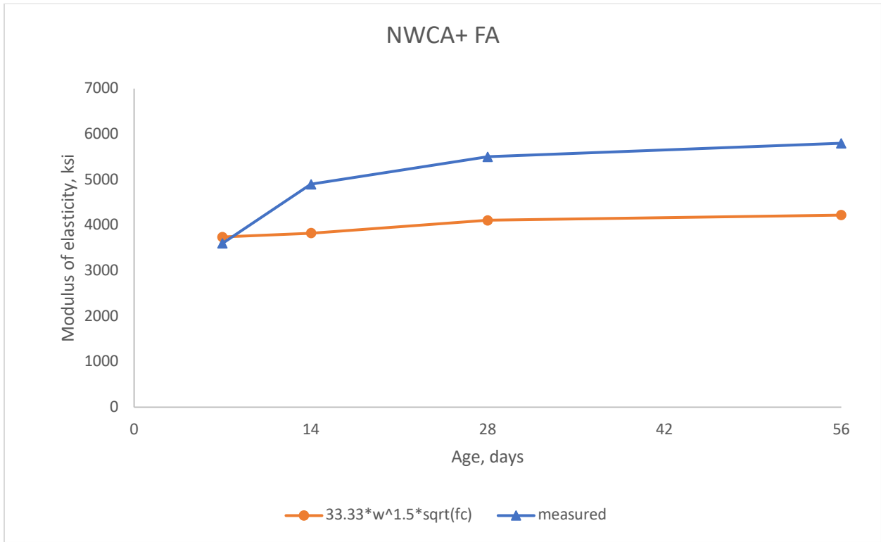
Figure 5-44: Modulus of elasticity, NWCA+ FA
