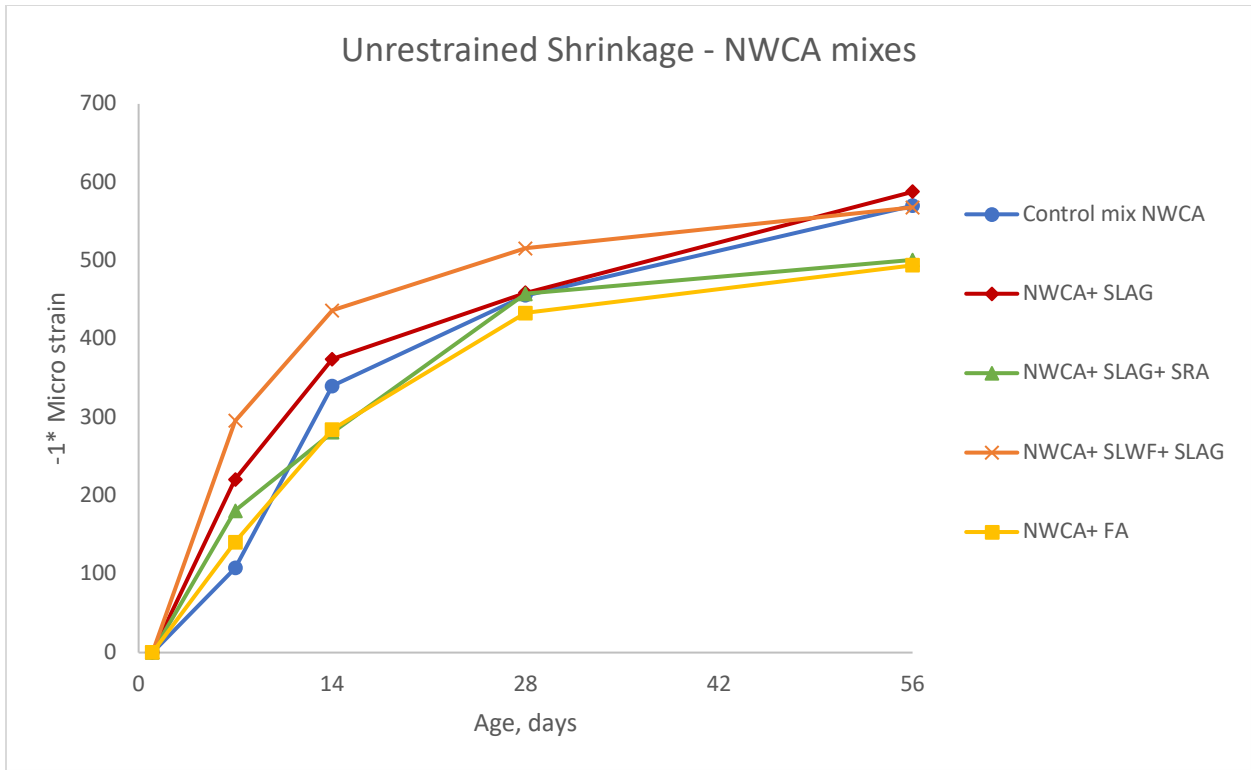
Figure 4-3: Unrestrained Shrinkage of NWCA mixtures
