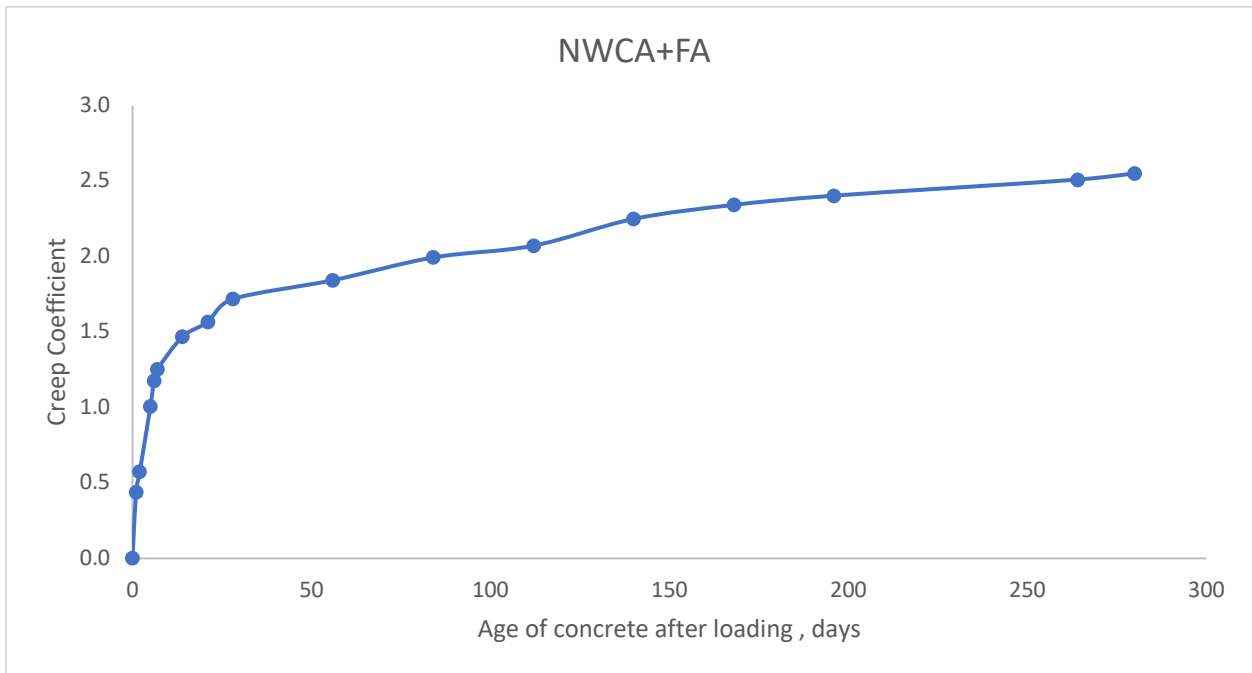
Figure 4-9: Creep coefficient, NWCA+ FA
