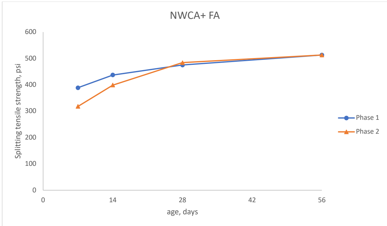
Figure 5-39: Comparison of Splitting tensile strength of NWCA+ FA mix in phase I & II
