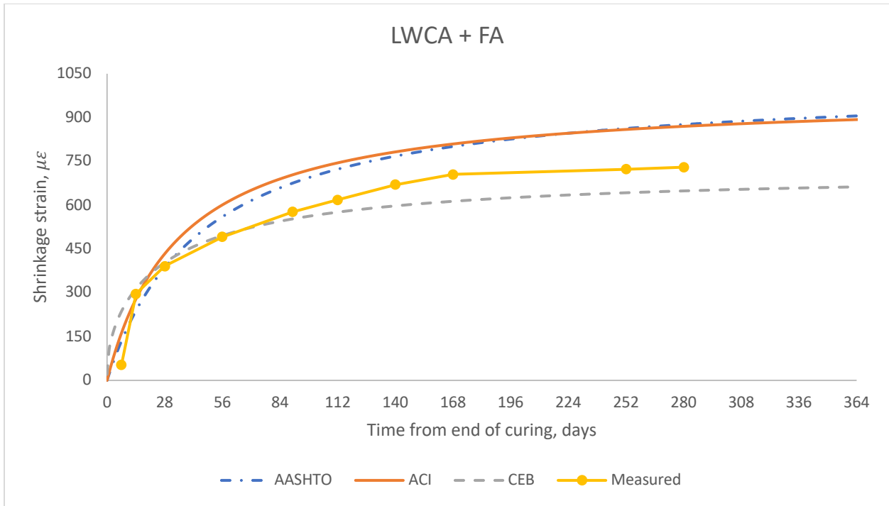
Figure 5-51: Comparison of measured shrinkage with predicted models of LWCA+FA mix
