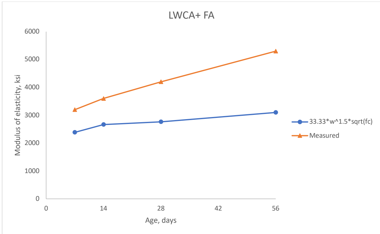
Figure 5-23: Modulus of elasticity, LWCA+ FA
