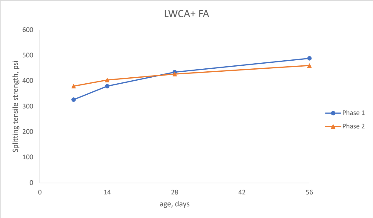
Figure 5-38: Comparison of Splitting tensile strength of LWCA+ FA mix in phase I & phase II
