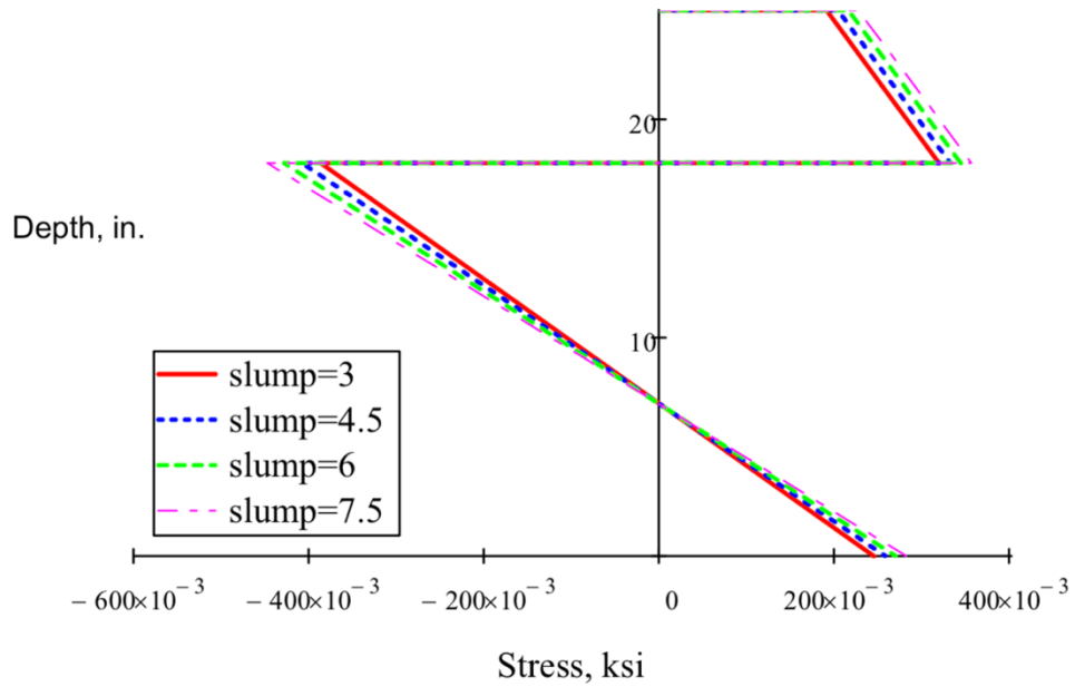
Figure 5-65: Stresses in deck for varying slump of the deck mix – LWCA+SRA+SLAG
