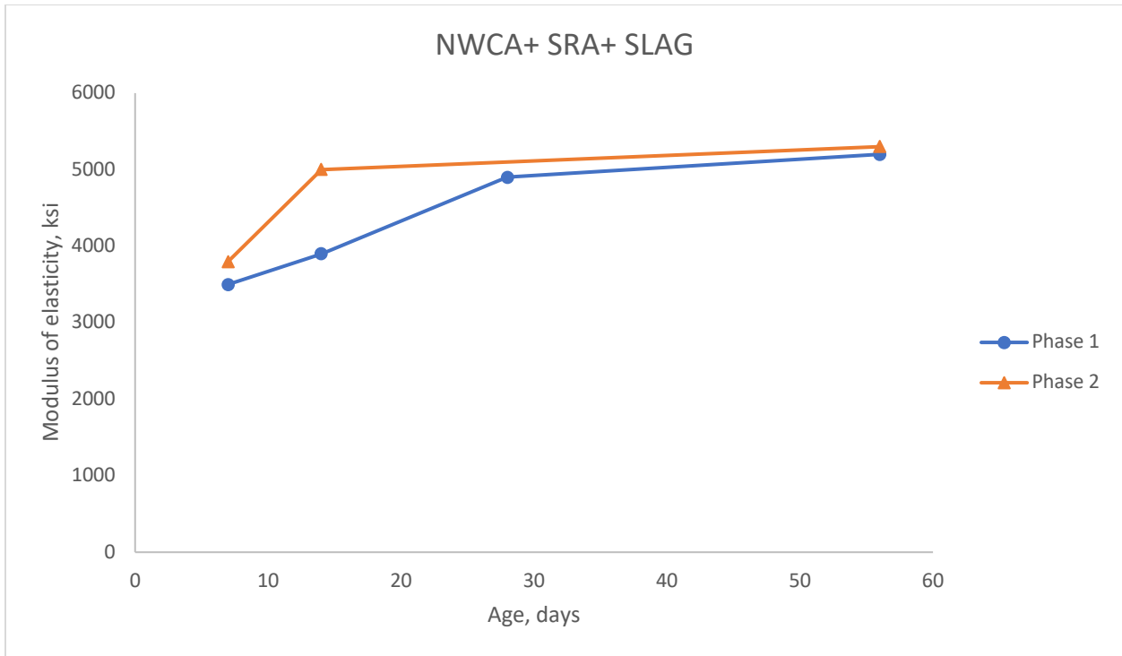
Figure 5-46: Comparison of modulus of elasticity of NWCA+ SRA+ SLAG mix in phase I & II
