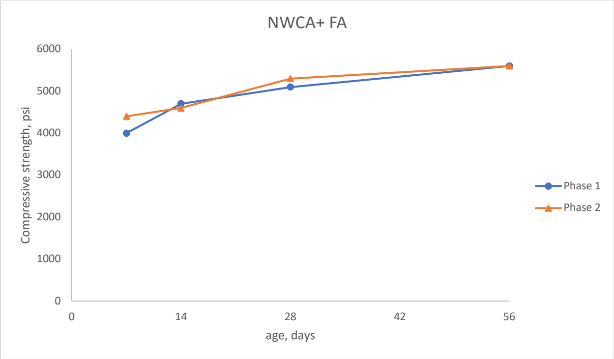
Figure 5-30: Comparison of compressive strength of NWCA+ FA mix in phase I & phase II
