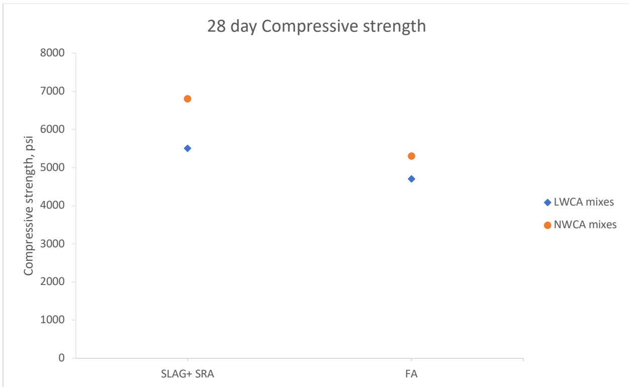
Figure 5-26: Comparison of 28-day compressive strength, phase II
