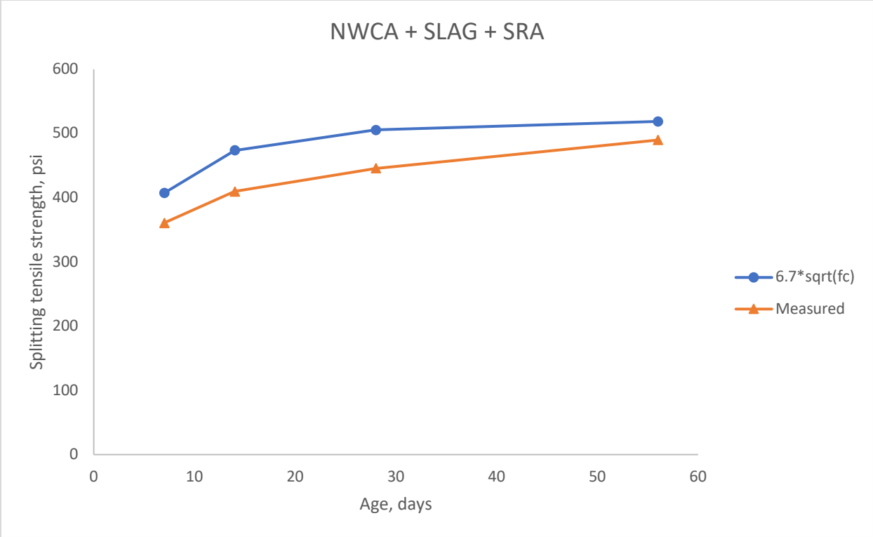
Figure 5-5: Splitting tensile strength NWCA + SLAG + SRA
