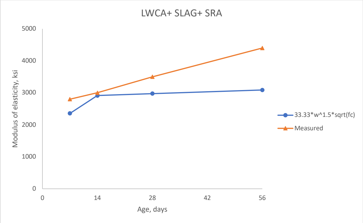
Figure 5-21: Modulus of elasticity, LWCA+ SLAG+ SRA
