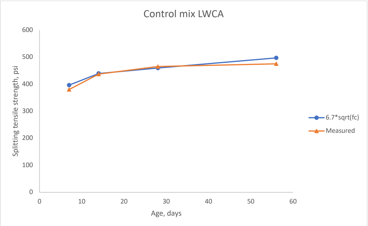
Figure 5-8: Splitting tensile strength Control mix LWCA
