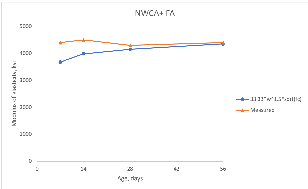
Figure 5-18: Modulus of elasticity, NWCA+ FA
