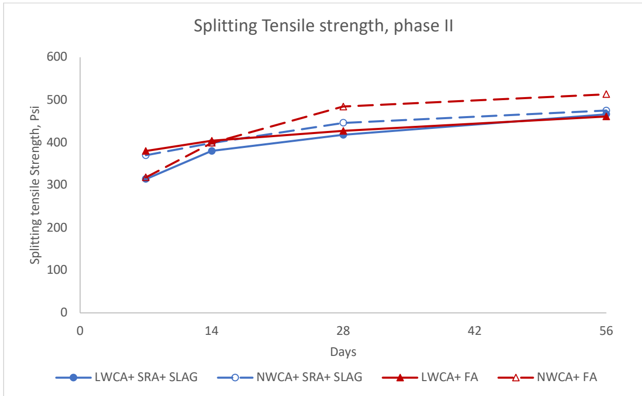
Figure 5-31: Splitting tensile strength of mixes in Phase II
