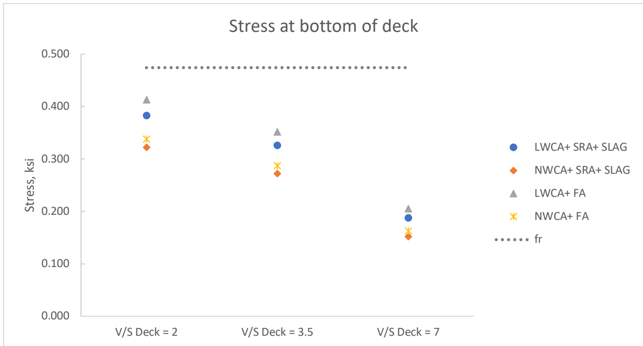
Figure 5-64: Stresses at bottom of deck for varying V/S ratio of deck
