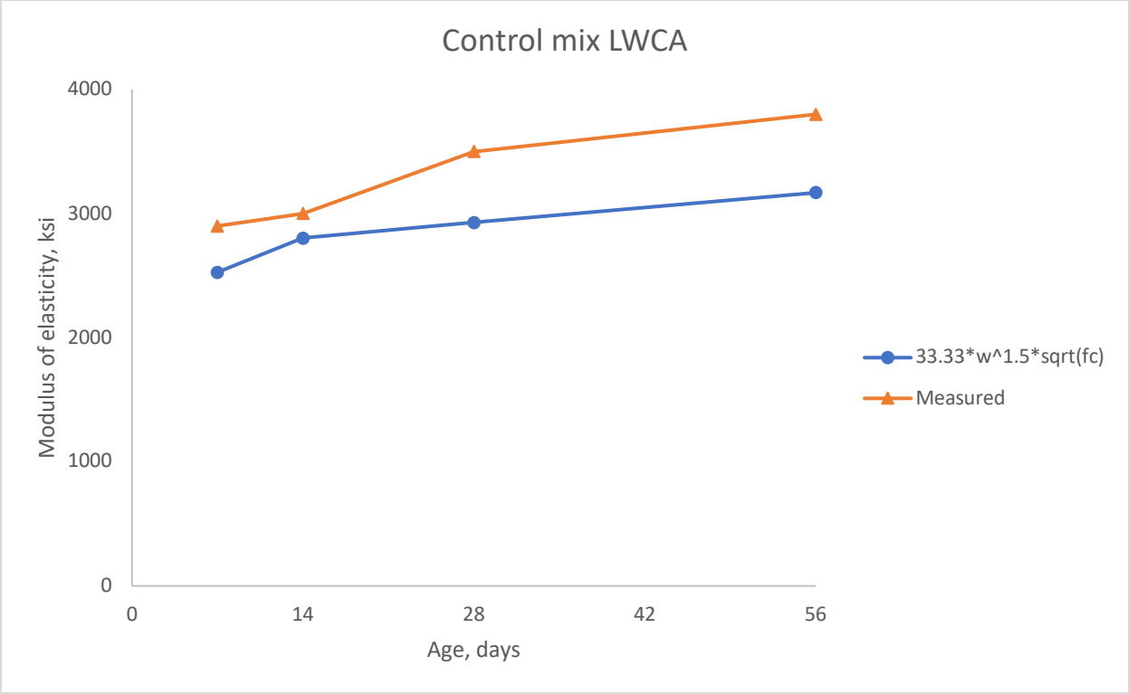
Figure 5-19: Modulus of elasticity, Control mix LWCA
