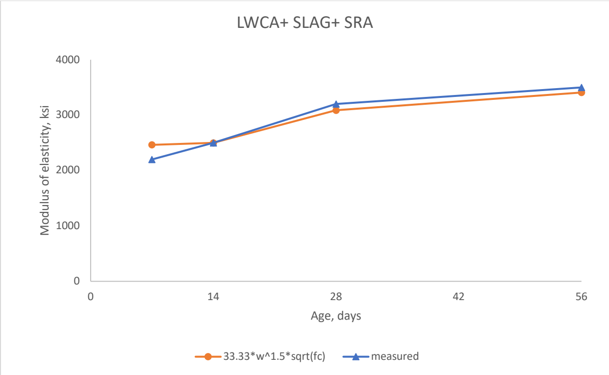
Figure 5-41: Modulus of elasticity, LWCA+ SLAG+ SRA
