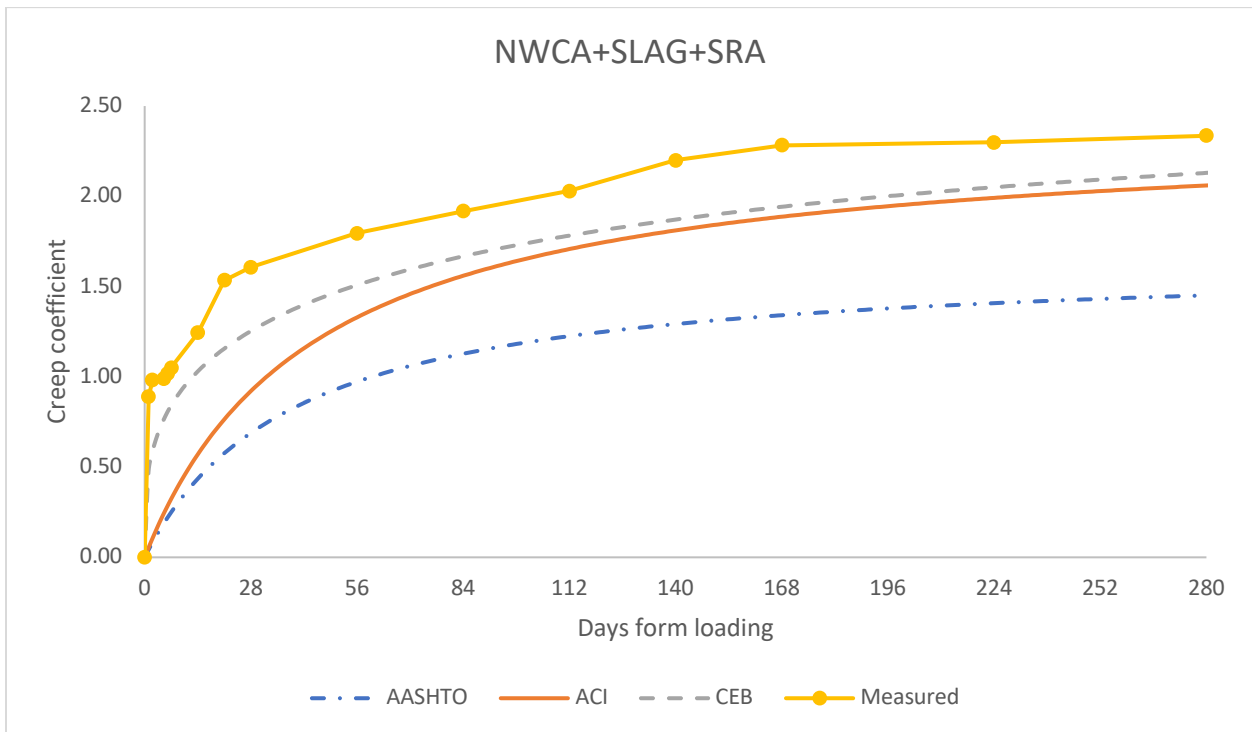
Figure 5-55: Comparison of creep coefficient calculated with predicted models of NWCA+SLAG+SRA mix
