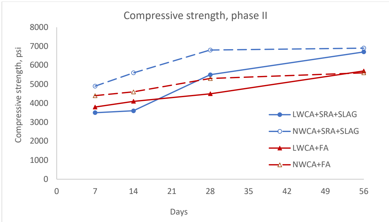
Figure 5-25: Compressive strength of mixes in Phase II
