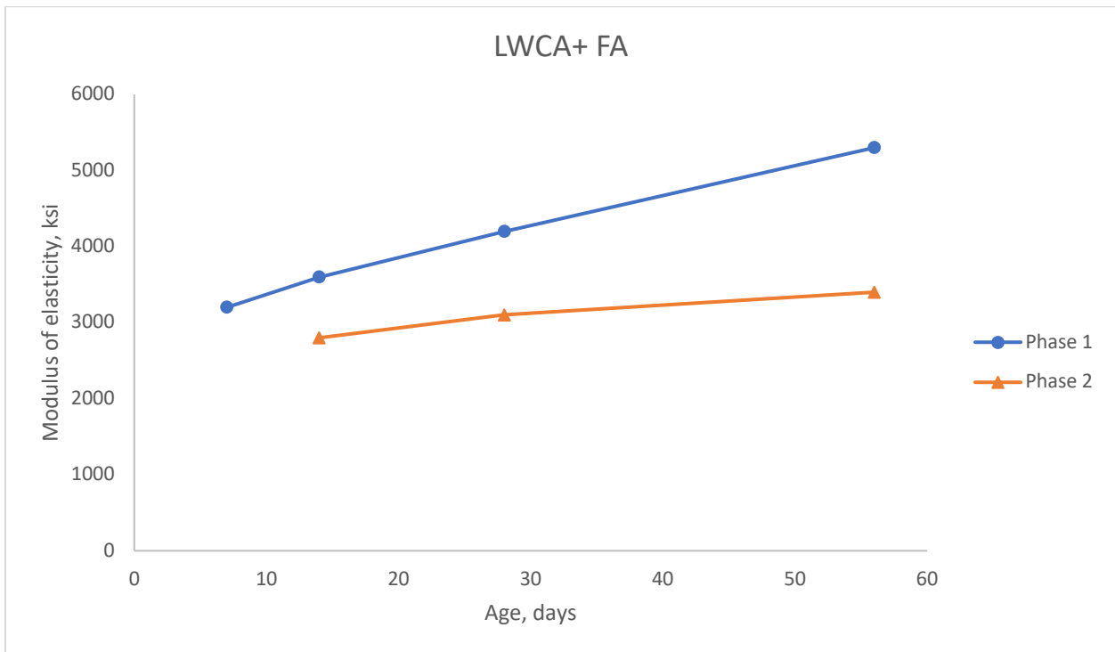
Figure 5-47: Comparison of modulus of elasticity of LWCA+ FA mix in phase I & II
