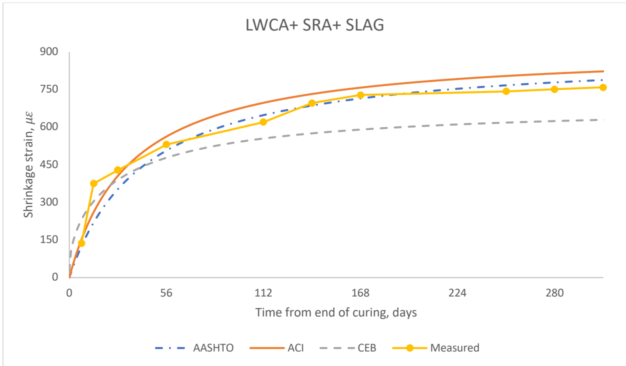
Figure 5-49: Comparison of measured shrinkage with predicted models of LWCA+SLAG+SRA mix
