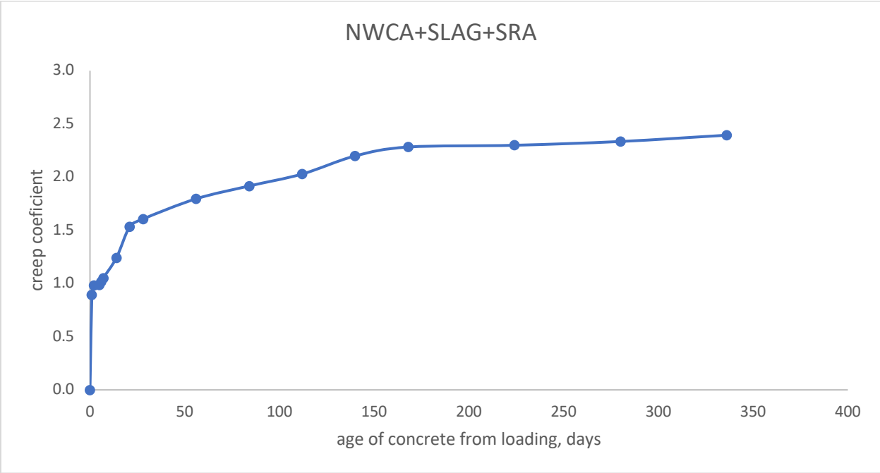
Figure 4-7: Creep coefficient, NWCA+ SRA+ SLAG
