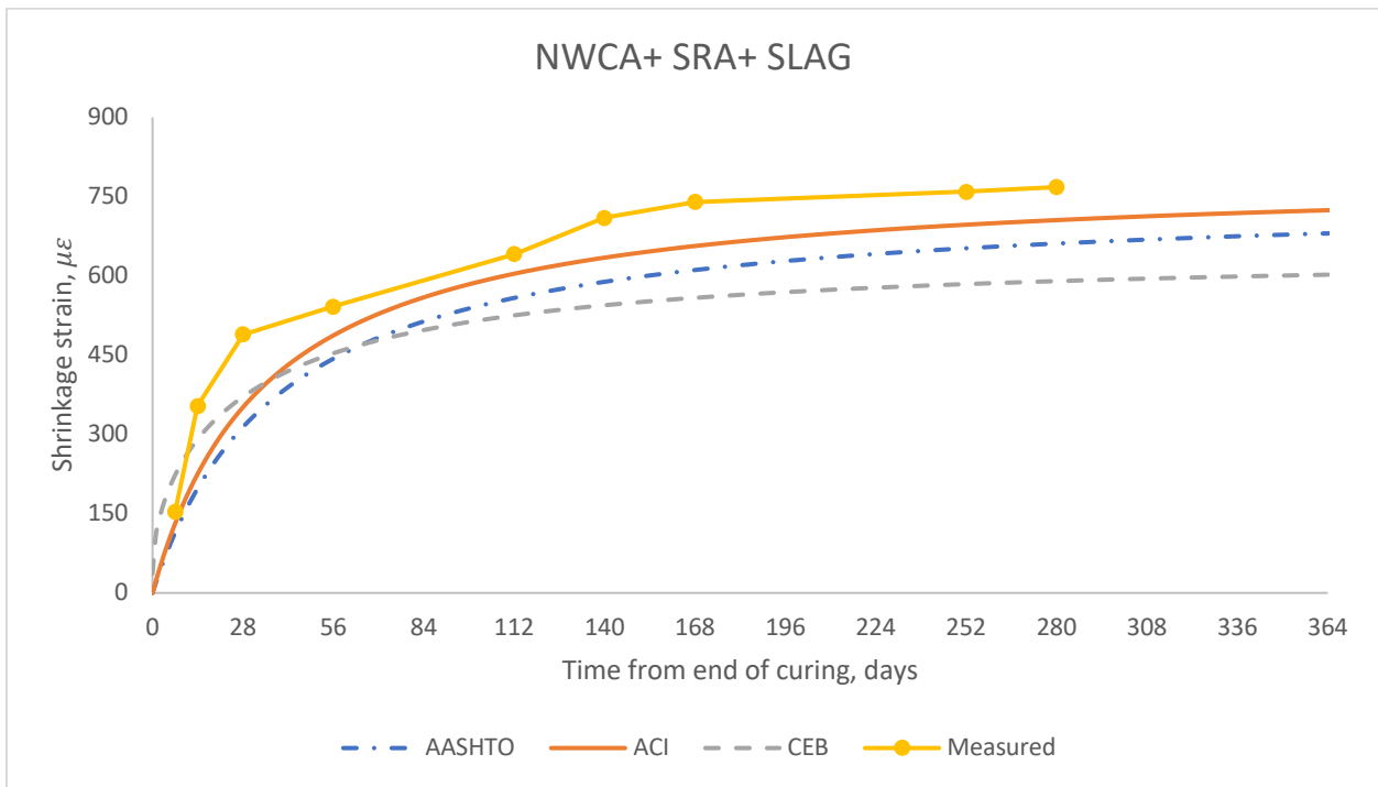
Figure 5-50: Comparison of measured shrinkage with predicted models of NWCA+SLAG+SRA mix
