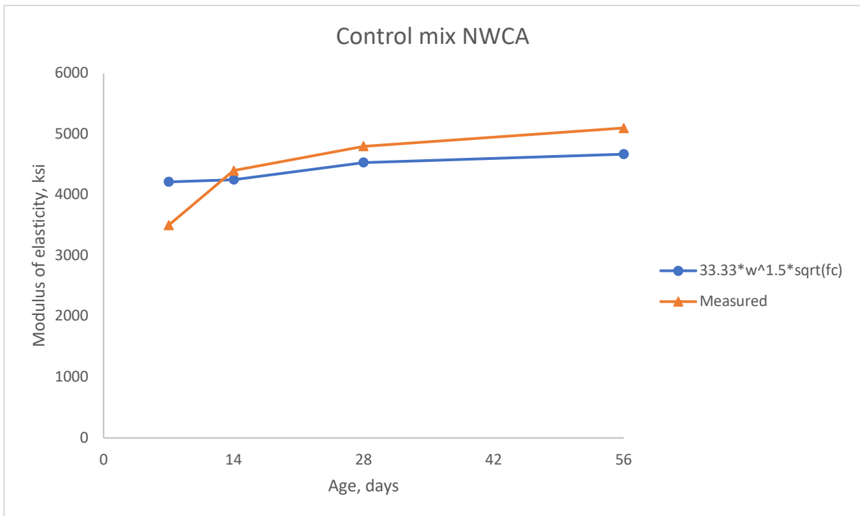
Figure 5-14: Modulus of elasticity, Control mix NWCA
