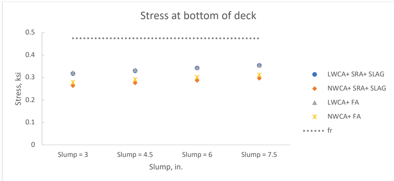
Figure 5-69: Stresses at bottom of deck for varying slump of deck concrete
