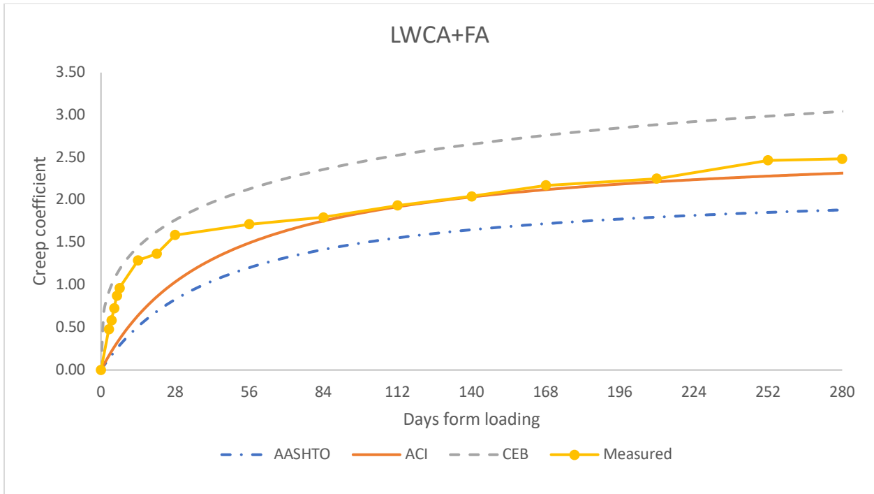
Figure 5-56: Comparison of creep coefficient calculated with predicted models of LWCA+ FA mix
