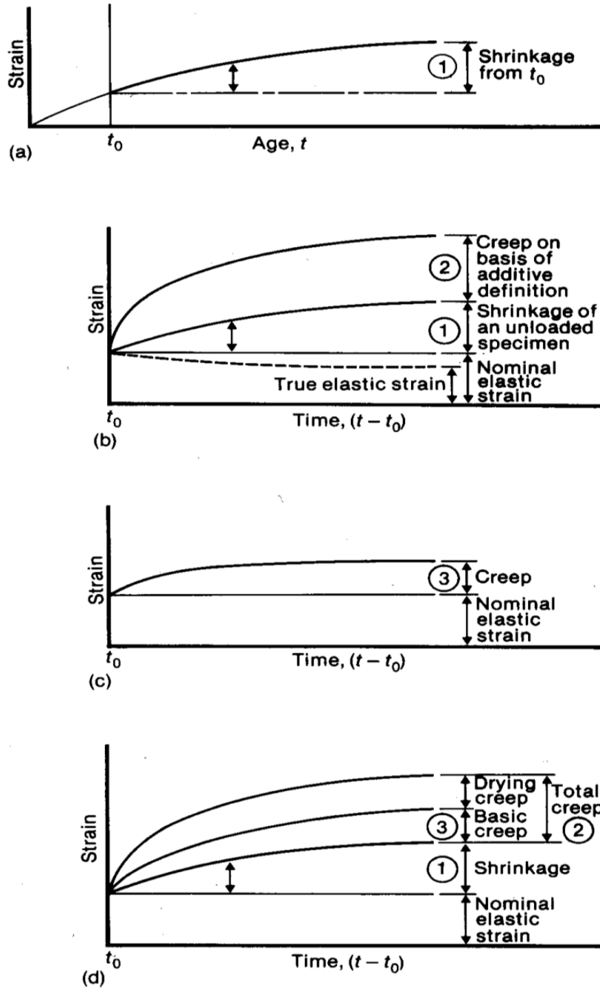
Figure 2-1: (a) Shrinkage of unloaded specimen, (b) Change in strain of a loaded and drying specimen, (c) Creep of a loaded specimen in hygral equilibrium with the ambient medium. (d) Change in strain of a loaded and drying specimen (Neville, 1983)
