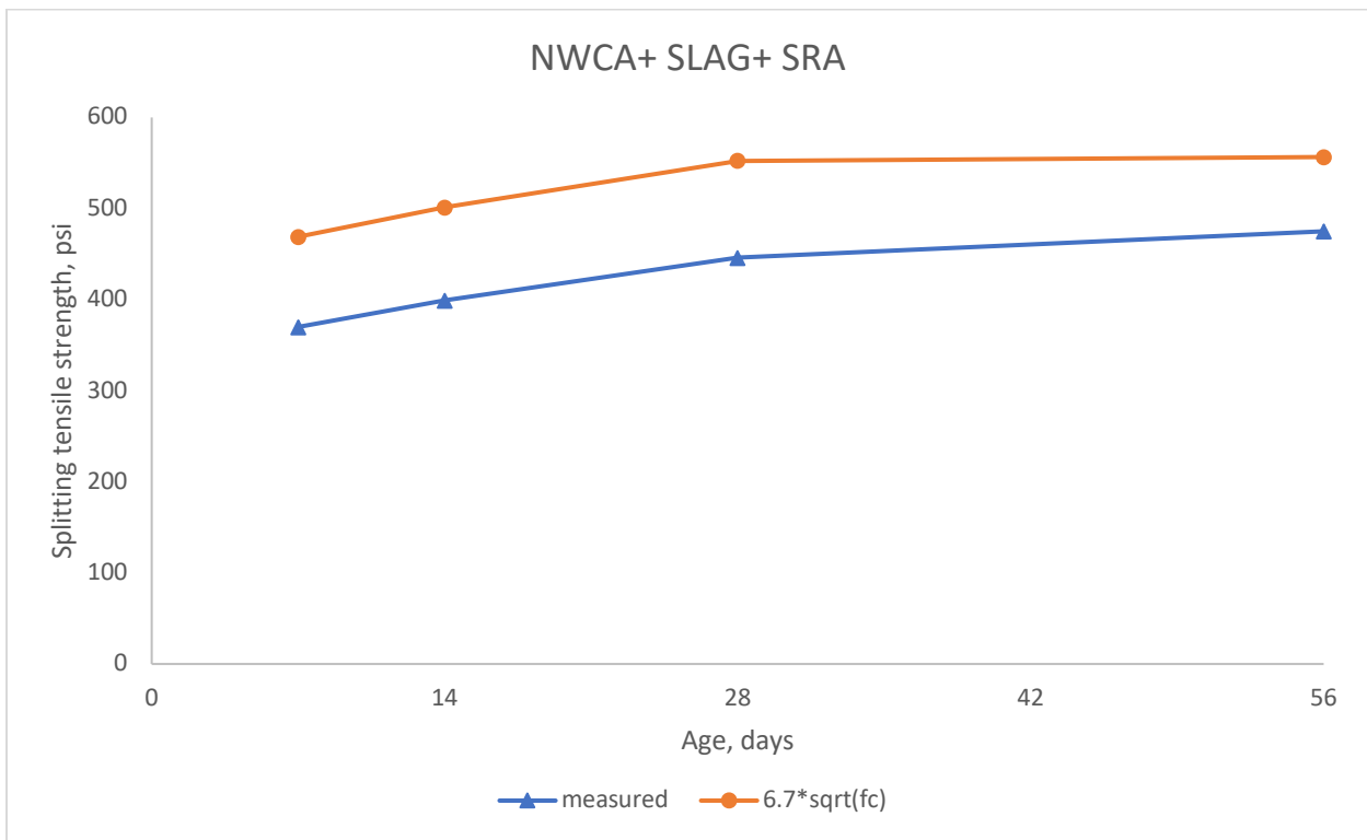
Figure 5-33: Splitting tensile strength of NWCA+ SLAG+ SRA
