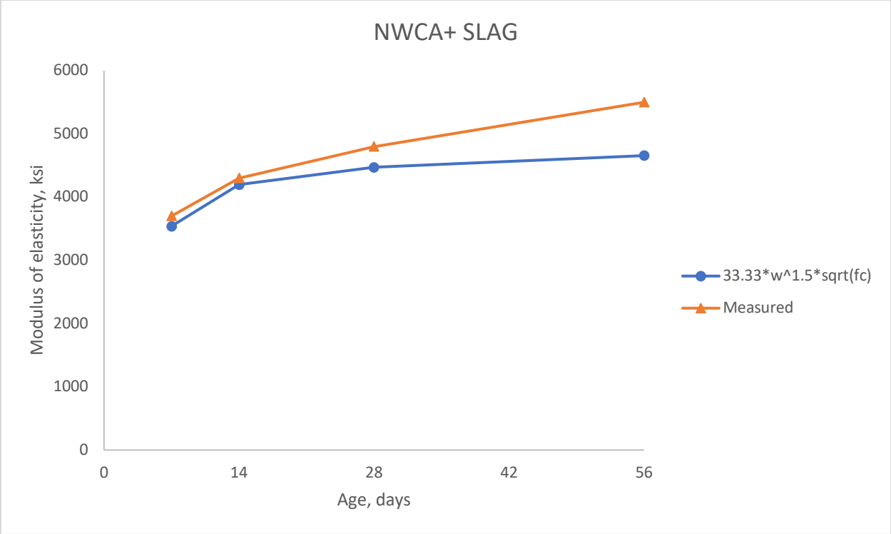
Figure 5-15: Modulus of elasticity, NWCA+ SLAG
