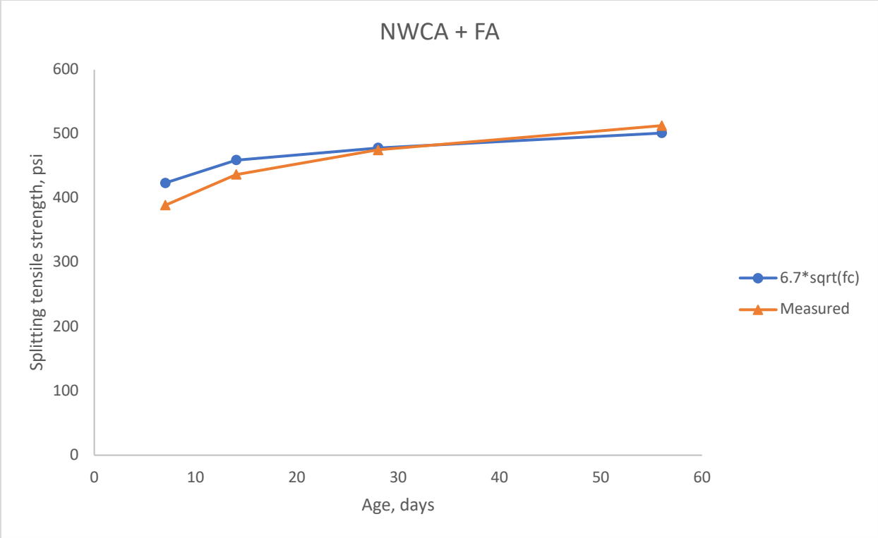
Figure 5-7: Splitting tensile strength NWCA +FA
