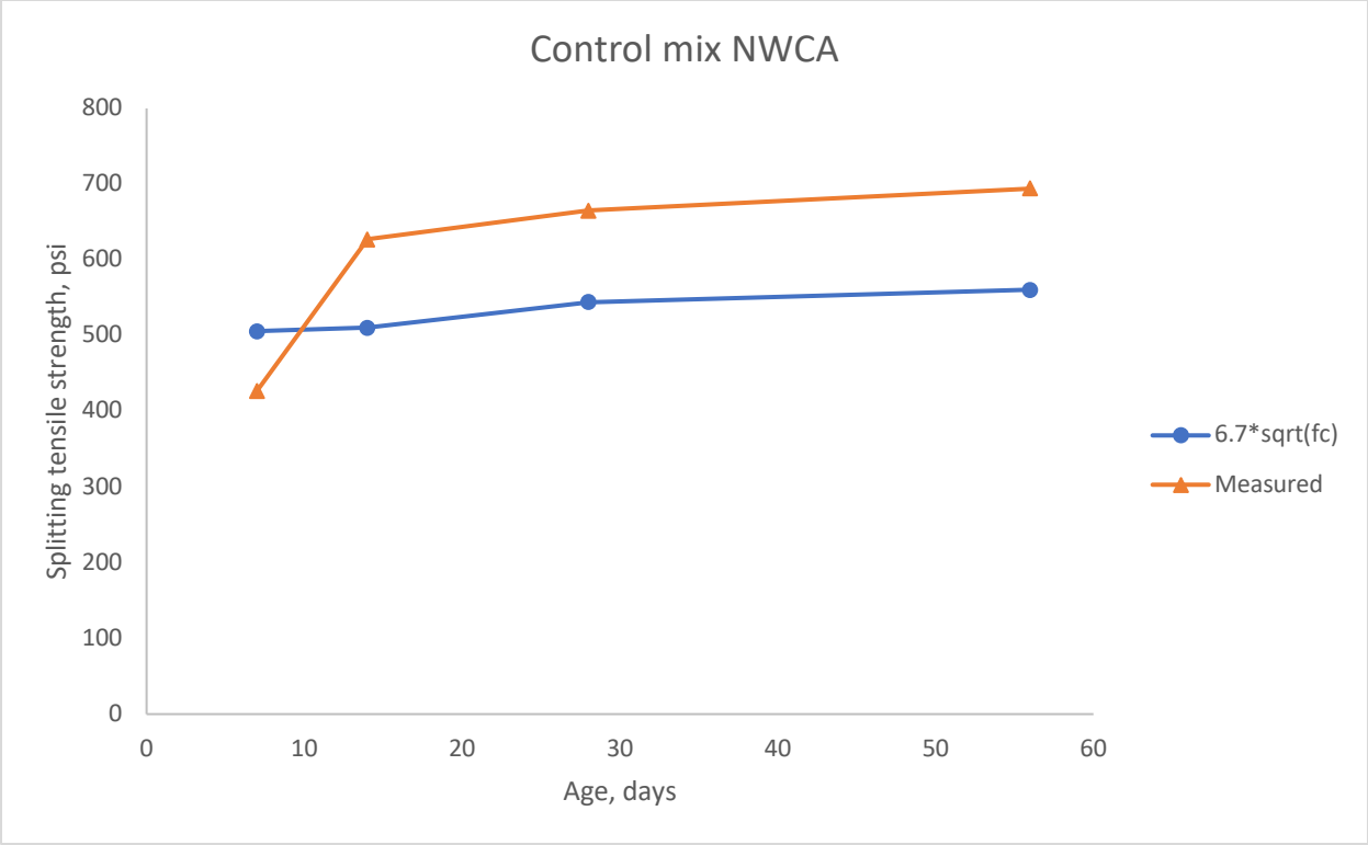
Figure 5-3: Splitting tensile strength Control mix NWCA
