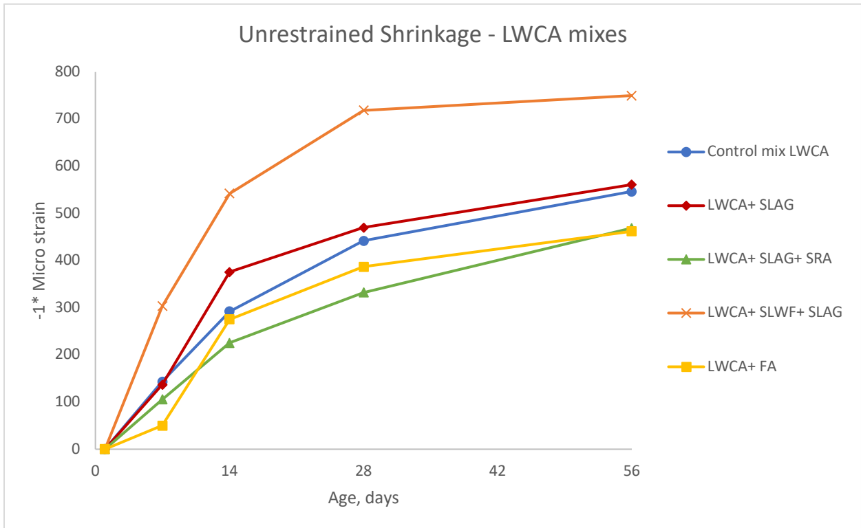
Figure 4-4: Unrestrained Shrinkage of LWCA mixtures
