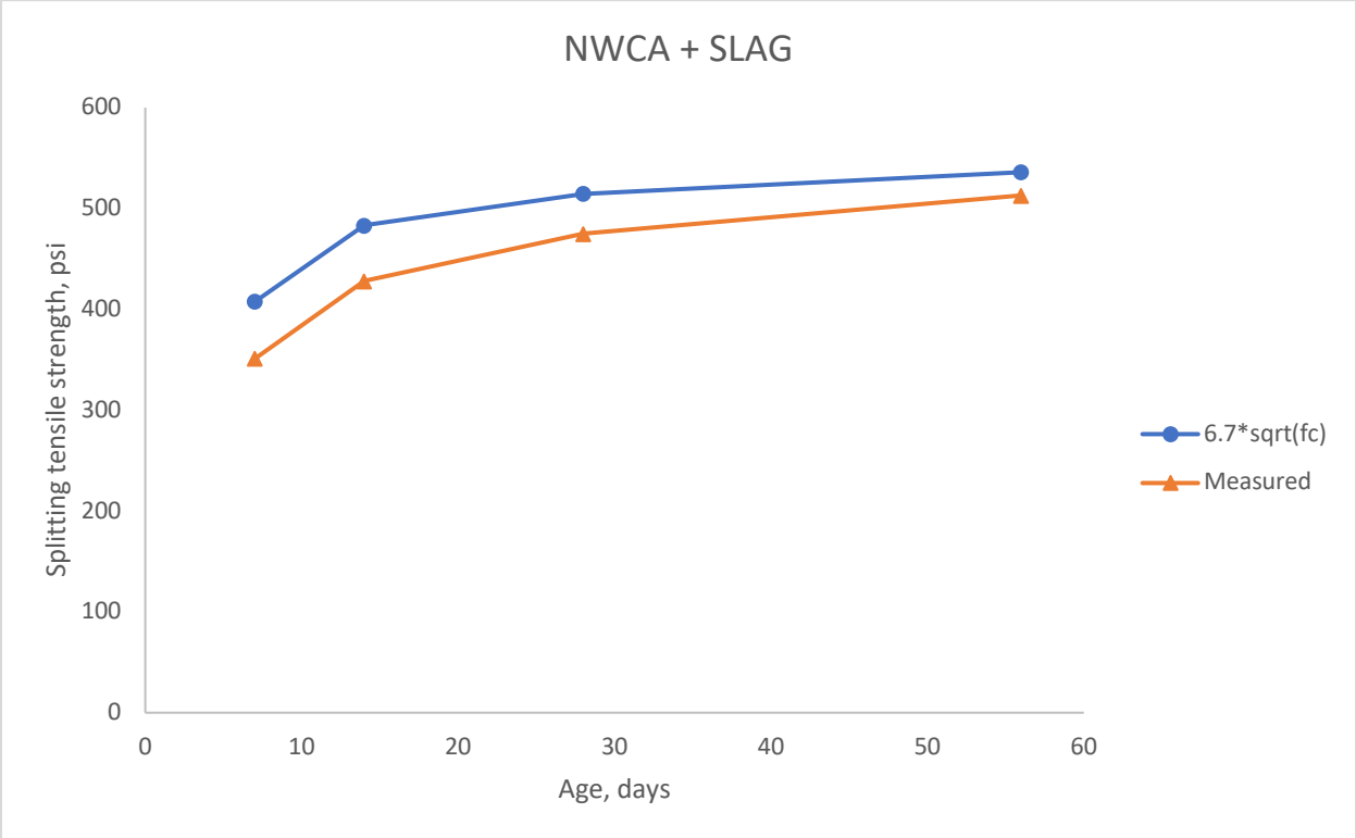
Figure 5-4: Splitting tensile strength NWCA + SLAG
