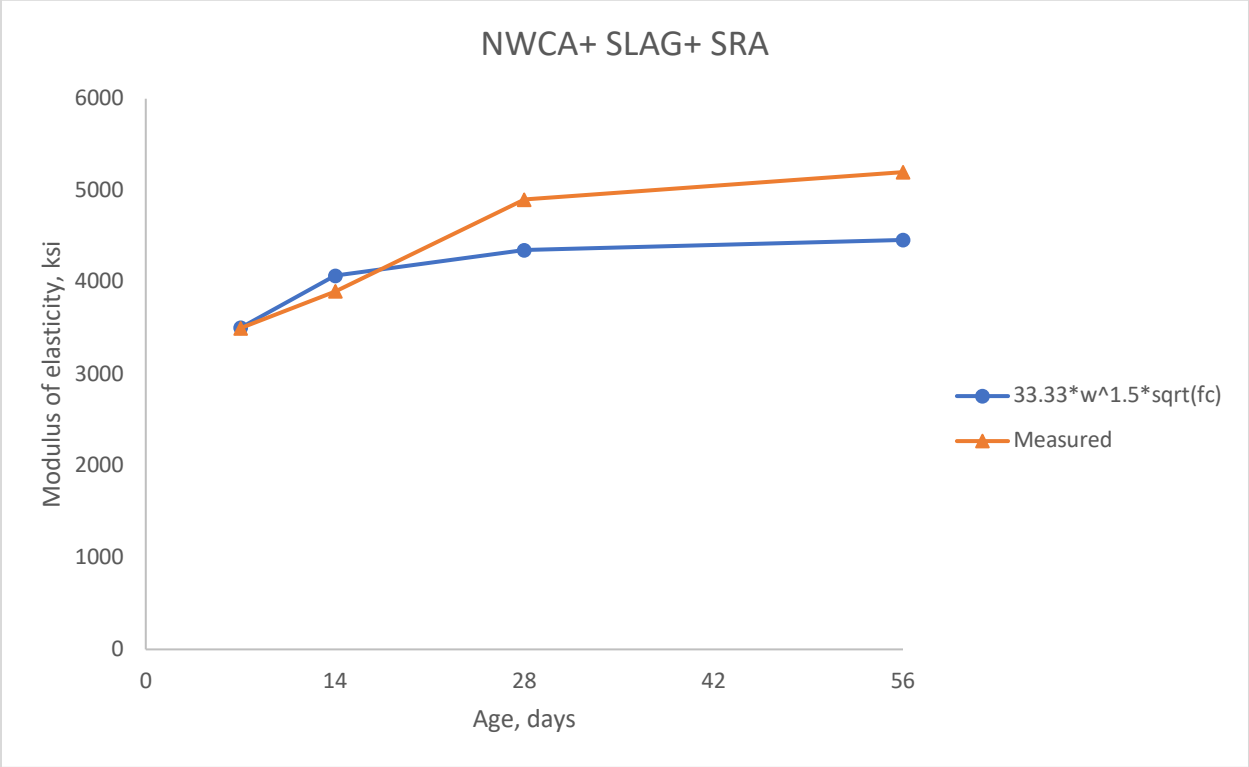
Figure 5-16: Modulus of elasticity, NWCA+ SLAG+ SRA
