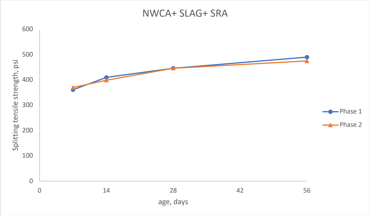
Figure 5-37: Comparison of Splitting tensile strength of NWCA+ slag+ SRA mix in phase I & phase II
