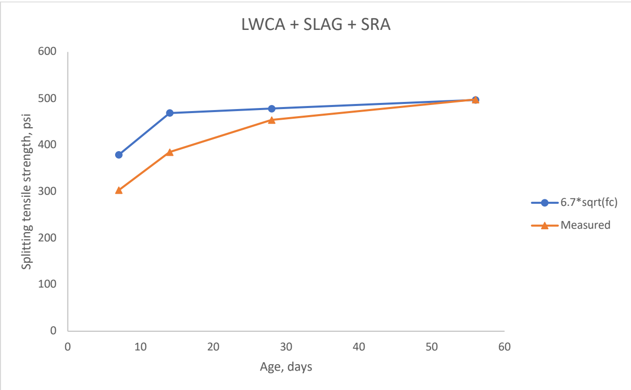
Figure 5-10: Splitting tensile strength LWCA + SLAG+ SRA
