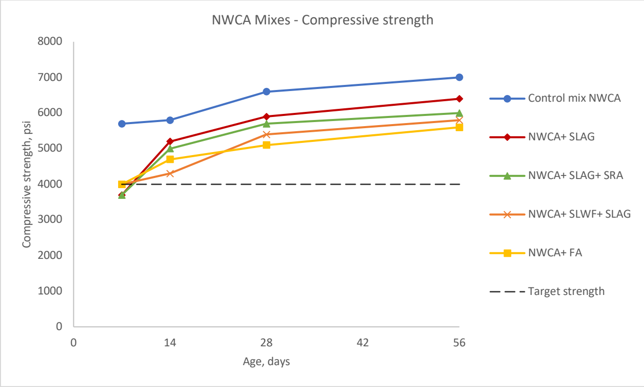
Figure 4-1: Compressive strength, NWCA mixes
