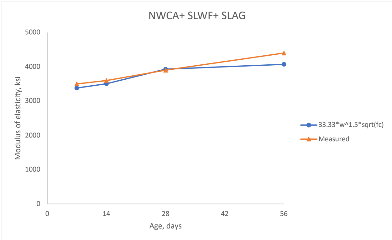
Figure 5-17: Modulus of elasticity, NWCA+ SLWF+ SLAG
