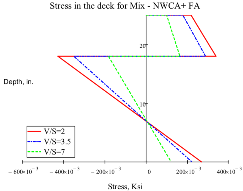
Figure 5-63: Stresses in deck for varying V/S ratio – LWCA+ FA
