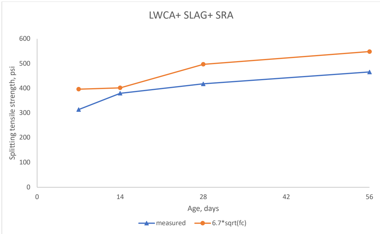
Figure 5-32: Splitting tensile strength of LWCA+ SLAG+ SRA
