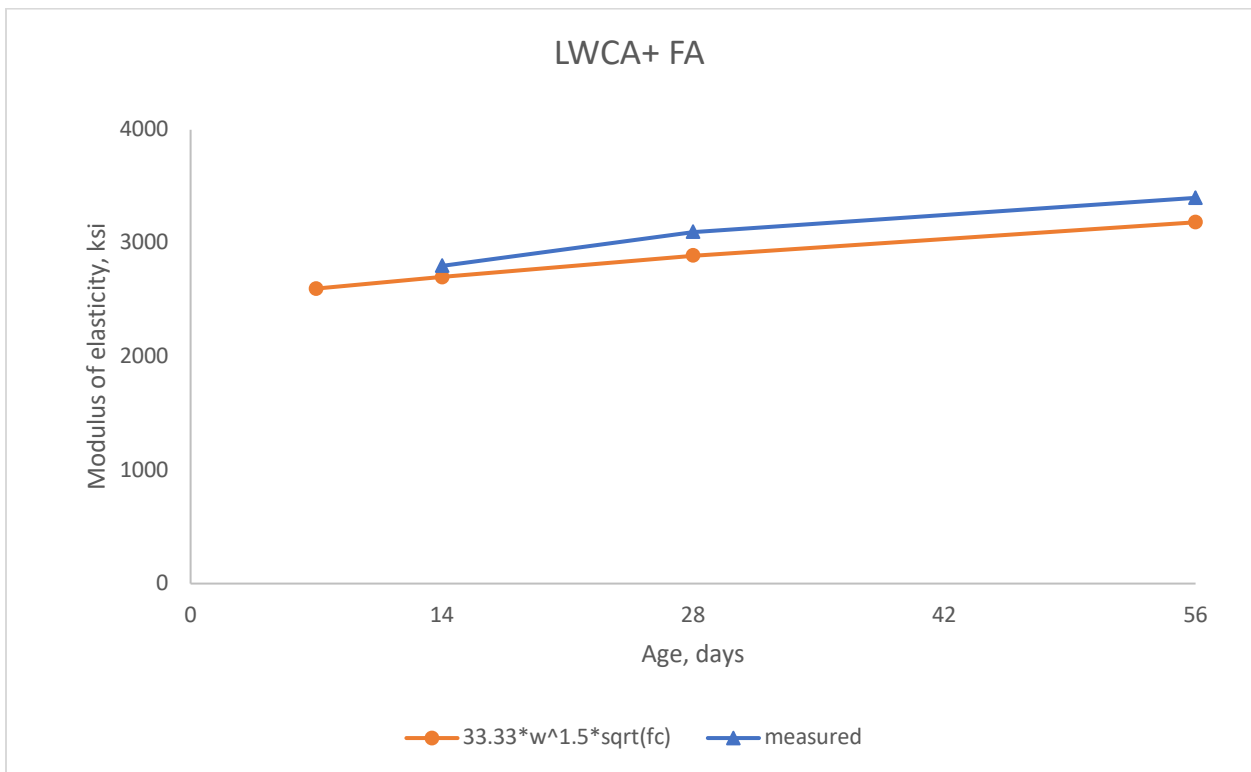
Figure 5-43: Modulus of elasticity, LWCA+ FA
