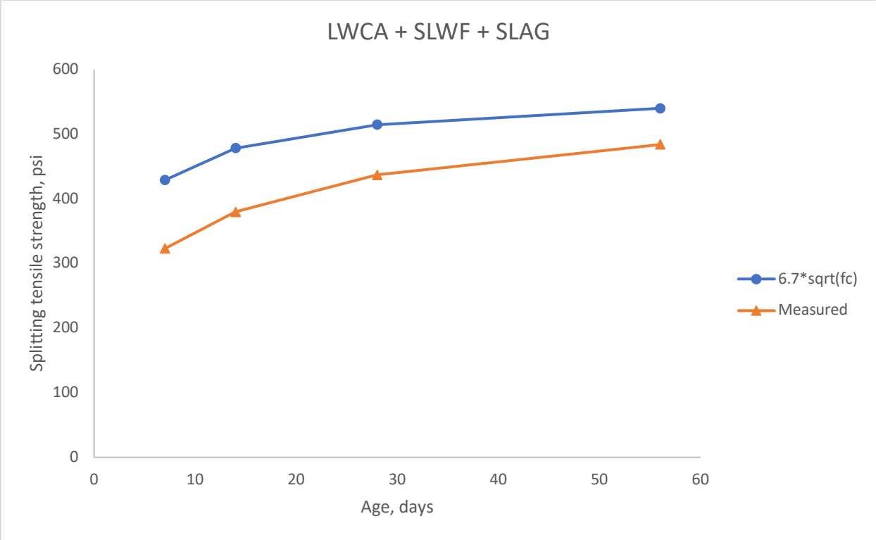
Figure 5-11: Splitting tensile strength LWCA + SLWF + SLAG
