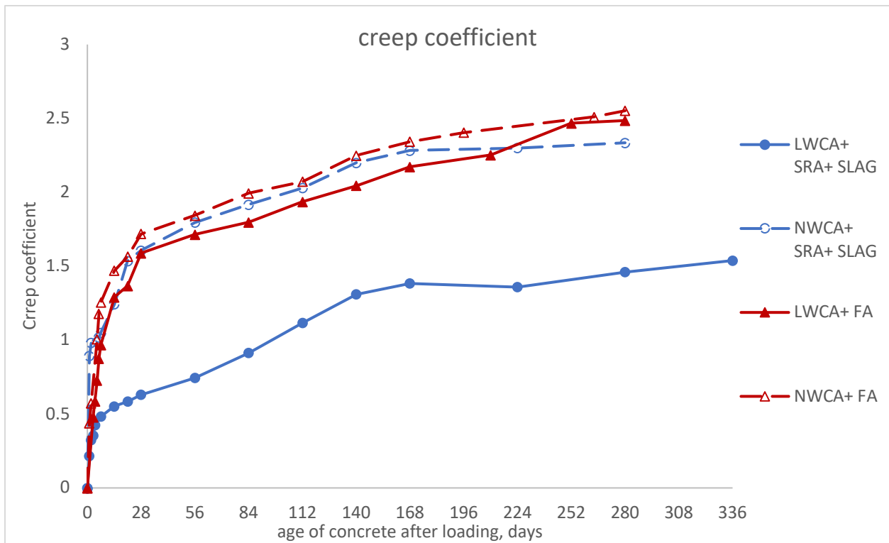
Figure 5-53: Creep coefficient for mixes in phase II
