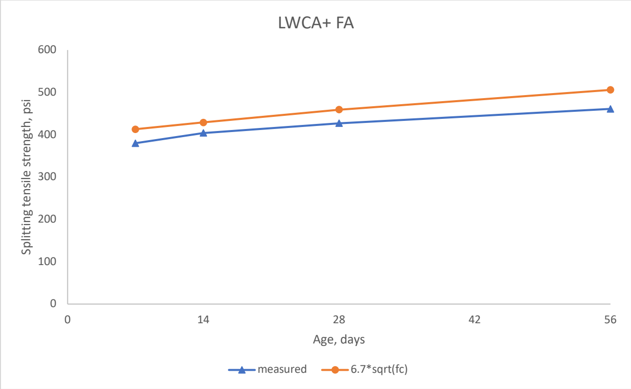
Figure 5-34: Splitting tensile strength of LWCA+ FA
