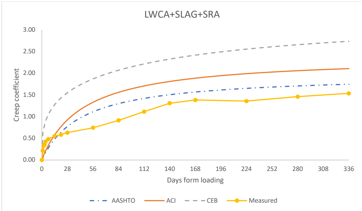
Figure 5-54: Comparison of creep coefficient calculated with predicted models of LWCA+SLAG+SRA mix
