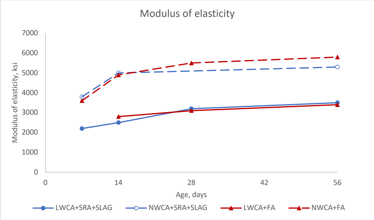
Figure 5-40: Modulus of elasticity of mixes in phase II
