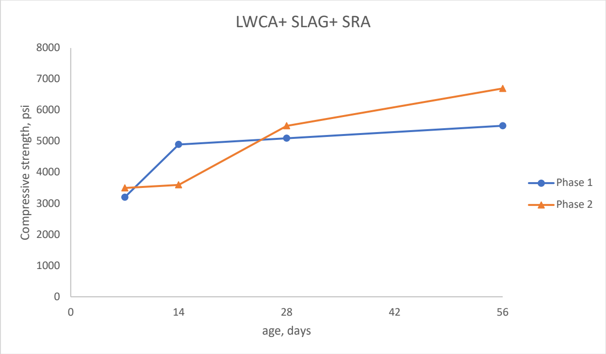
Figure 5-27: Comparison of compressive strength of LWCA+ slag+ SRA mix in phase I & phase II
