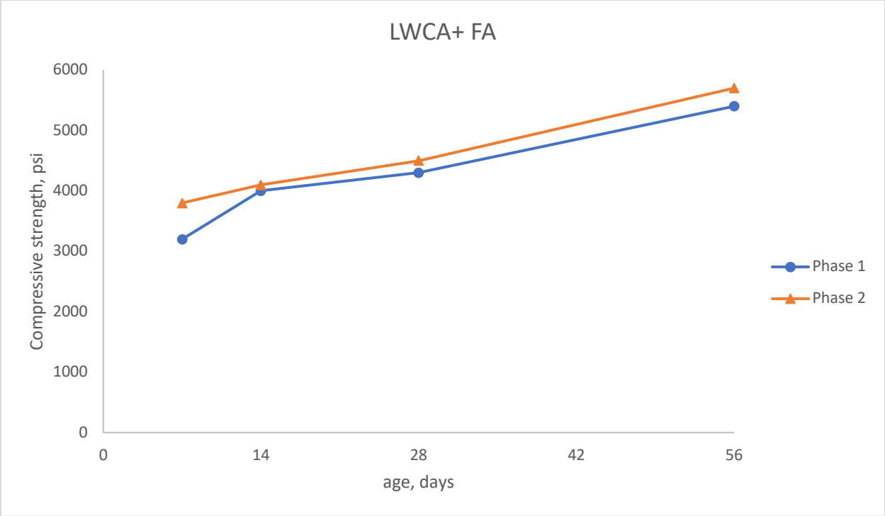
Figure 5-29: Comparison of compressive strength of LWCA+ FA mix in phase I & phase II
