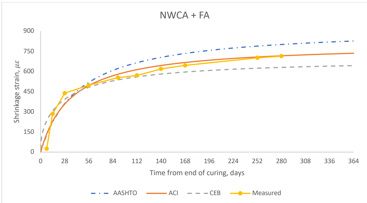
Figure 5-52: Comparison of measured shrinkage with predicted models of NWCA+FA mix
