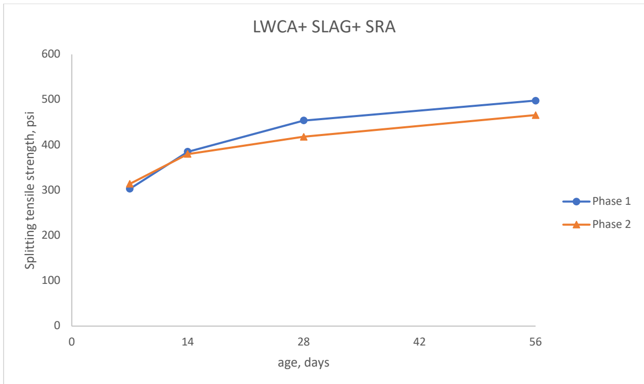
Figure 5-36: Comparison of Splitting tensile strength of LWCA+ slag+ SRA mix in phase I & phase II
