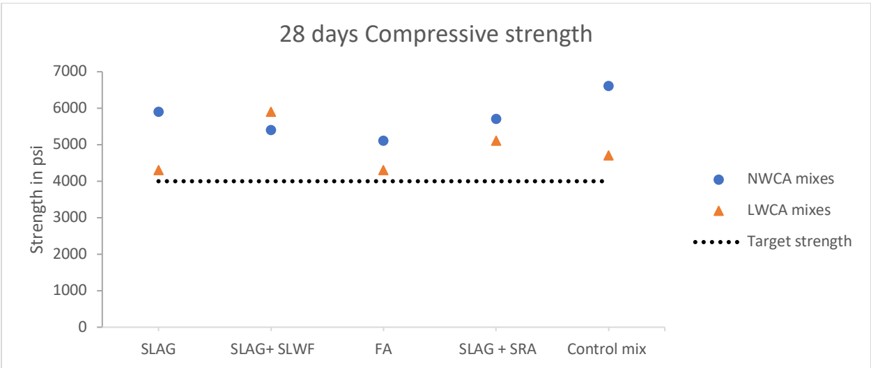
Figure 5-1: Comparison of 28-day compressive strength- Phase I
