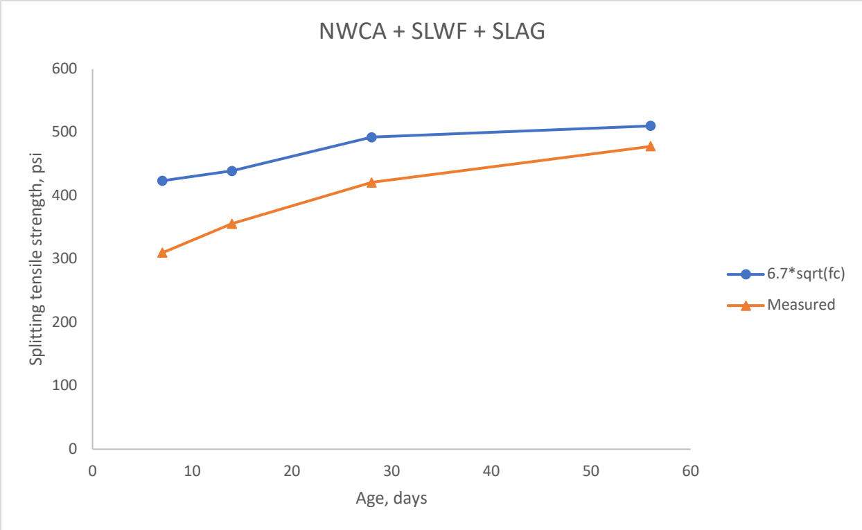
Figure 5-6: Splitting tensile strength NWCA + SLWF + SLAG
