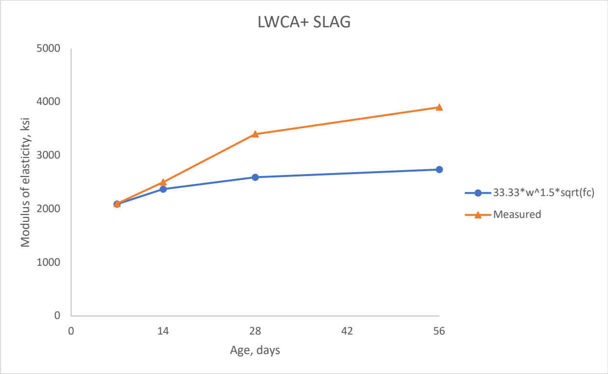
Figure 5-20: Modulus of elasticity, LWCA+ SLAG
