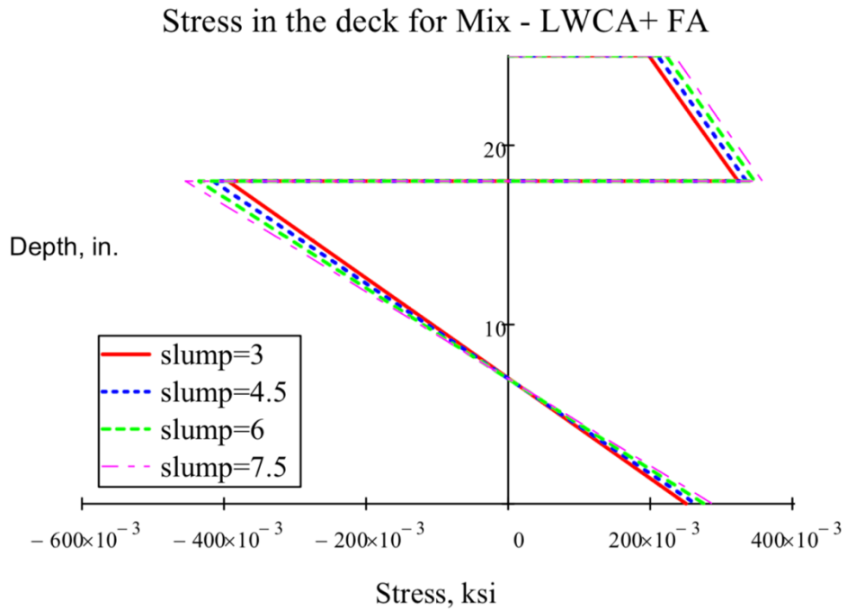
Figure 5-67: Stresses in deck for varying slump of the deck mix – LWCA+FA
