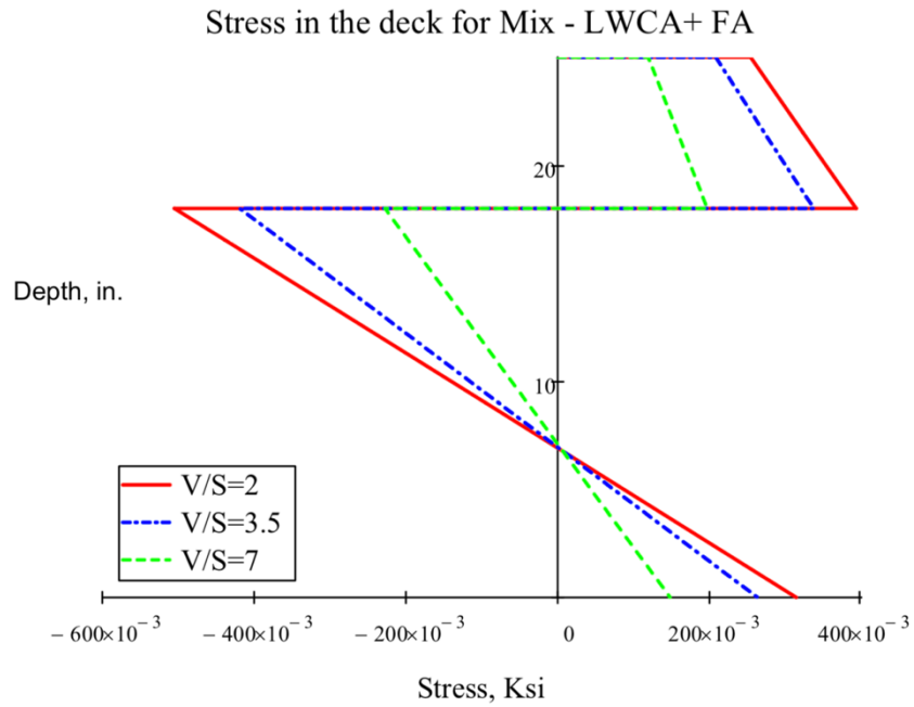
Figure 5-62: Stresses in deck for varying V/S ratio – LWCA+ FA
