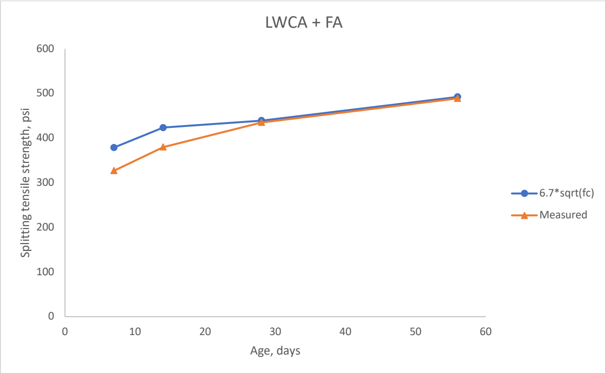
Figure 5-12: Splitting tensile strength LWCA + FA
