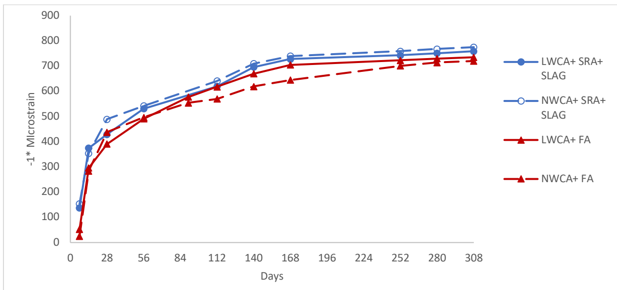
Figure 4-5: Unrestrained shrinkage of mixes in Phase II
