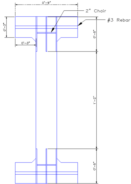
Figure 3-1: Tensile creep specimen, schematic.
