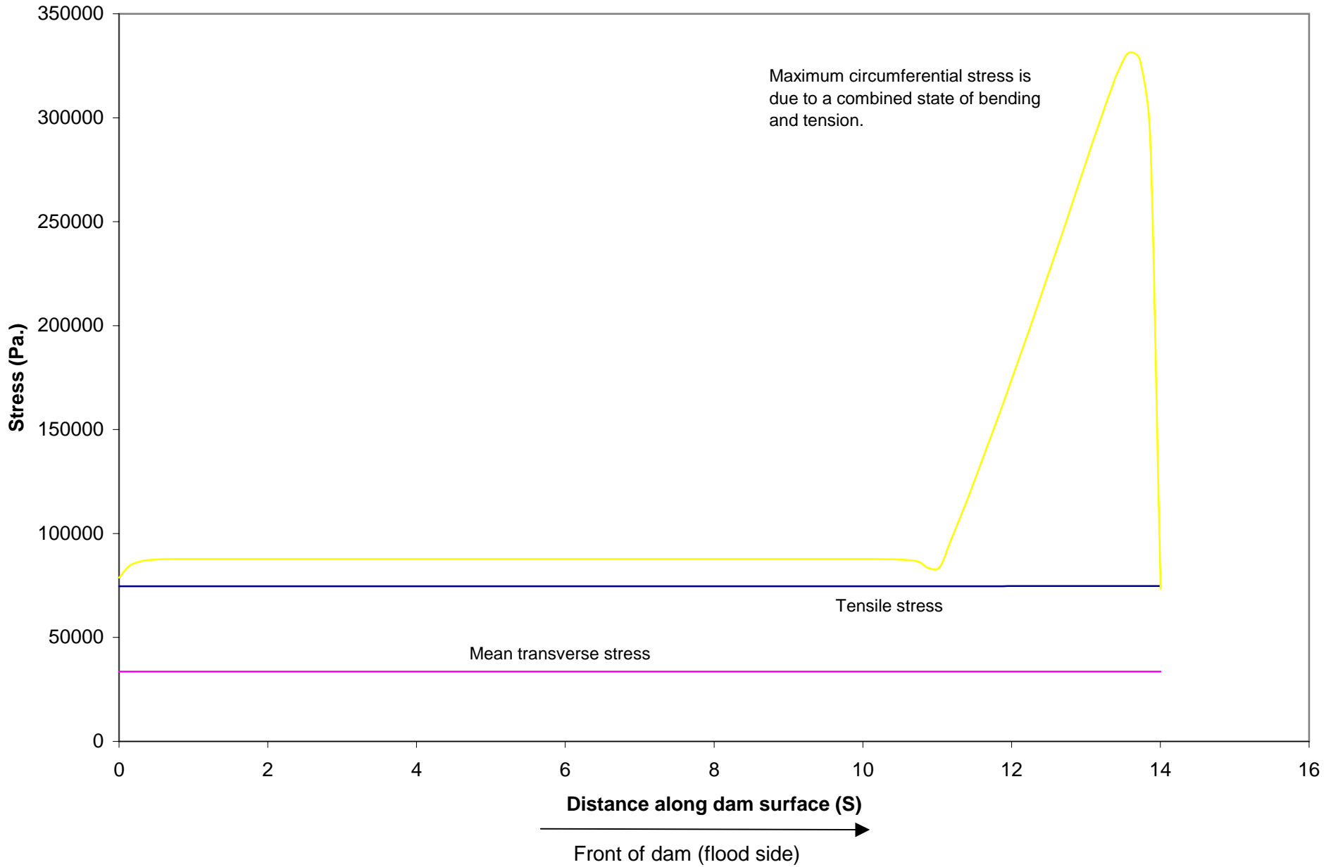
Figure I-11: Plot of the stresses in the dam for a low inflation pressure.
