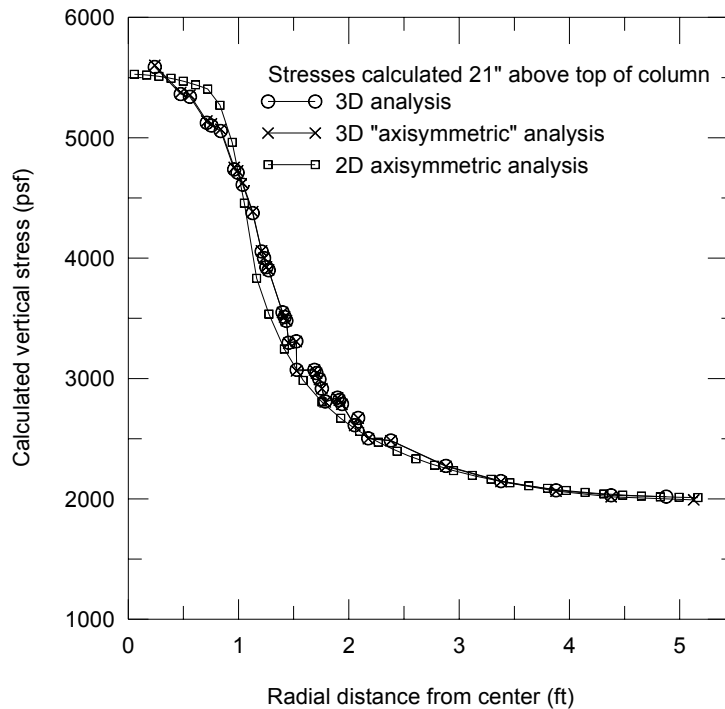
Figure 3. Comparison of two- and three-dimensional numerical analyses of the I-95/Route 1 test embankment at an elevation near the level of the pressure cells.
