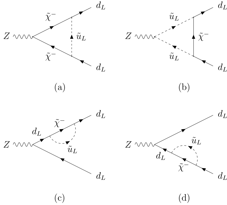
FIG. 3. Examples of leading 1PI R-parity conserving chargino-sfermion contributions subsumed into \delta s^2 . There are analogous diagrams with u_L quark final states and with lepton final states.
