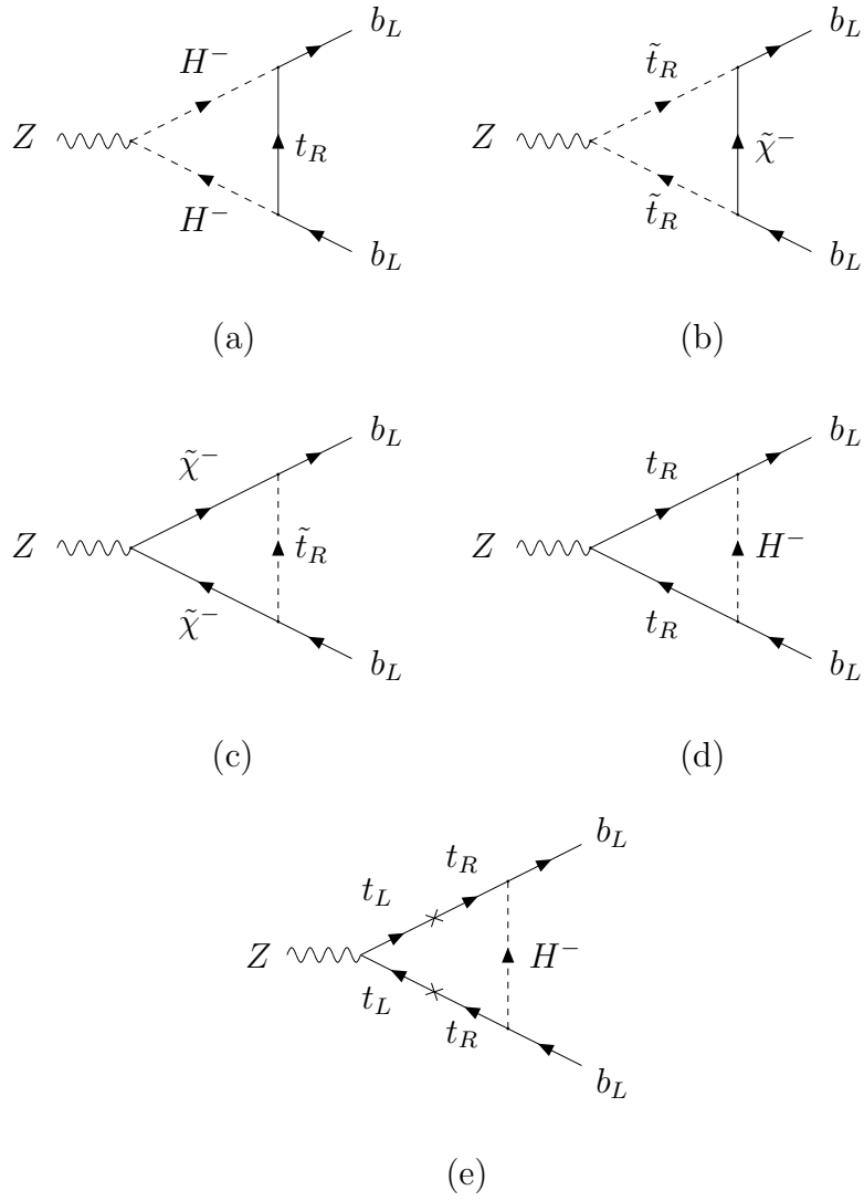
FIG. 4. Leading 1PI R-parity conserving contributions specific to \delta h_{b_L}^{\text{Higgs}} .
