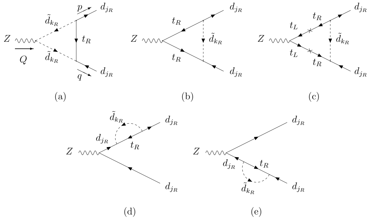
FIG. 2. One-loop corrections to Z \rightarrow d_{jR} \bar{d}_{jR} involving the R-parity violating \lambda'' couplings.
