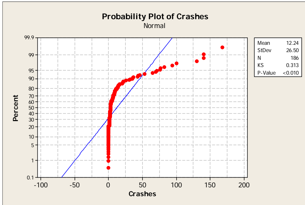
Figure 24. Normality Test
