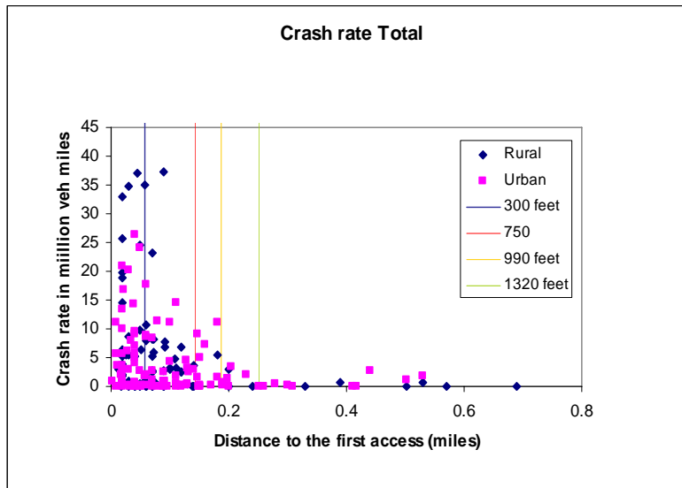
Figure B-1. Crash Rate for the Urban/Rural Category
