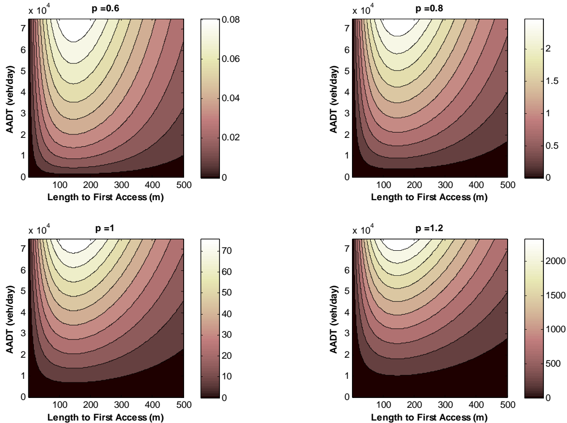
Figure 33. Variation in Expected Crashes as a Function of AADT Exponent
