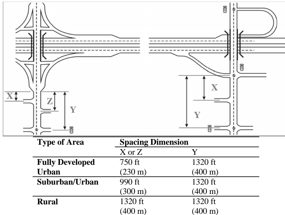
Figure 7. Minimum Spacing for Freeway Interchange Area for Two-Lane Road
