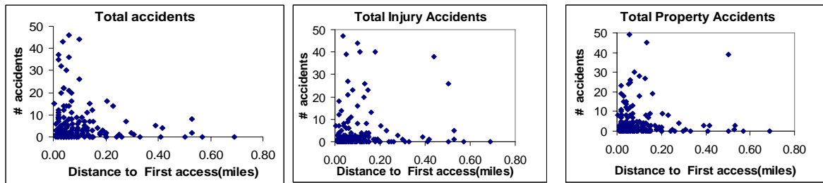
Figure 16. Number of Crashes for different type of Accidents as a Function of the Distance to the First Access
