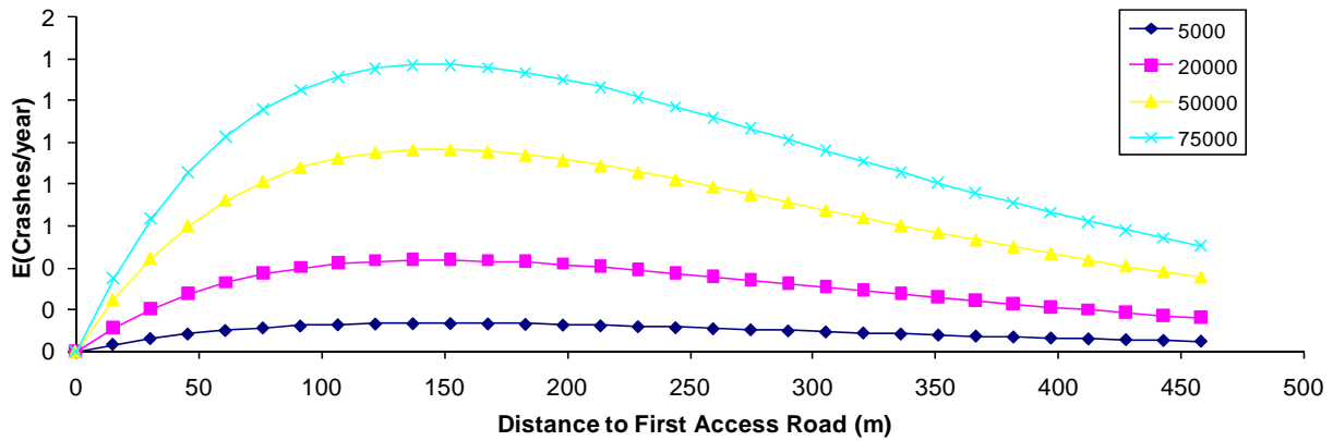
Figure 38. 95% Lower Confidence Limit of the Expected Number of Yearly Crashes As a Function of the Access Section Length and AADT
