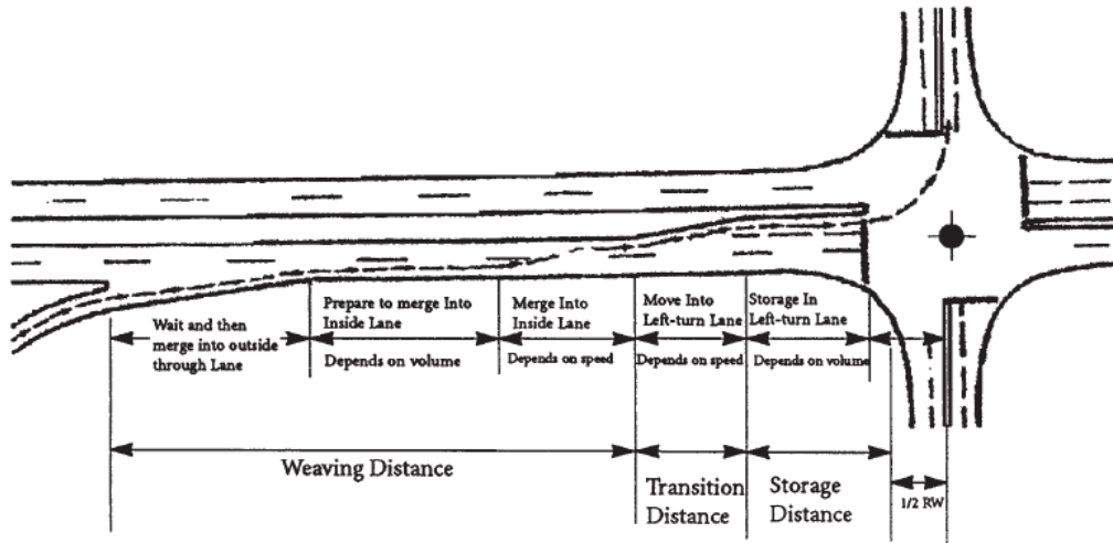
Figure 5. Access Separation Distance
