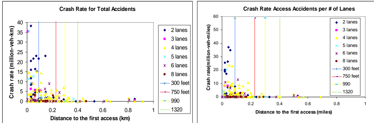
Figure 20. Crash Rate for the Number of Lanes Category
