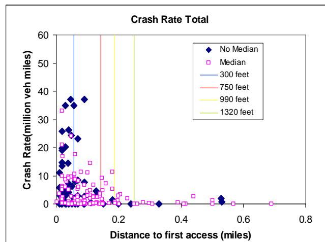
Figure B-2 Crash Rate for the Median/No Median Category
