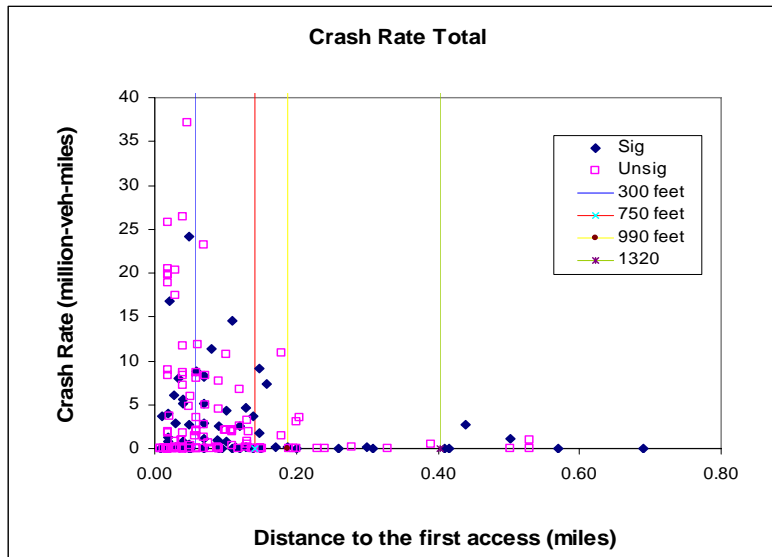
Figure B-6. Crash Rate for the Signalized/Unsignalized Category
