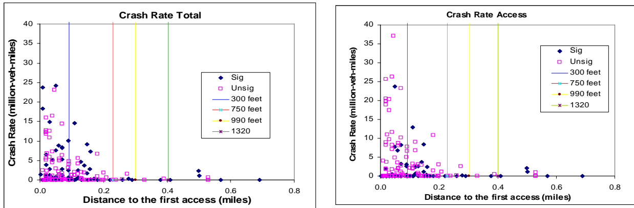
Figure 22. Crash Rate for the Signalized/Unsignalized Category
