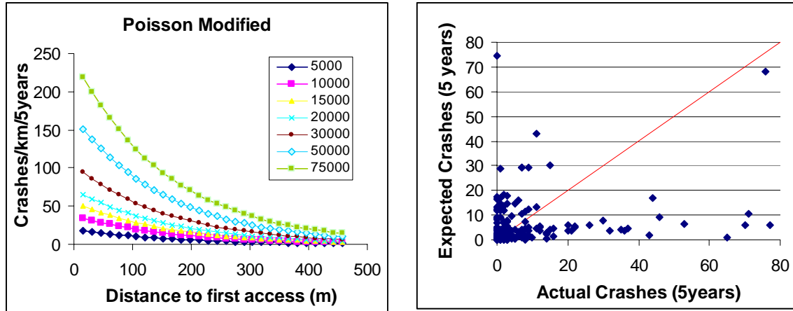
Figure 31. Variation in the Expected Number of Crashes as Function to the Distance to the First Access and Comparison of Actual and Expected Crashes
