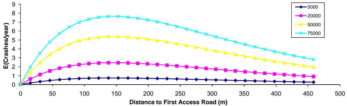
Figure 34: Variation in the Expected Number of Yearly Crashes As a Function of the Access Section Length and AADT
