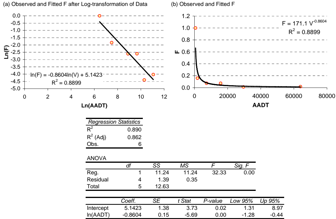
Figure 27. Computation of Exposure Measures
