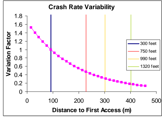
Figure C-5. Variation in the Expected Number of Crashes as a Function to the Distance to the First Access and Comparison of Actual and Expected Crashes
