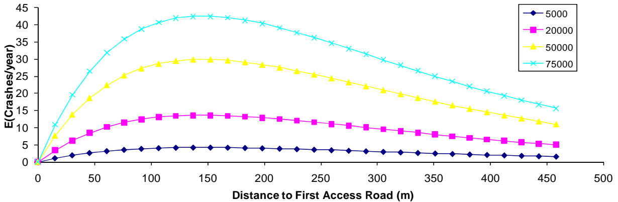
Figure 37. 95% Upper Confidence Limit of the Expected Number of Yearly Crashes As a Function of the Access Section Length and AADT
