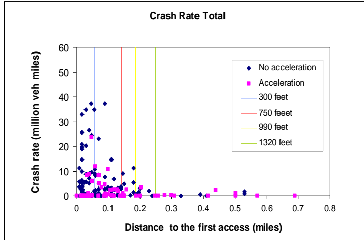
Figure B-7. Crash Rate as a Function of the Presence of Acceleration Lane
