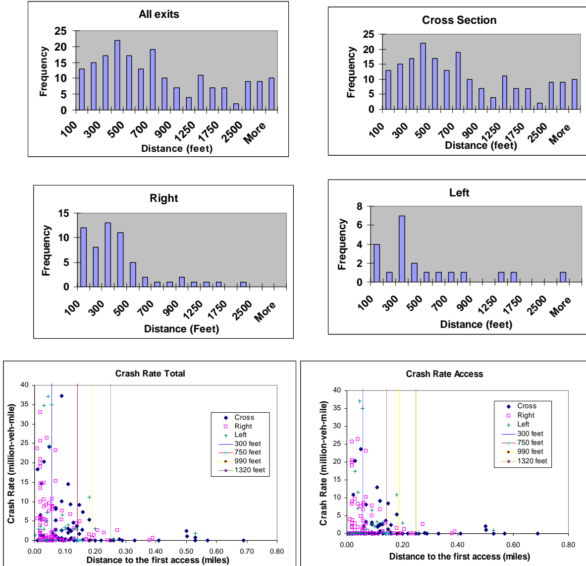
Figure 19. Distribution of Distances and Crash Rate for the Type of Access Category
