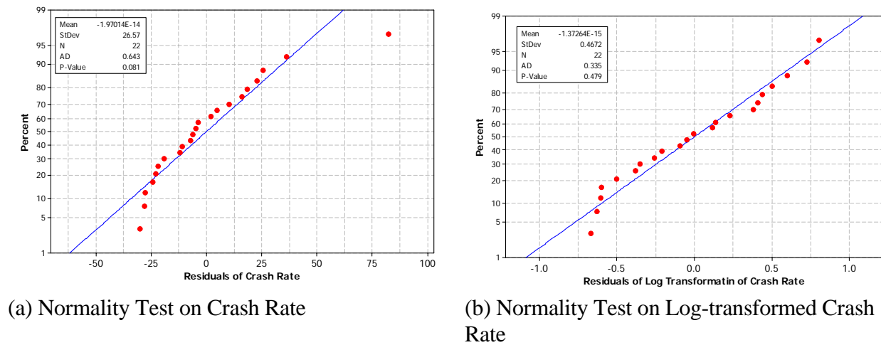
Figure 28. Test of Normality for Crash Rate Data
