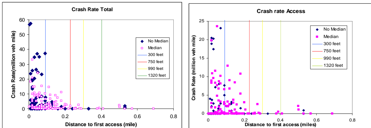
Figure 18. Crash Rate as a Function of the Presence of a Median
