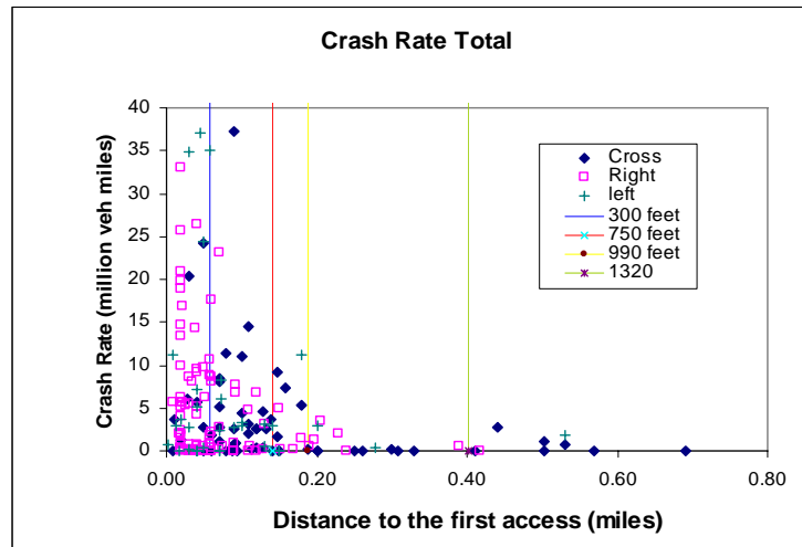
Figure B-3. Distribution of Distances and Crash Rate for the Type of Access Category
