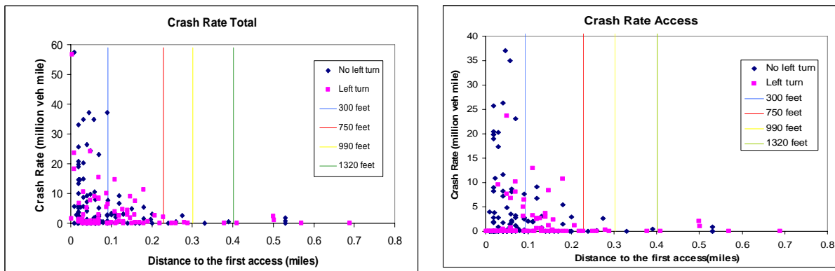
Figure 21. Crash Rate as a Function of the Presence of a Left Turn Storage Lane
