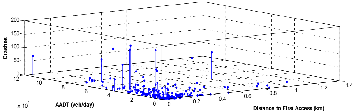
Figure 15. Number of Crashes as a Function of AADT and Distance to the First Access
