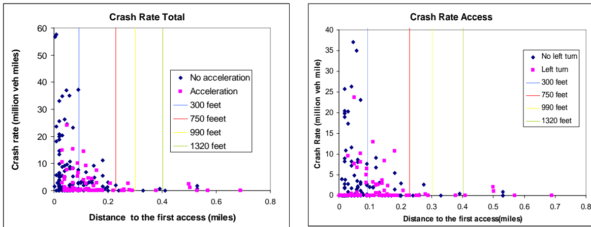
Figure 23. Crash Rate As a Function of the Presence of Acceleration Lane
