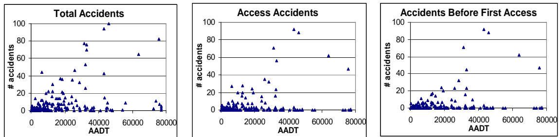
Figure 14. Number of Accidents versus AADT
