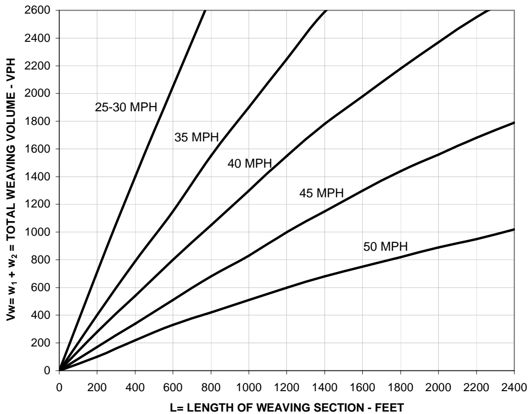
Figure 2. Analysis of Service Road Weaving Conditions (Layton, 1996)
