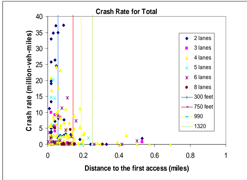
Figure B-4. Crash Rate for the Number of Lanes Category
