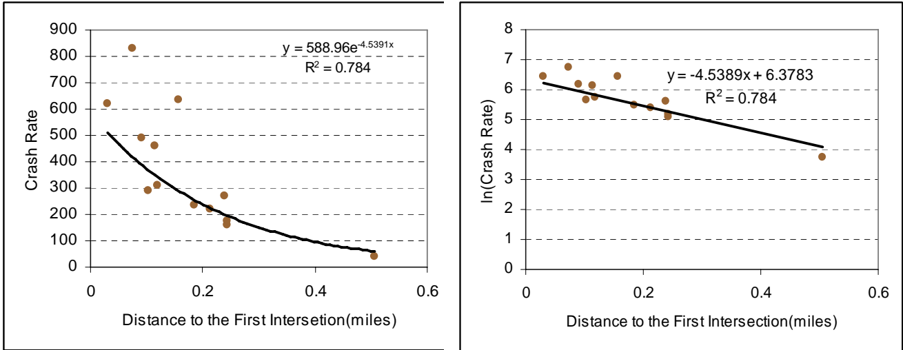
Figure C-4. Crash Prediction Model Considering Nearest Intersection
