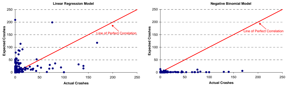
Figure 39. Comparison of Actual and Expected Crashes (All 186 Sites)
