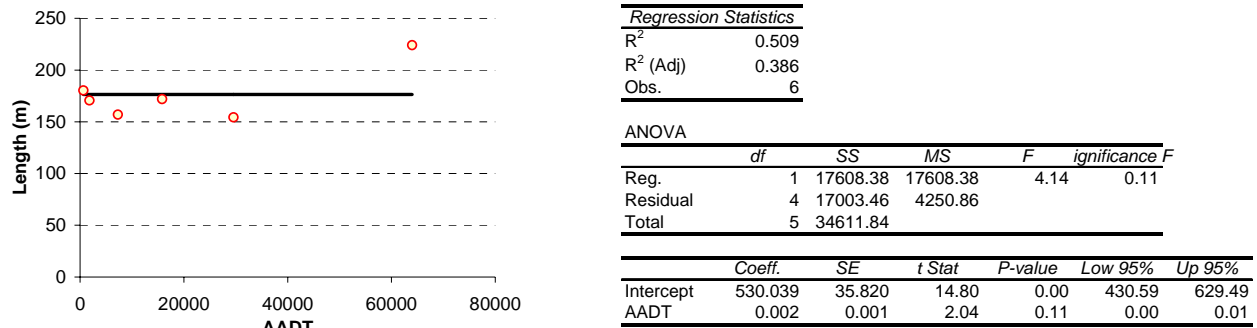
Figure 25. Effect of Access Section Length within AADT Binning
