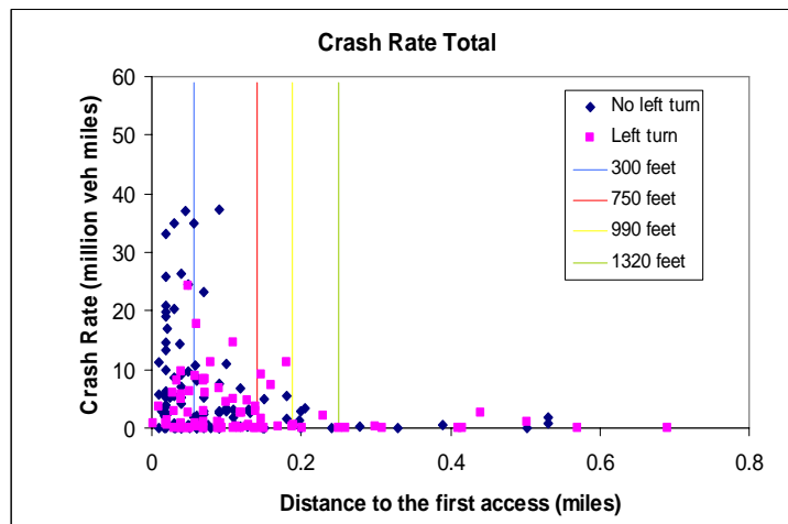
Figure B-5. Crash Rate as a Function of the Presence of a Left Turn Storage Lane
