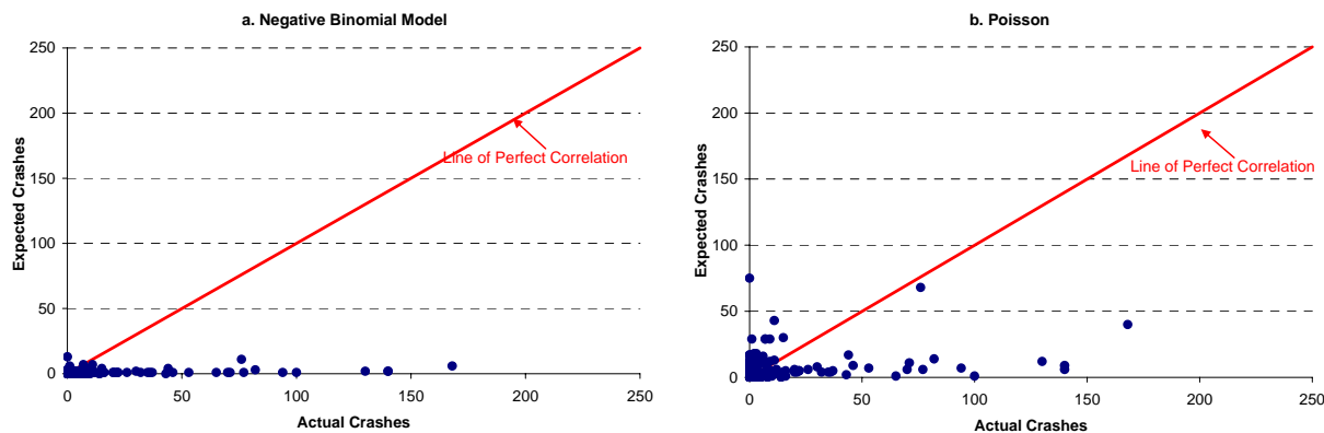
Figure 32. Comparison of Negative Binomial and Poisson Model Estimates
