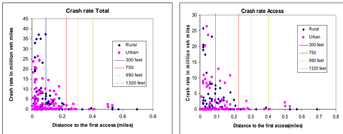
Figure 17. Crash Rate for the Urban/Rural Category
