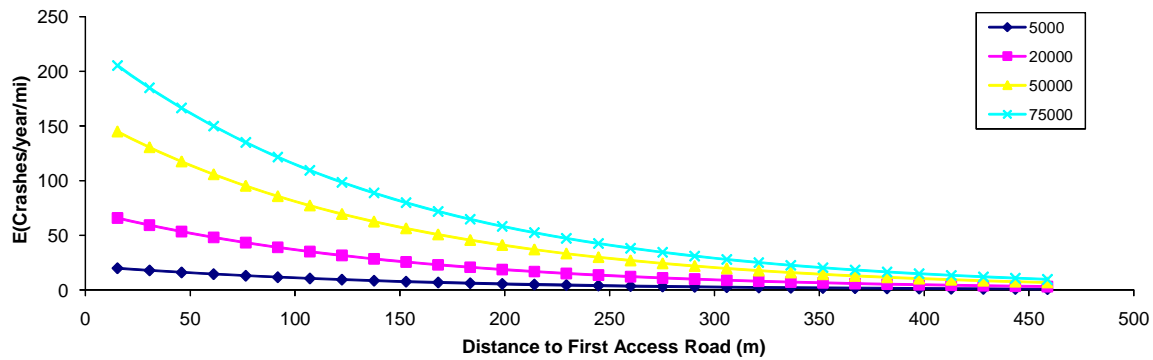
Figure 36. Variation in the Expected Number of Yearly Crashes per Mile As a Function of the Access Section Length and AADT
