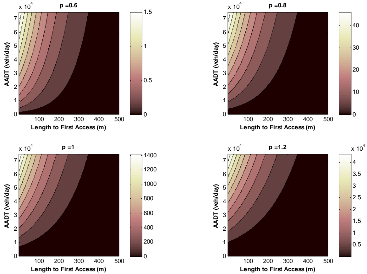
Figure 35. Variation in Expected Crashes/Km As a Function of AADT Exponent
