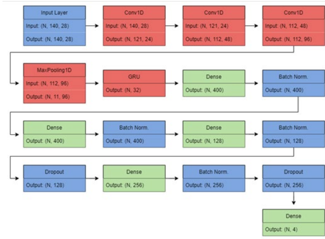
Figure 6. Diagram. Neural network diagram – glance only model.
