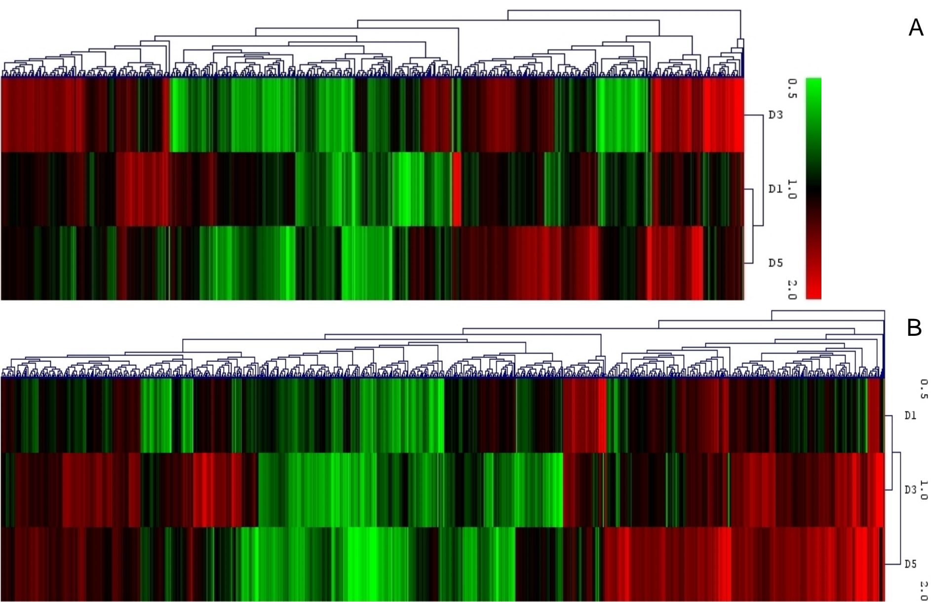
Additional file 2 – Hierarchical cluster of 722 selected genes from NAA-treated FAZ (A) and 1057 selected genes from shading-treated FAZ (B) from the 40 K apple microarray. The fold changes in gene expression are scaled from 0.5 to 2.0 to allow clustering by expression pattern, with intense red representing maximum expression and intense green representing minimum expression.
